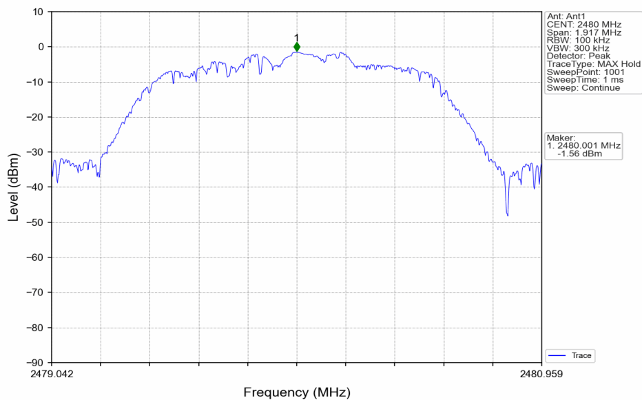
Pi/4DQPSK_2DH5_HCH_2480MHz_Ant1_NTNV
