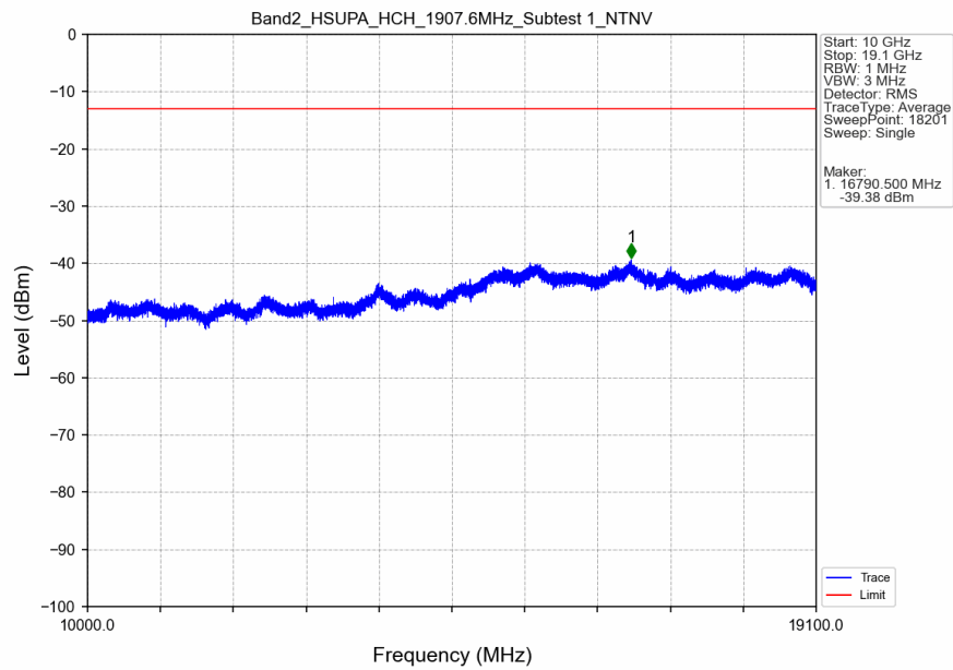
Band2_HSUPA_HCH_1907.6MHz_Subtest 1_NTNV
