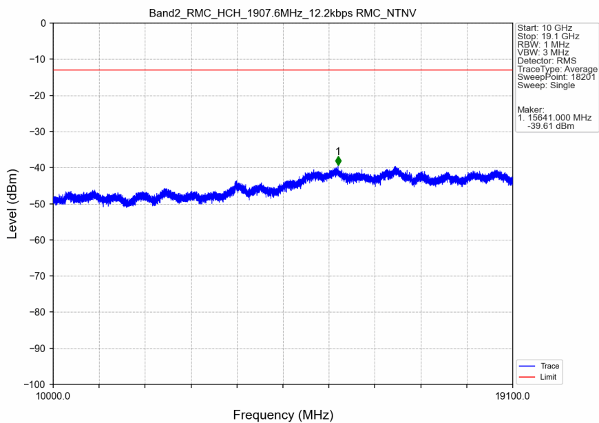
Band2_RMC_HCH_1907.6MHz_12.2kbps RMC_NTNV
