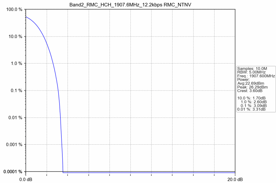
Band2_RMC_HCH_1907.6MHz_12.2kbps RMC_NTNV
