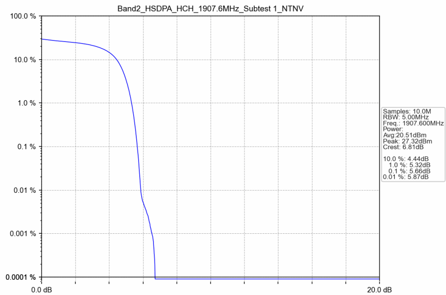
Band2_HSDPA_HCH_1907.6MHz_Subtest 1_NTNV
