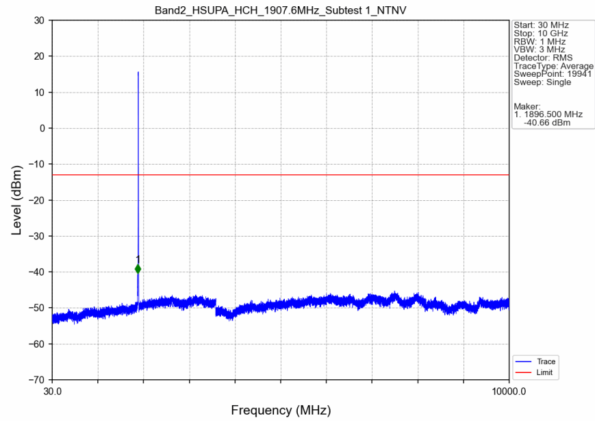
Band2_HSUPA_HCH_1907.6MHz_Subtest 1_NTNV
