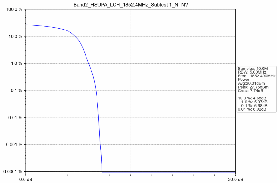
Band2_HSUPA_LCH_1852.4MHz_Subtest 1_NTNV
