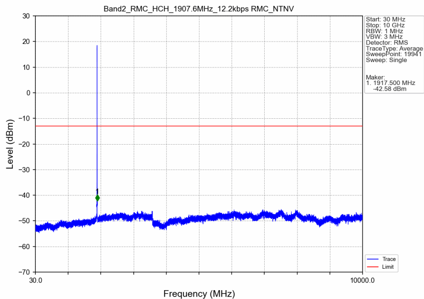
Band2_RMC_HCH_1907.6MHz_12.2kbps RMC_NTNV
