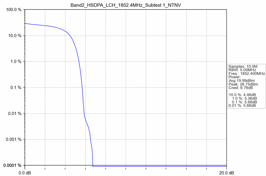
Band2_HSDPA_LCH_1852.4MHz_Subtest 1_NTNV
