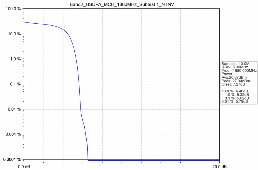
Band2_HSDPA_MCH_1880MHz_Subtest 1_NTNV
