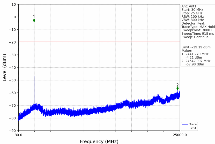
Pi/4DQPSK_2DH5_MCH_2441MHz_Ant1_NTNV
