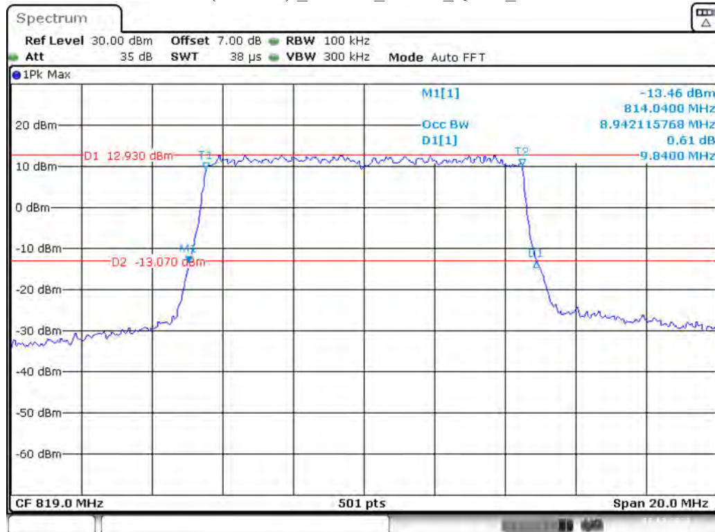
Band 26(Part 90S) _10 MHz_Middle_QPSK_RB50#0
