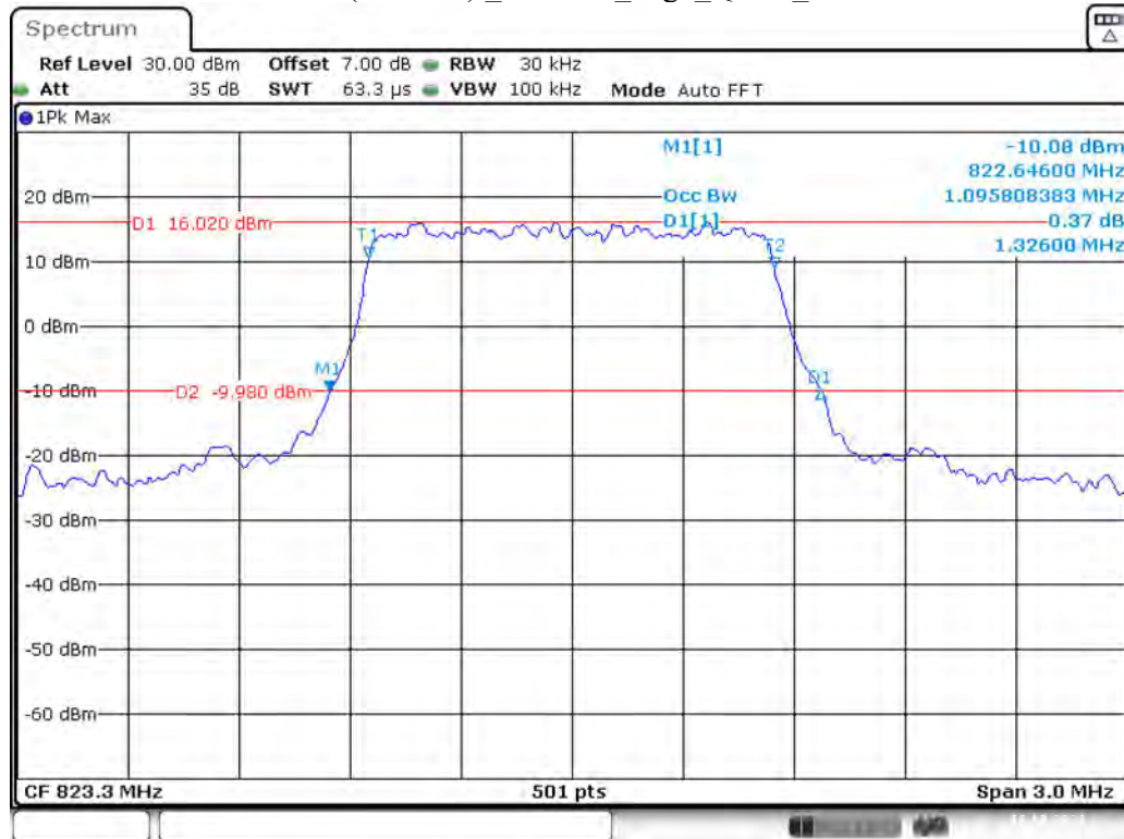
Band 26(Part 90S)_1.4 MHz_High_QPSK_RB6#0
