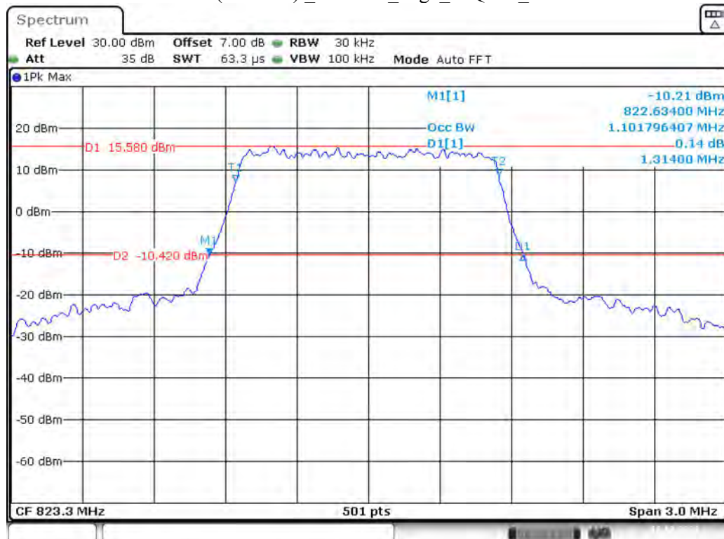
Band 26(Part 90S)_1.4 MHz_High_16QAM_RB6#0
