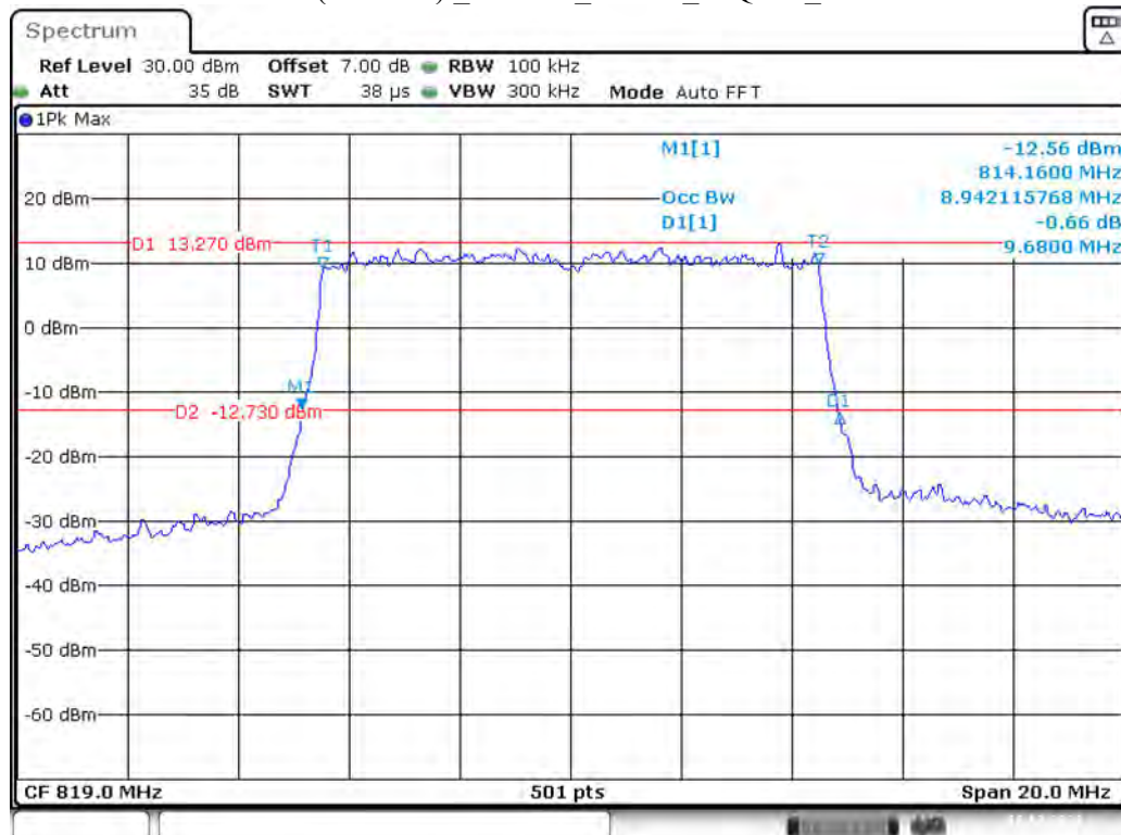
Band 26(Part 90S) _10 MHz_Middle_16QAM_RB50#0
