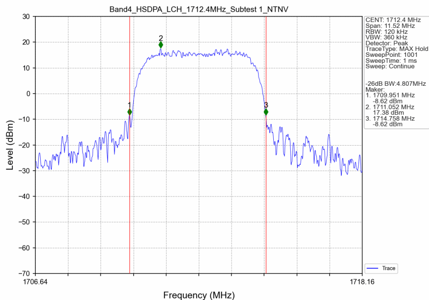
Band4_HSDPA_LCH_1712.4MHz_Subtest 1_NTNV
