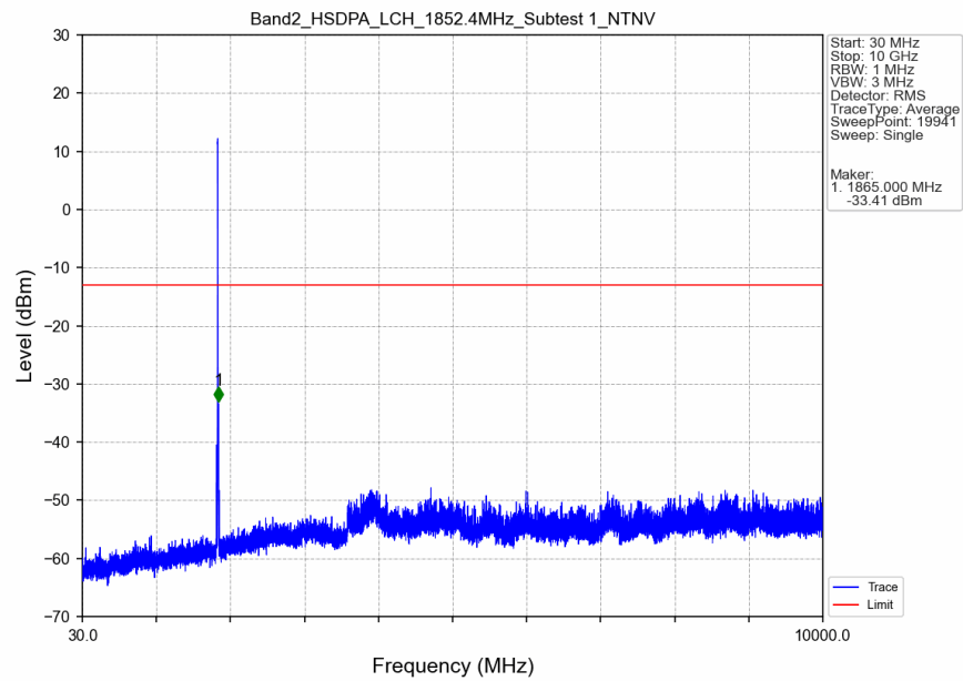
Band2_HSDPA_LCH_1852.4MHz_Subtest 1_NTNV
