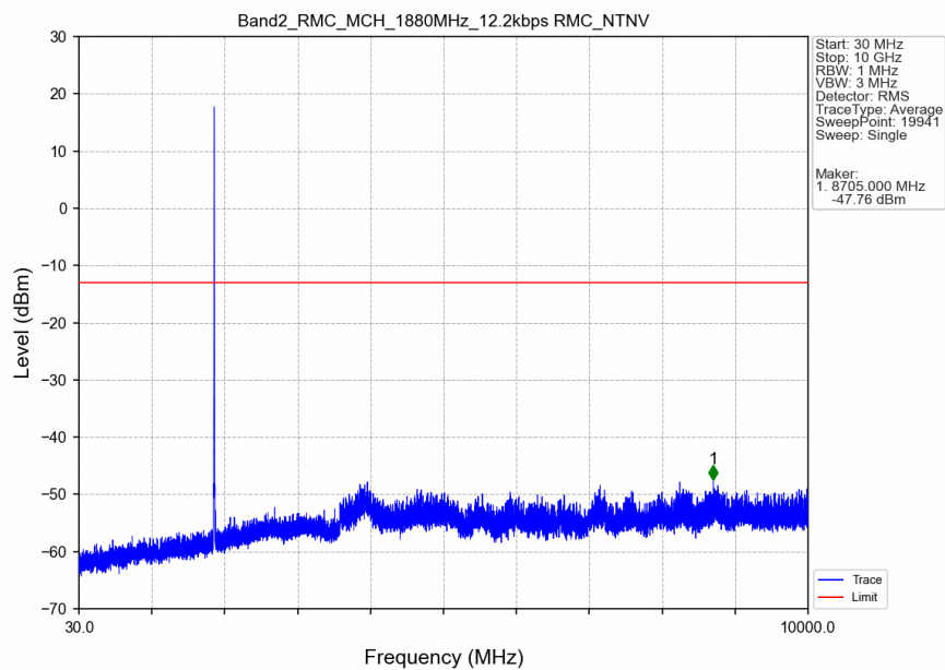
Band2_RMC_MCH_1880MHz_12.2kbps RMC_NTNV
