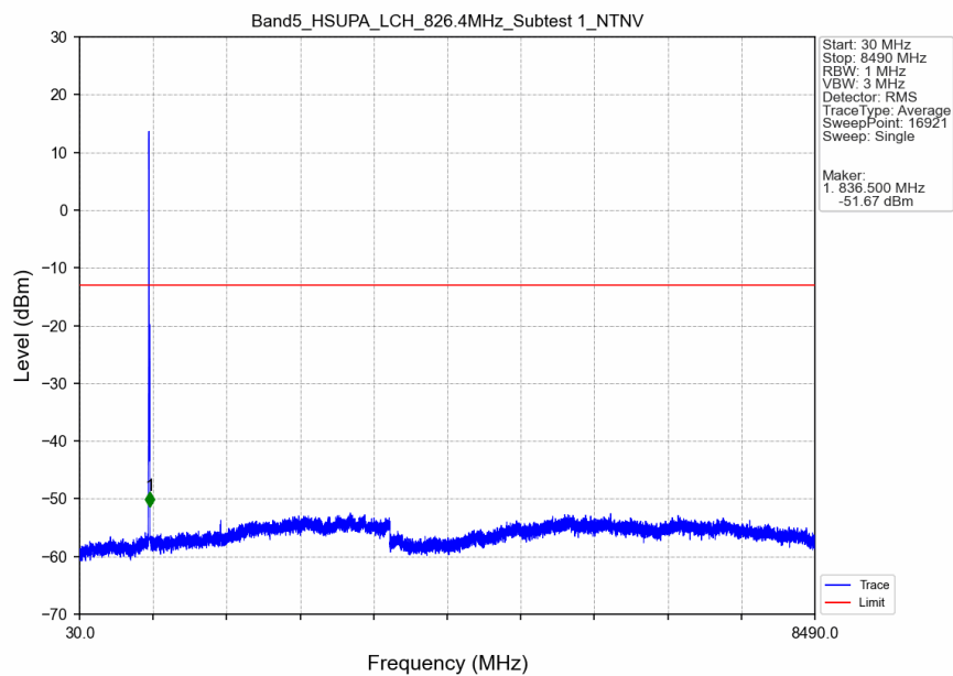
Band5_HSUPA_LCH_826.4MHz_Subtest 1_NTNV
