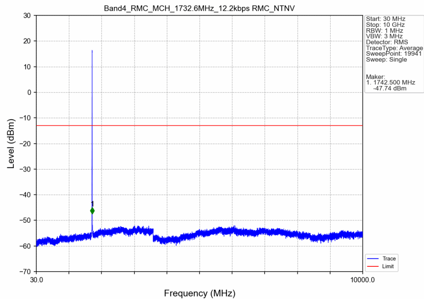
Band4_RMC_MCH_1732.6MHz_12.2kbps RMC_NTNV
