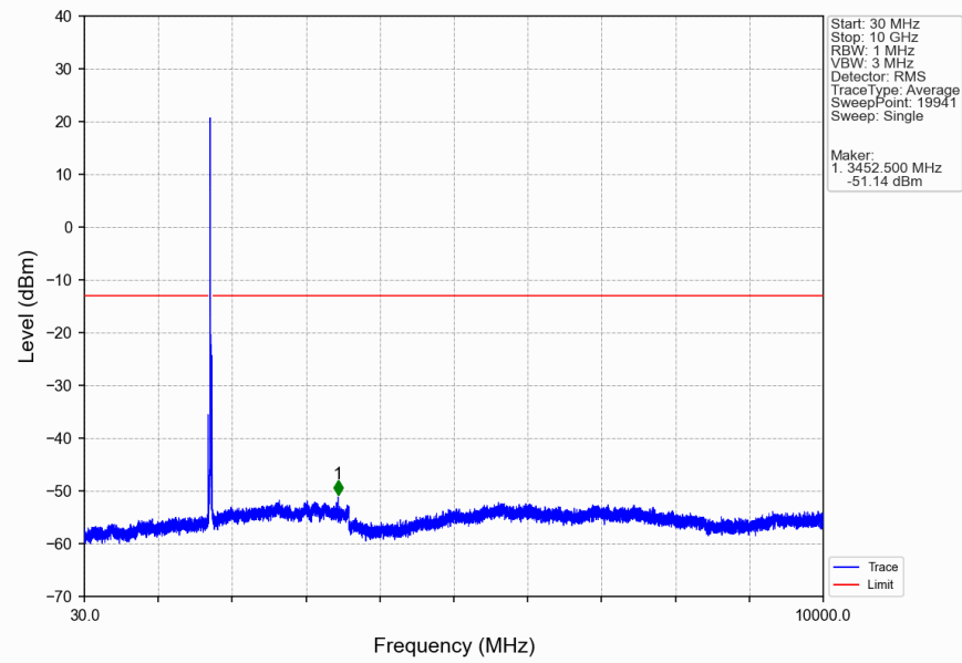
Band4_15MHz_QPSK_MCH_1732.5MHz_RB_1_0_NTNV
