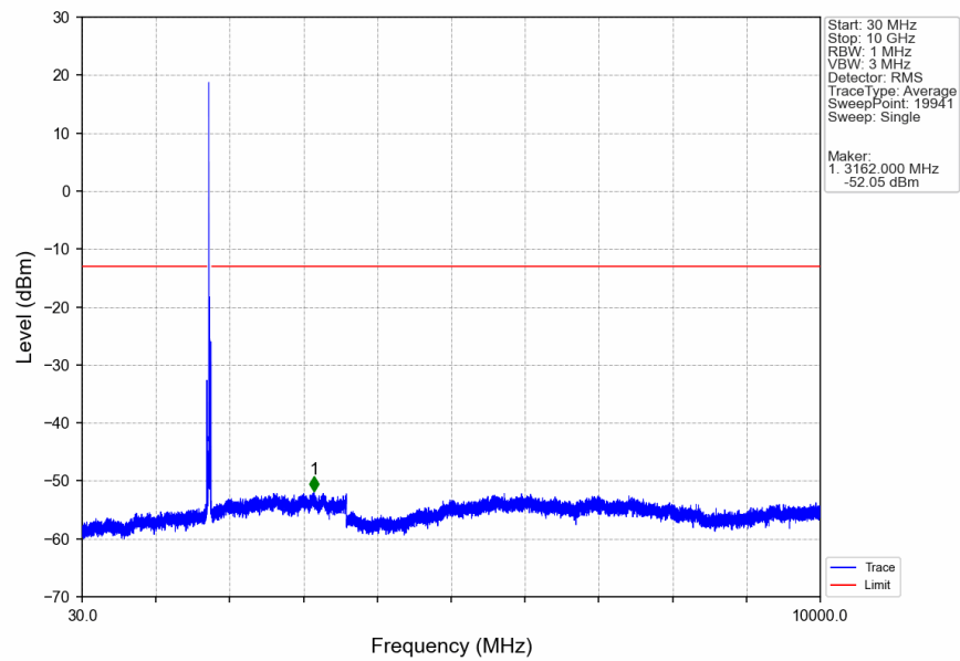
Band4_15MHz_QPSK_HCH_1747.5MHz_RB_1_0_NTNV
