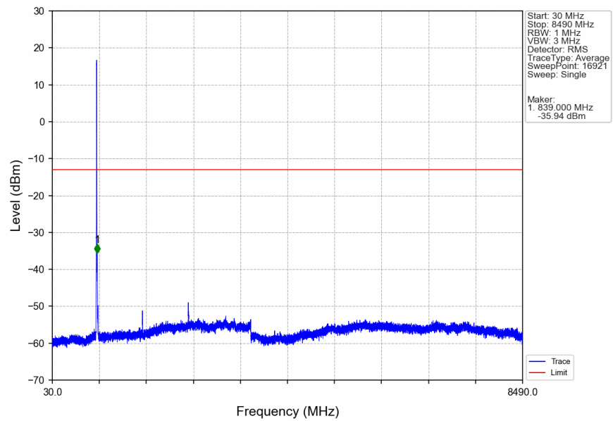
Band5_HSUPA_LCH_826.4MHz_Subtest 1_NTNV
