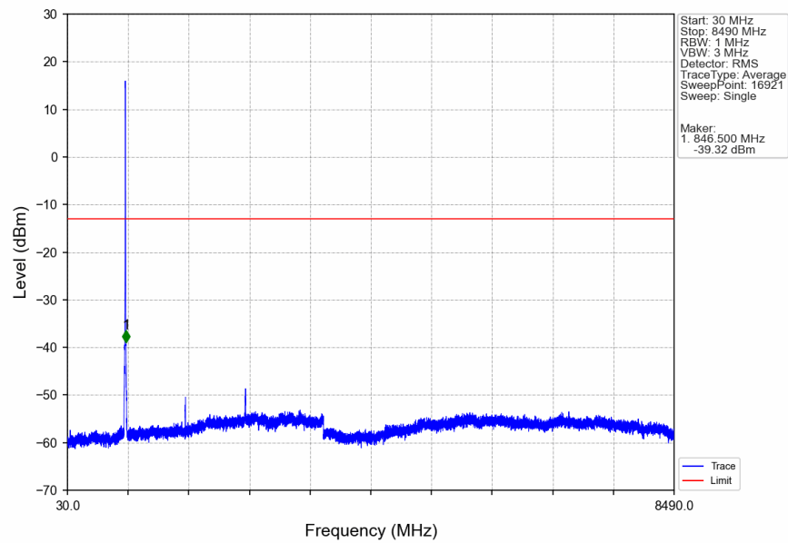
Band5_HSDPA_MCH_836.6MHz_Subtest 1_NTNV
