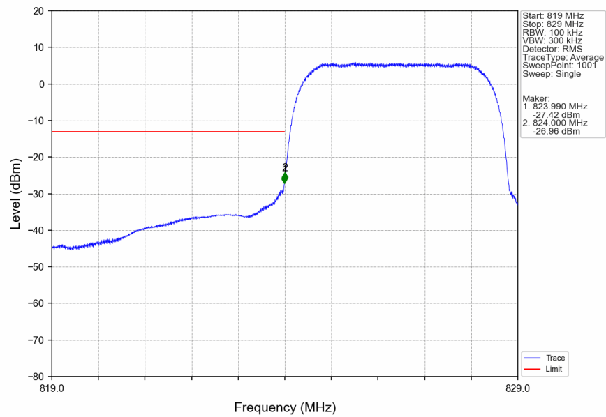
Band5_HSDPA_LCH_826.4MHz_Subtest 1_NTNV
