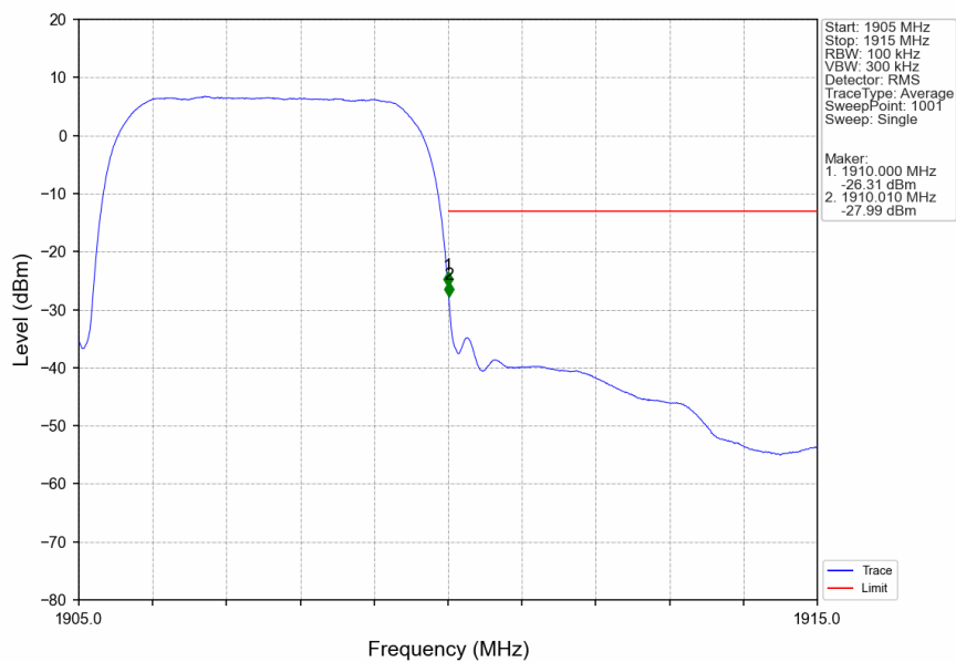
Band2_RMC_HCH_1907.6MHz_12.2kbps RMC_NTNV
