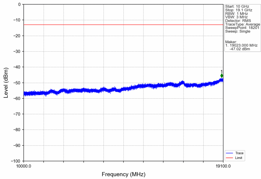
Band2_RMC_MCH_1880MHz_12.2kbps RMC_NTNV
