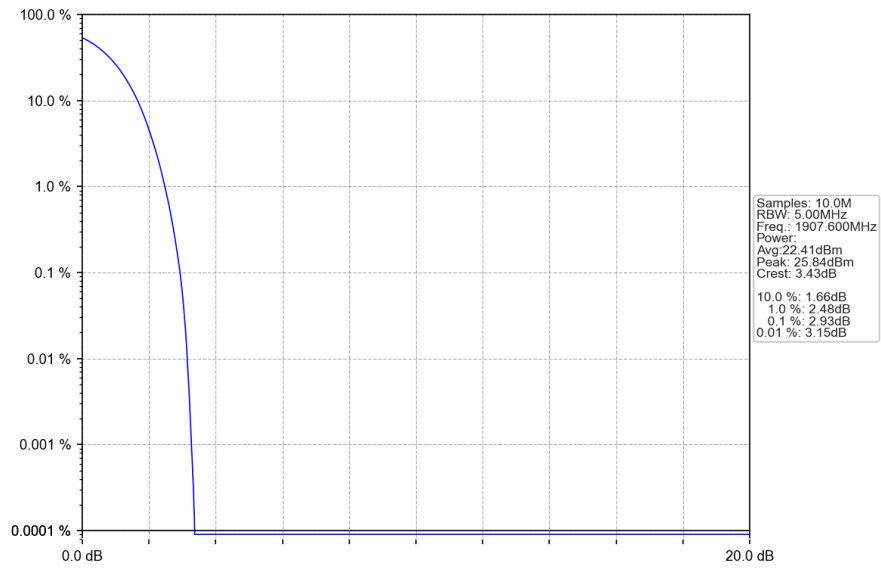
Band2_RMC_HCH_1907.6MHz_12.2kbps RMC_NTNV
