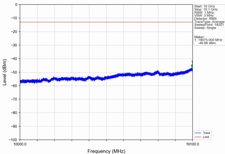
Band2_RMC_HCH_1907.6MHz_12.2kbps RMC_NTNV
