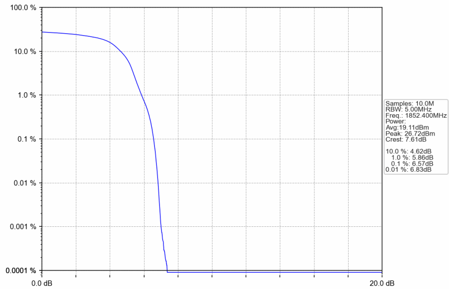
Band2_HSUPA_LCH_1852.4MHz_Subtest 1_NTNV
