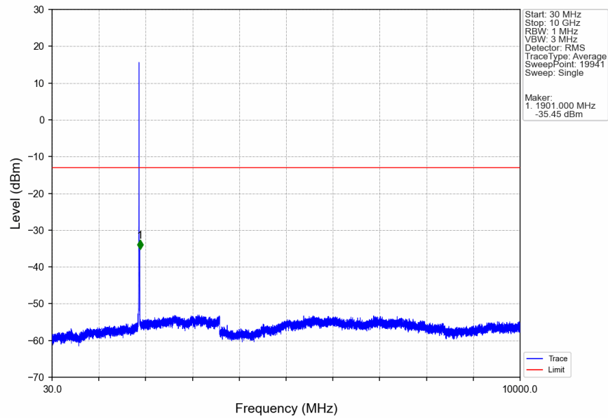
Band2_HSDPA_MCH_1880MHz_Subtest 1_NTNV
