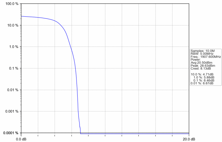
Band2_HSUPA_HCH_1907.6MHz_Subtest 1_NTNV
