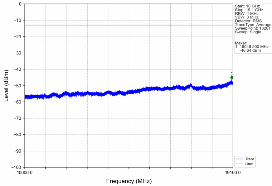
Band2_HSDPA_MCH_1880MHz_Subtest 1_NTNV
