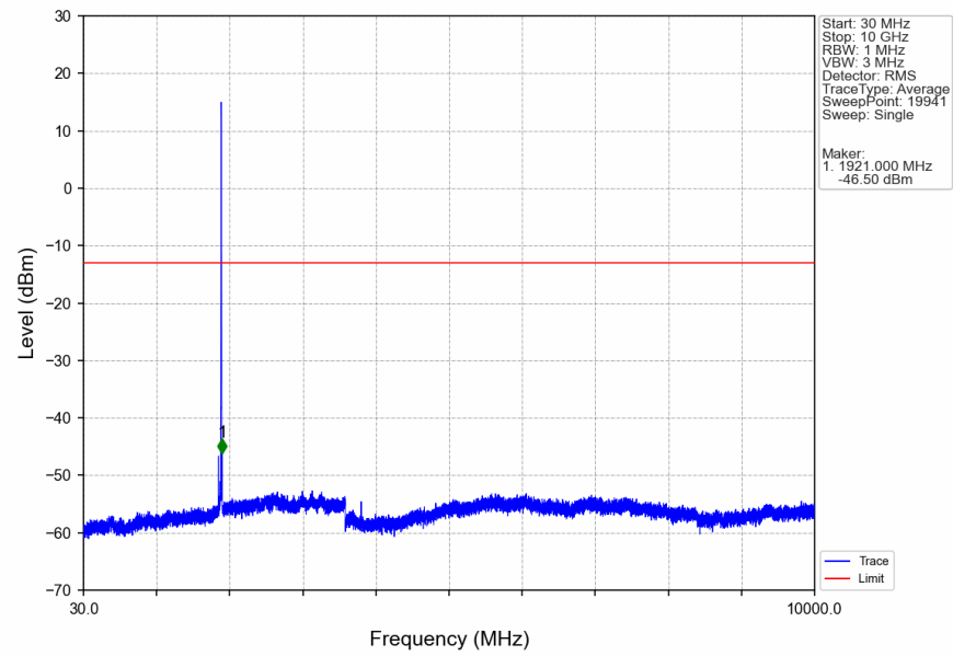
Band2_HSUPA_HCH_1907.6MHz_Subtest 1_NTNV
