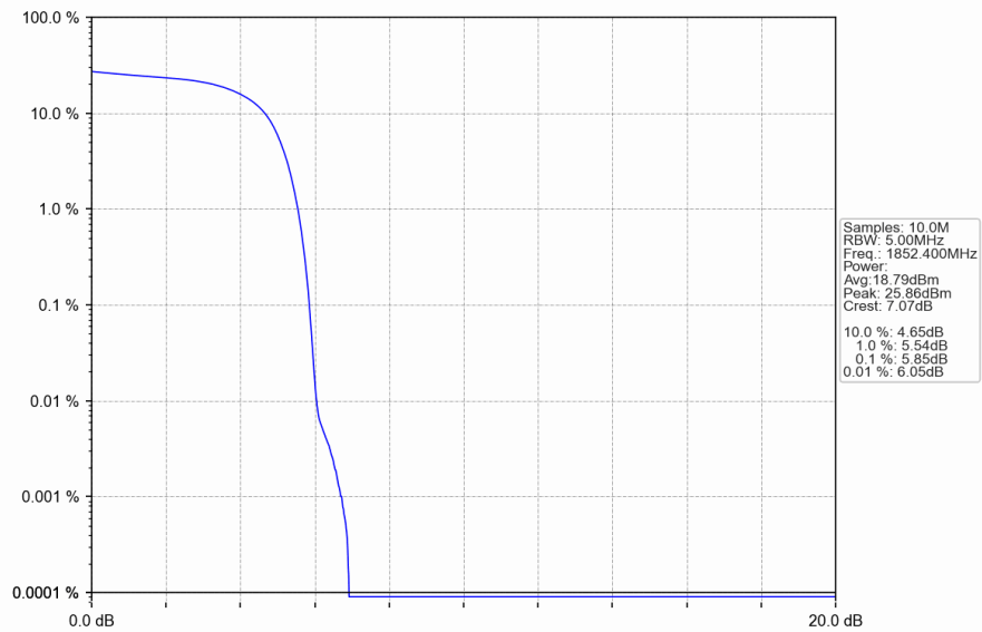
Band2_HSDPA_LCH_1852.4MHz_Subtest 1_NTNV
