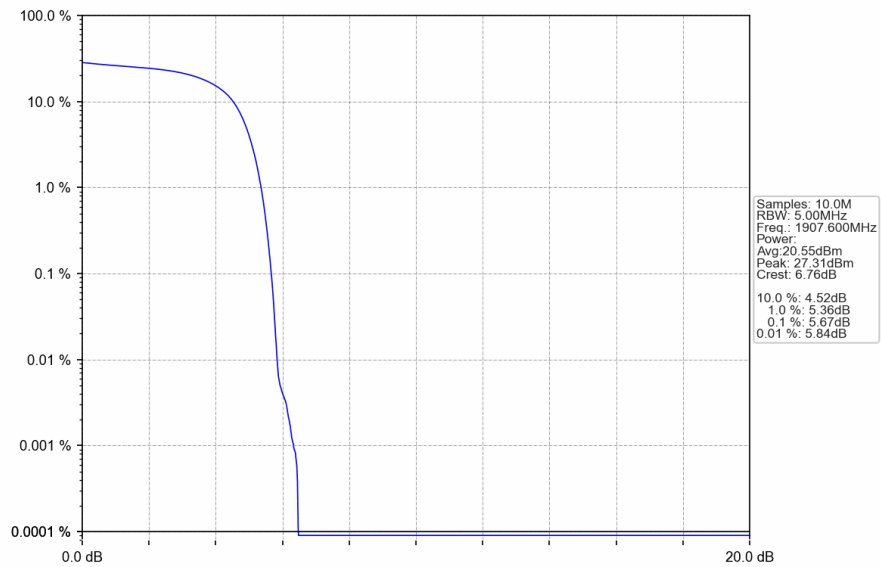
Band2_HSDPA_HCH_1907.6MHz_Subtest 1_NTNV
