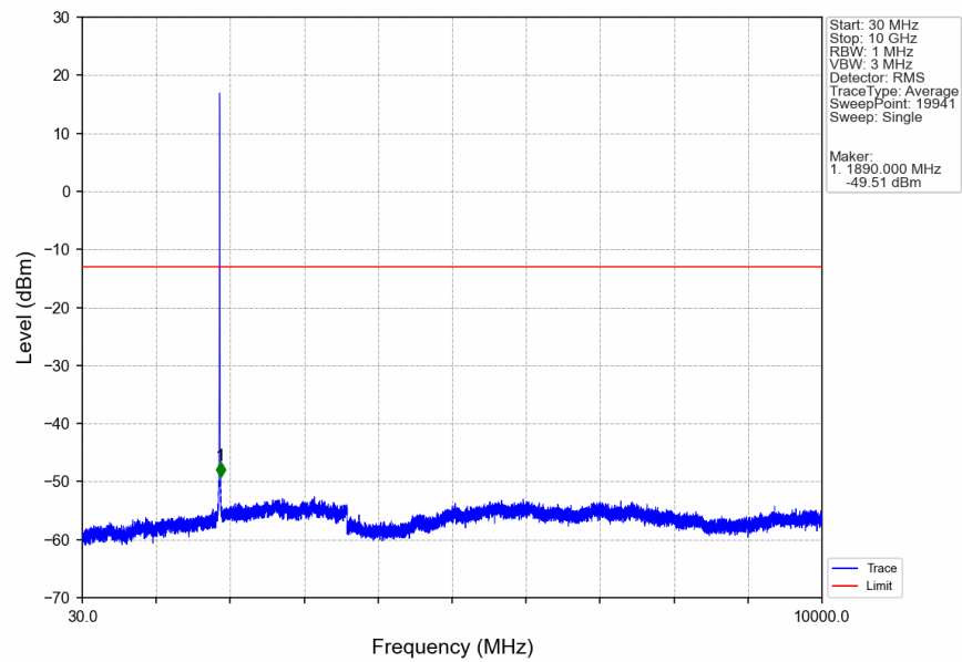
Band2_RMC_MCH_1880MHz_12.2kbps RMC_NTNV
