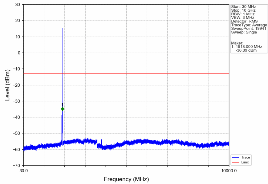
Band2_HSDPA_HCH_1907.6MHz_Subtest 1_NTNV
