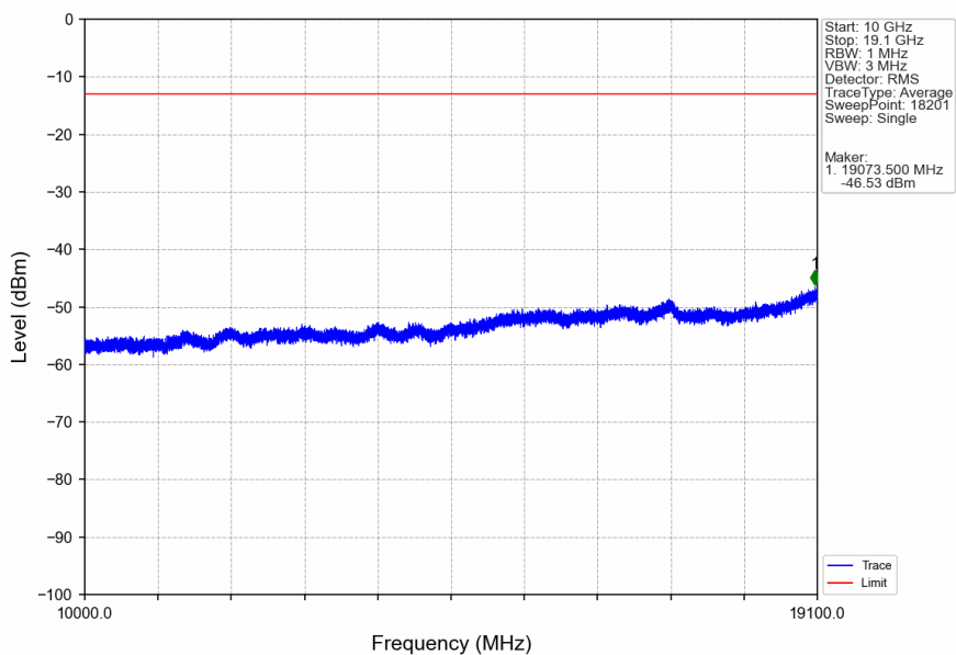
Band2_HSUPA_HCH_1907.6MHz_Subtest 1_NTNV
