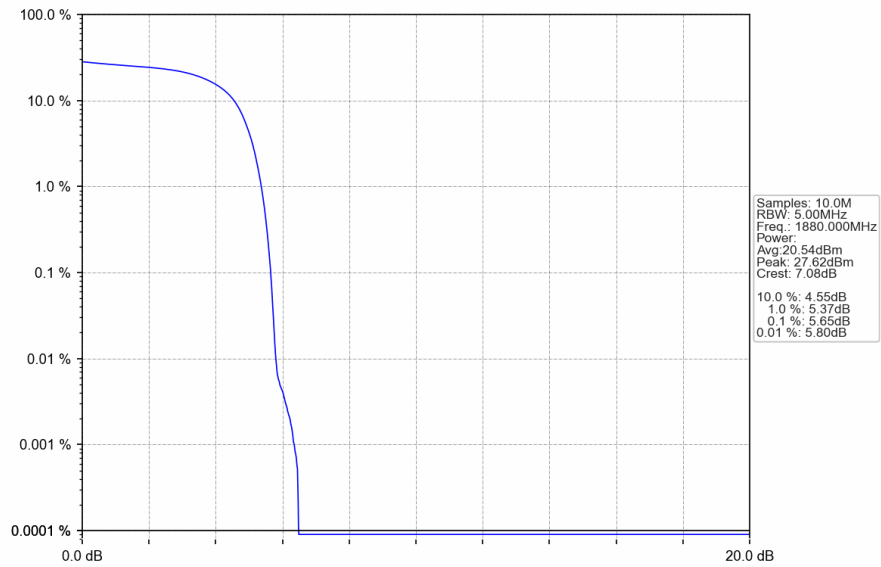
Band2_HSDPA_MCH_1880MHz_Subtest 1_NTNV
