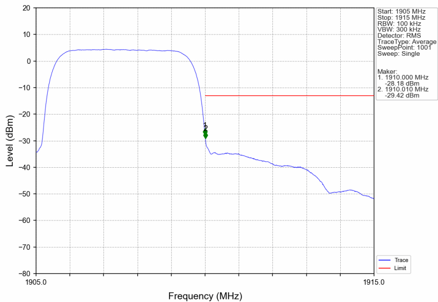
Band2_HSUPA_HCH_1907.6MHz_Subtest 1_NTNV
