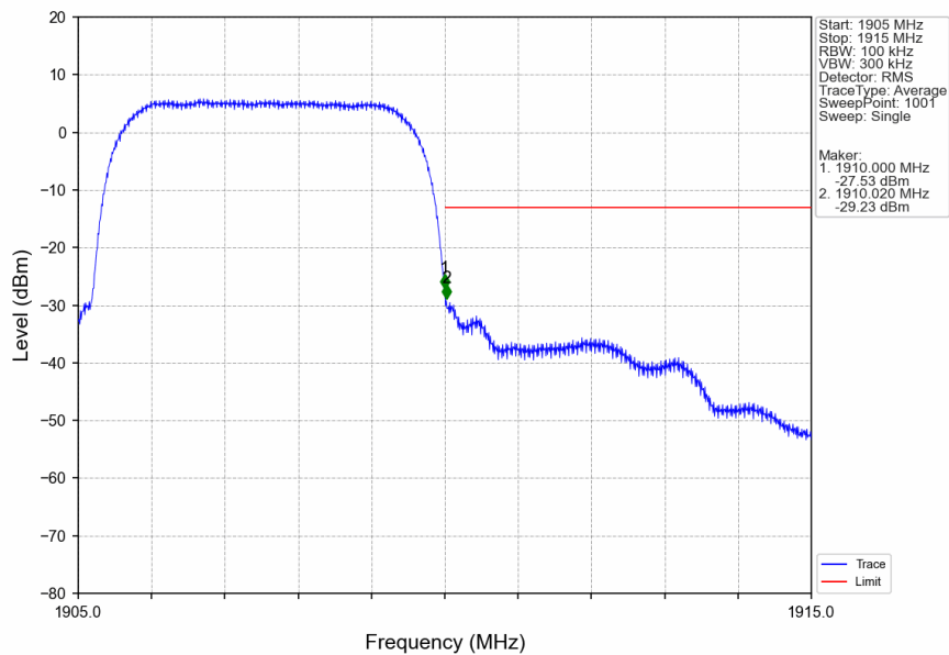
Band2_HSDPA_HCH_1907.6MHz_Subtest 1_NTNV
