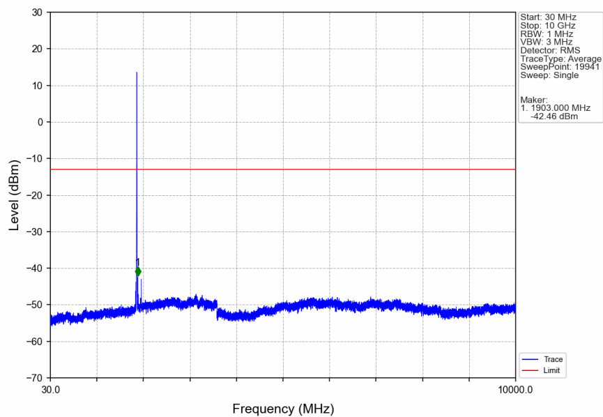
Band2_HSDPA_MCH_1880MHz_Subtest 1_NTNV
