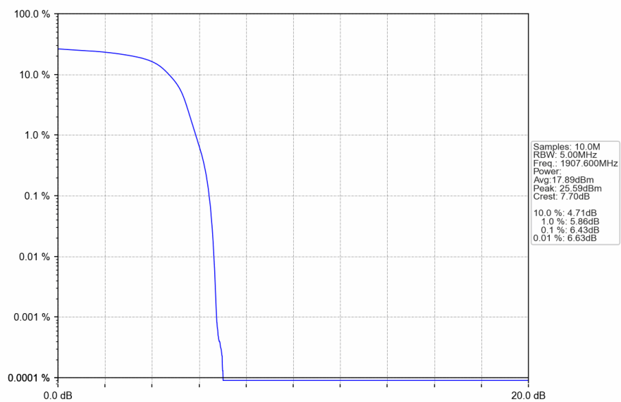
Band2_HSUPA_HCH_1907.6MHz_Subtest 1_NTNV
