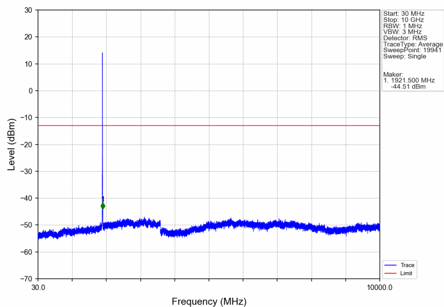
Band2_HSDPA_HCH_1907.6MHz_Subtest 1_NTNV
