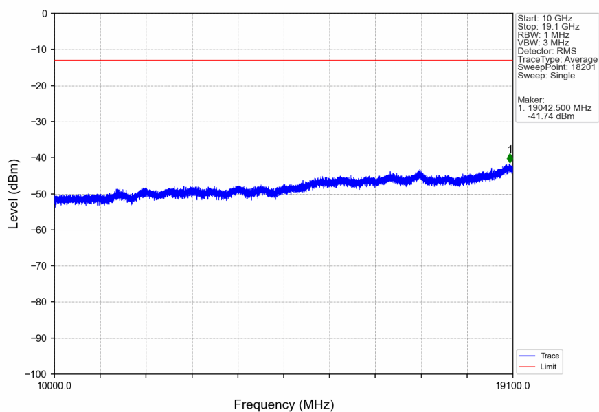
Band2_HSDPA_MCH_1880MHz_Subtest 1_NTNV
