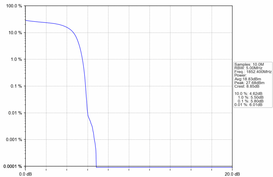
Band2_HSUPA_LCH_1852.4MHz_Subtest 1_NTNV
