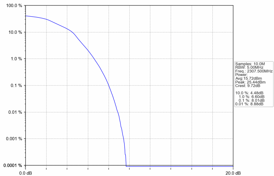
Band40a_5MHz_16QAM_LCH_2307.5MHz_RB_25_0_NTNV
