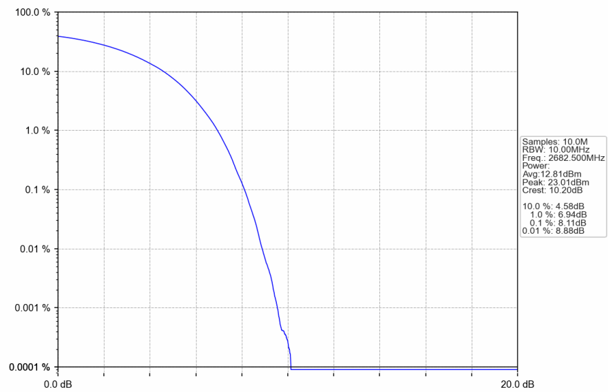
Band41_15MHz_16QAM_HCH_2682.5MHz_RB_75_0_NTNV
