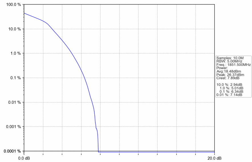
Band2_3MHz_16QAM_LCH_1851.5MHz_RB_15_0_NTNV
