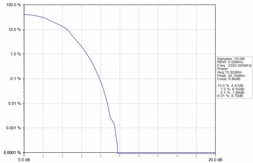
Band40b_5MHz_16QAM_MCH_2355MHz_RB_25_0_NTNV
