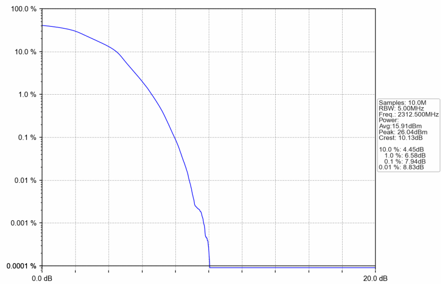
Band40a_5MHz_16QAM_HCH_2312.5MHz_RB_25_0_NTNV
