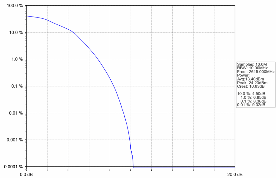
Band38_10MHz_16QAM_HCH_2615MHz_RB_50_0_NTNV
