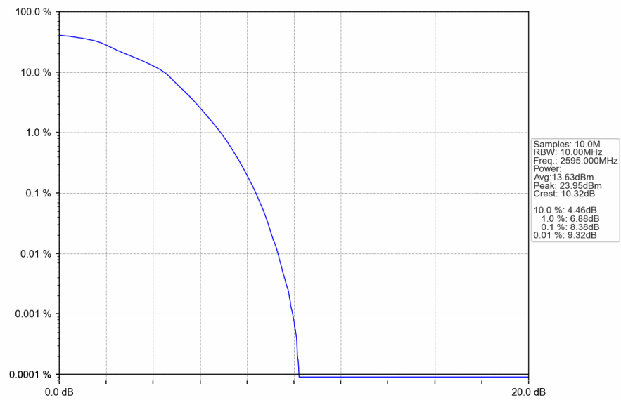
Band38_10MHz_16QAM_MCH_2595MHz_RB_50_0_NTNV
