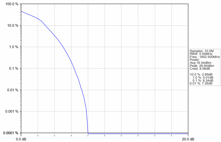
Band2_5MHz_16QAM_LCH_1852.5MHz_RB_25_0_NTNV
