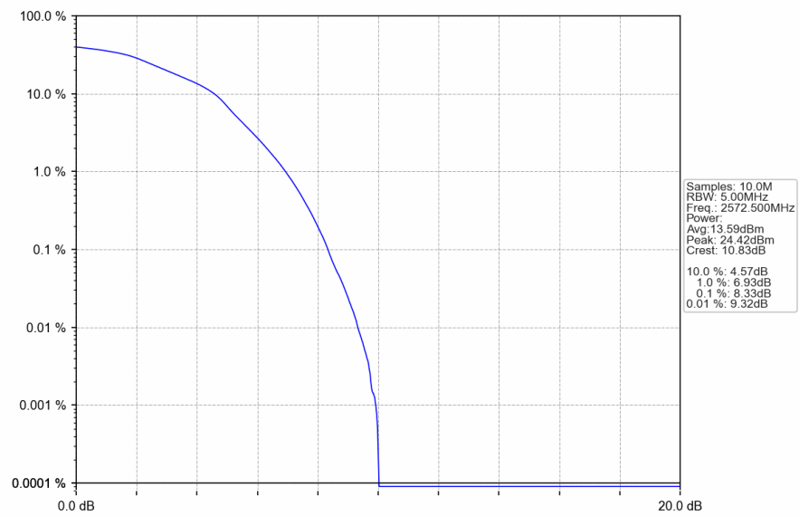
Band38_5MHz_16QAM_LCH_2572.5MHz_RB_25_0_NTNV
