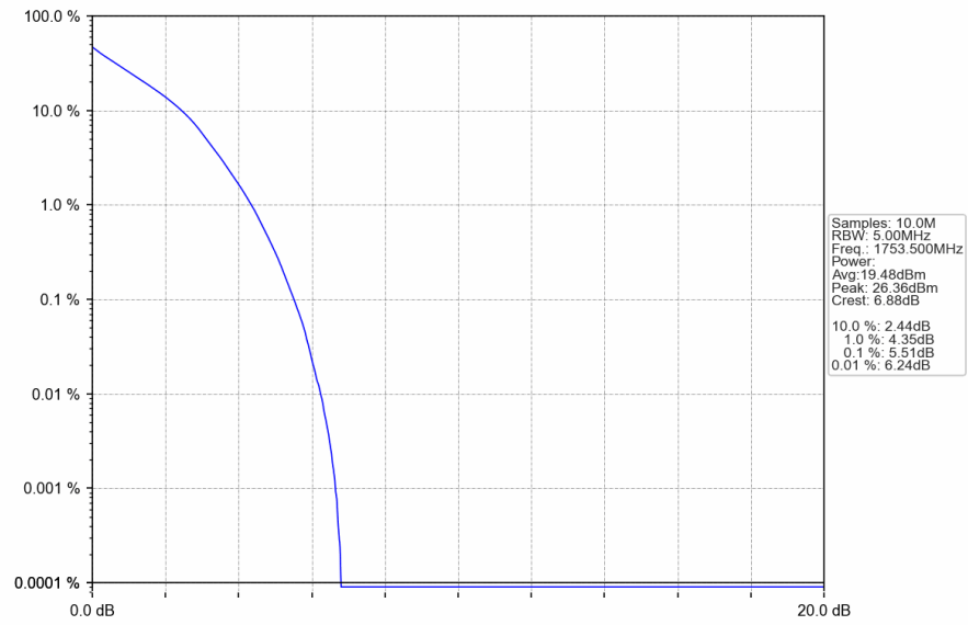
Band4_3MHz_QPSK_HCH_1753.5MHz_RB_15_0_NTNV
