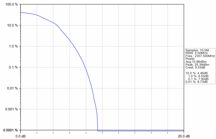
Band40b_5MHz_16QAM_HCH_2357.5MHz_RB_25_0_NTNV
