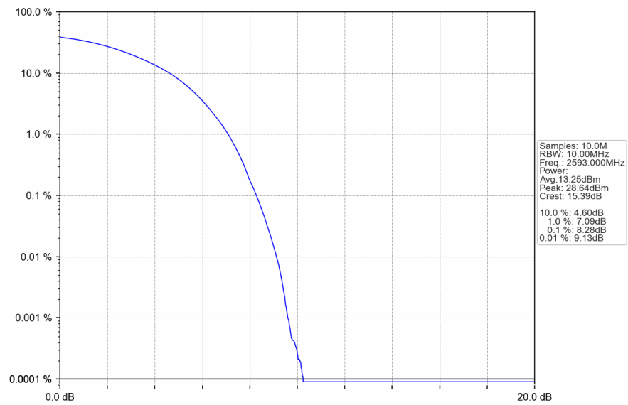
Band41_15MHz_16QAM_MCH_2593MHz_RB_75_0_NTNV
