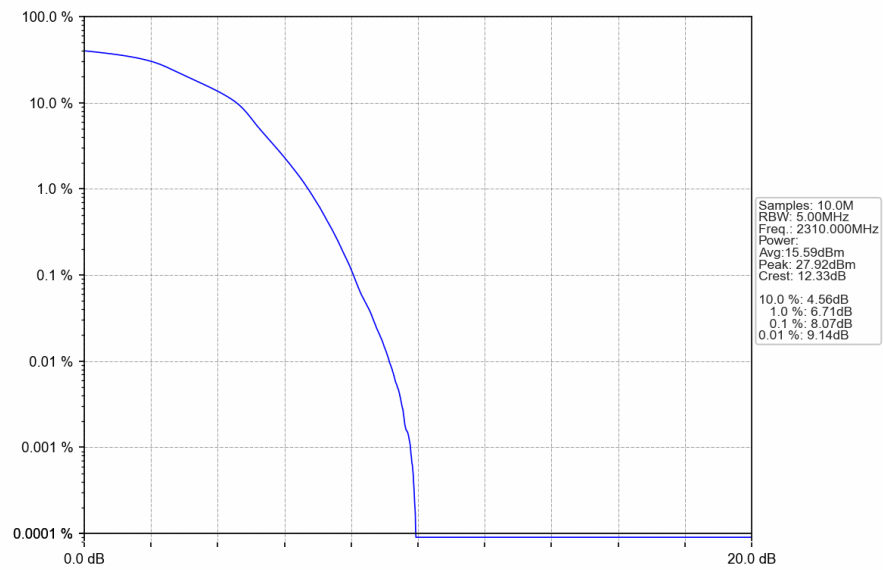
Band40a_5MHz_16QAM_MCH_2310MHz_RB_25_0_NTNV
