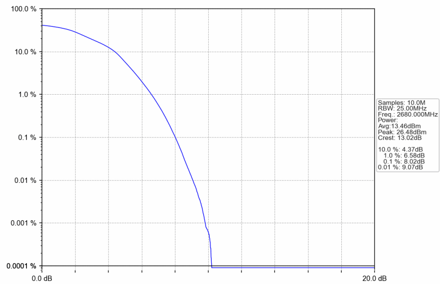
Band41_20MHz_16QAM_HCH_2680MHz_RB_100_0_NTNV
