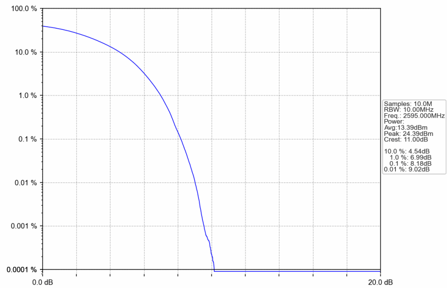
Band38_15MHz_16QAM_MCH_2595MHz_RB_75_0_NTNV
