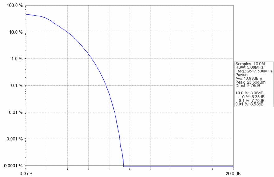
Band38_5MHz_QPSK_HCH_2617.5MHz_RB_25_0_NTNV
