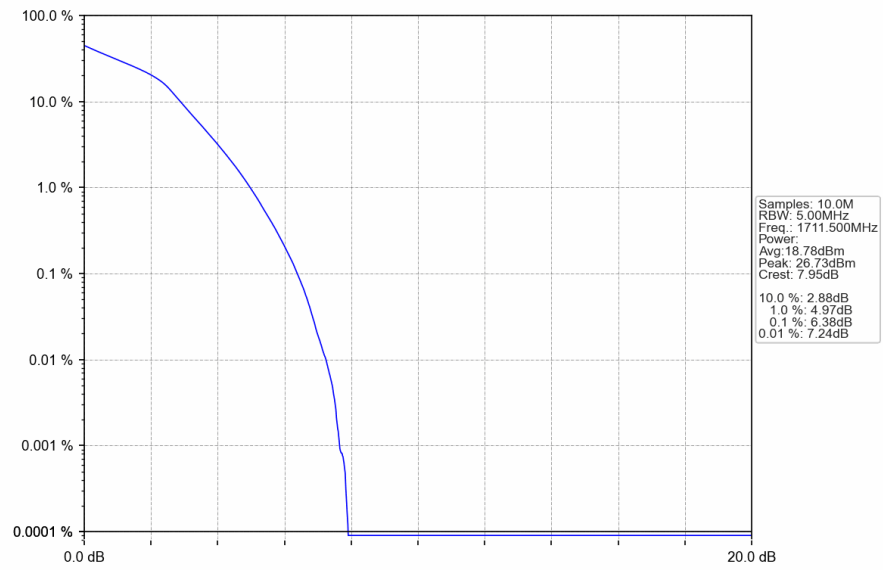
Band4_3MHz_16QAM_LCH_1711.5MHz_RB_15_0_NTNV
