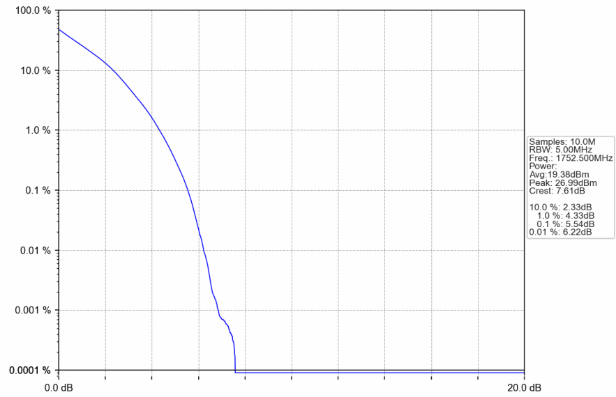
Band4_5MHz_QPSK_HCH_1752.5MHz_RB_25_0_NTNV
