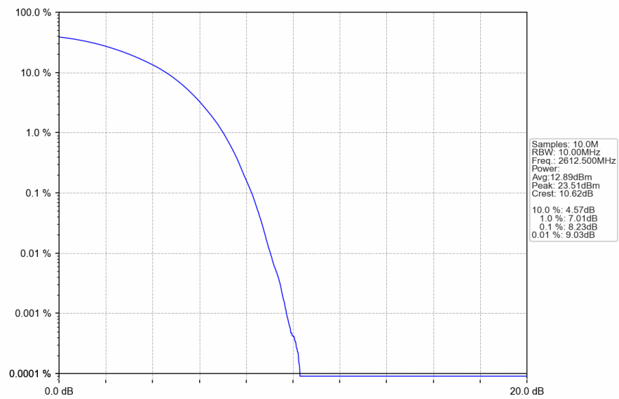
Band38_15MHz_16QAM_HCH_2612.5MHz_RB_75_0_NTNV
