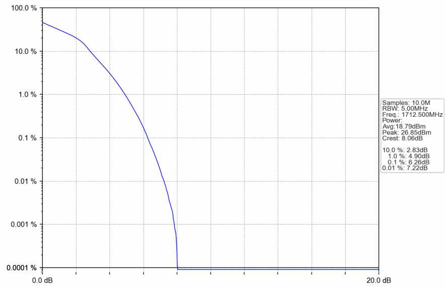
Band4_5MHz_16QAM_LCH_1712.5MHz_RB_25_0_NTNV
