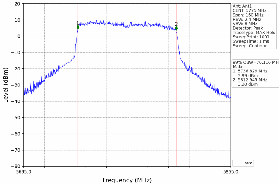
802.11ac(VHT80)_MCH_5775MHz_Ant1_NTNV
