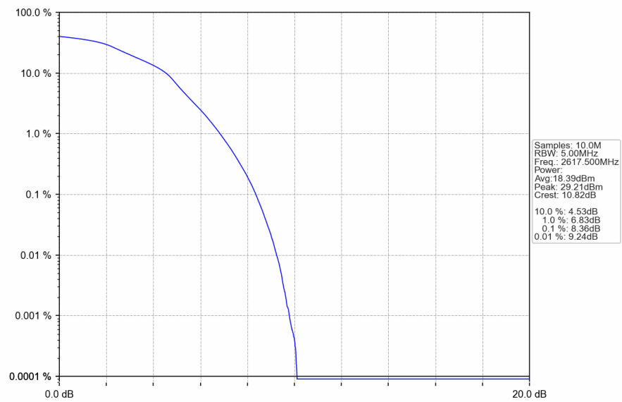
Band38_5MHz_16QAM_HCH_2617.5MHz_RB_25_0_NTNV
