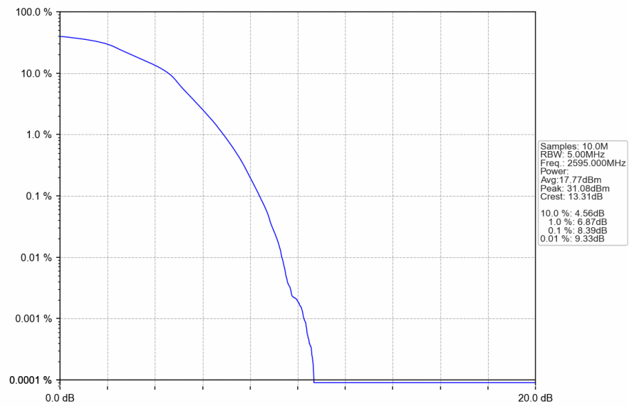
Band38_5MHz_16QAM_MCH_2595MHz_RB_25_0_NTNV
