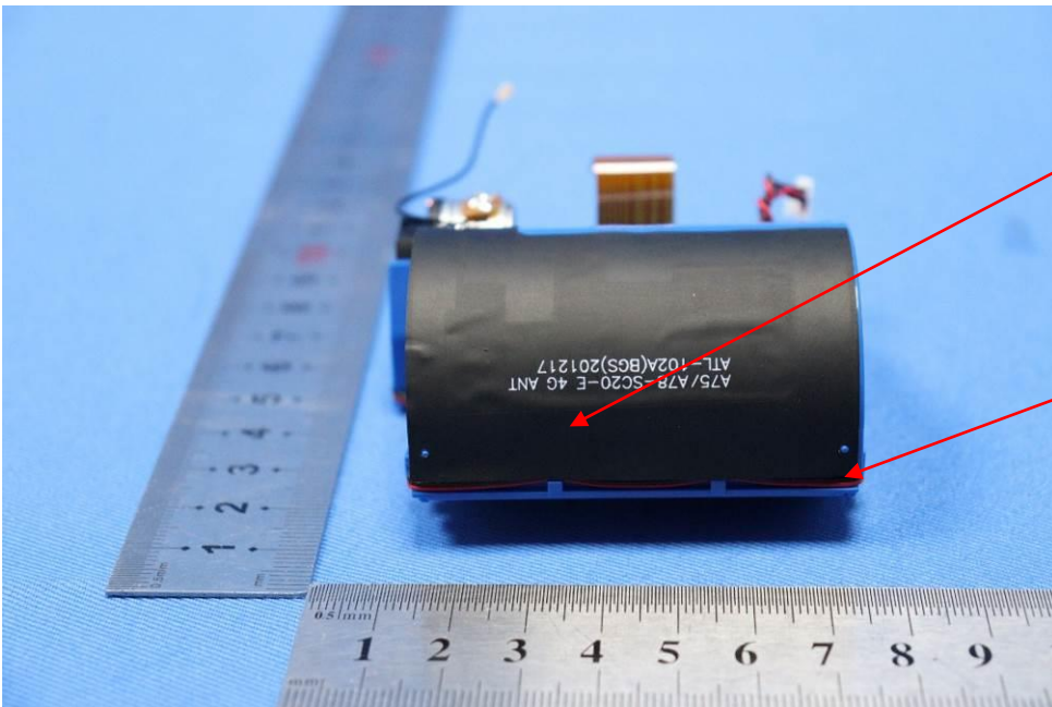
2G3G4G Antenna
