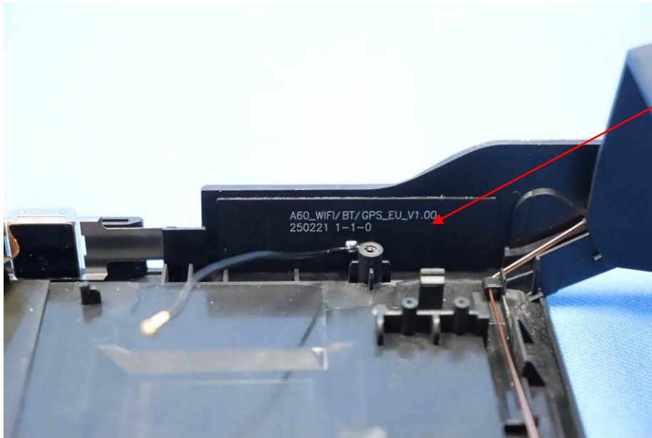
BT/Wi-Fi antenna
