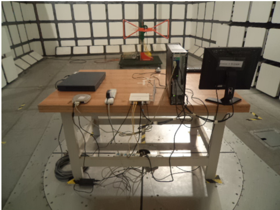
Spurious Radiated Emissions – Rear View (30 MHz - 1 GHz)
