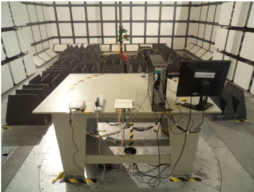
Spurious Radiated Emissions – Rear View (Above 1 GHz)
