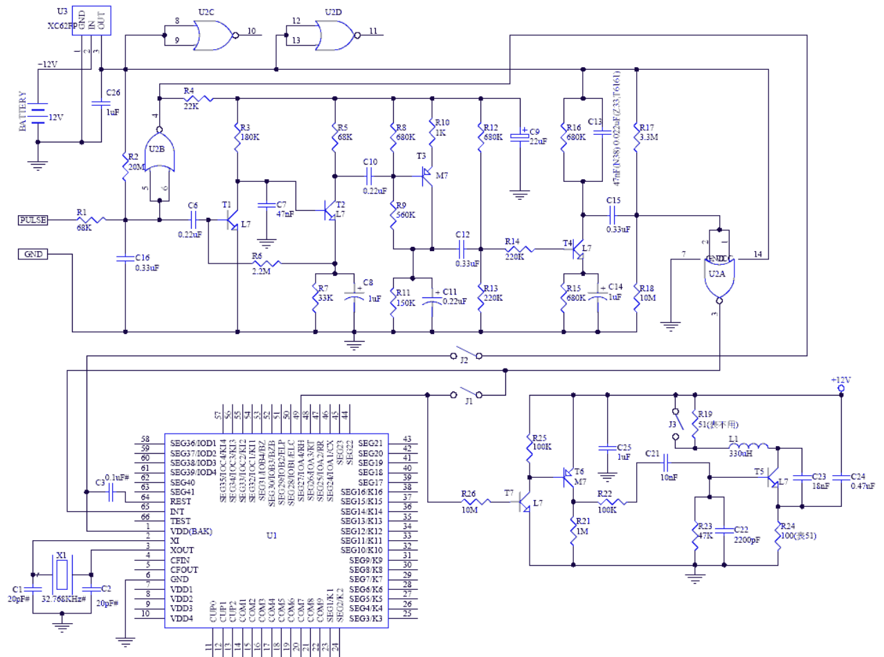
Figure 4.1 System Schematics
