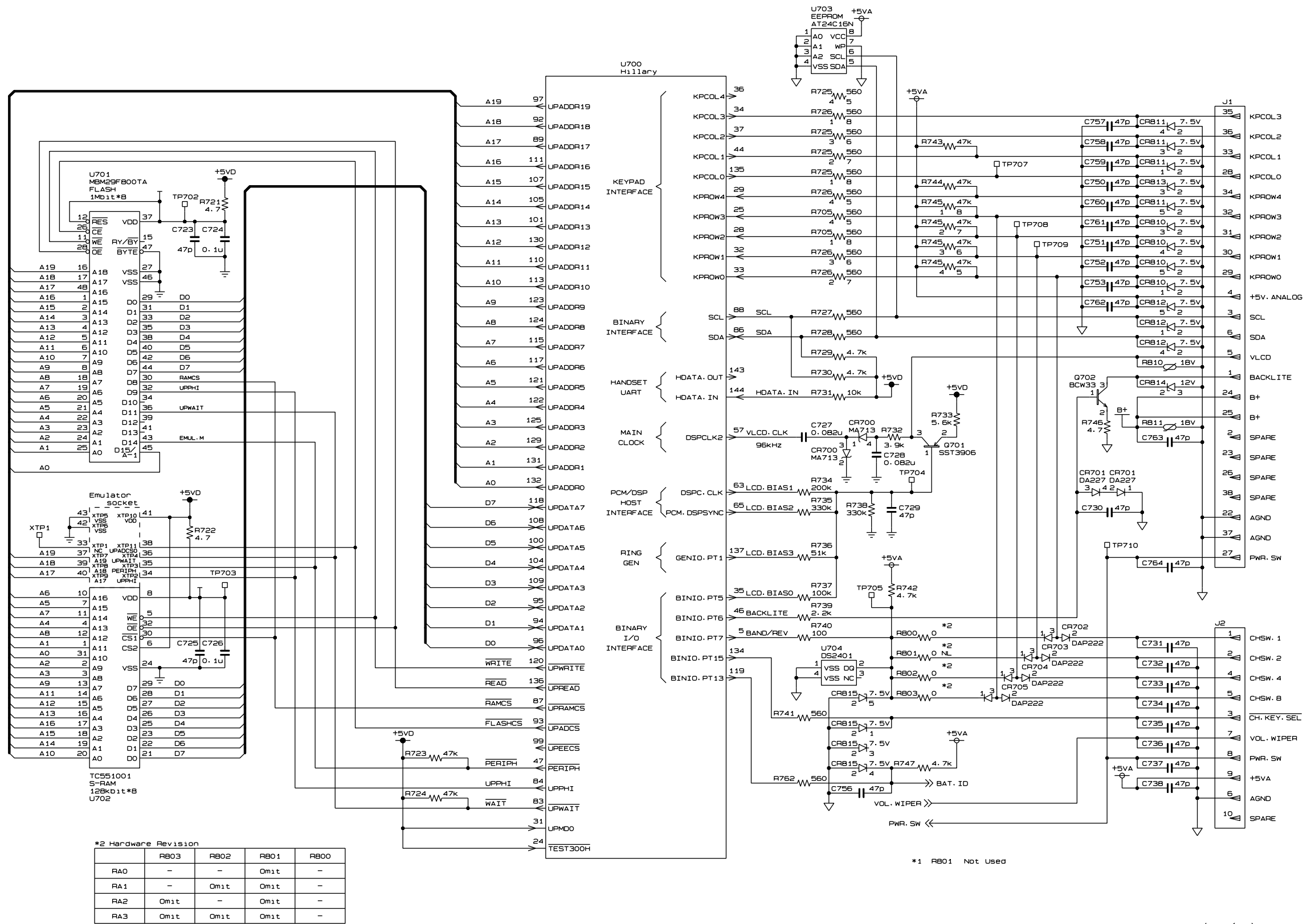
Jaguar 700P 900M MAIN Logic Block Schematic Diagram(4/6)
