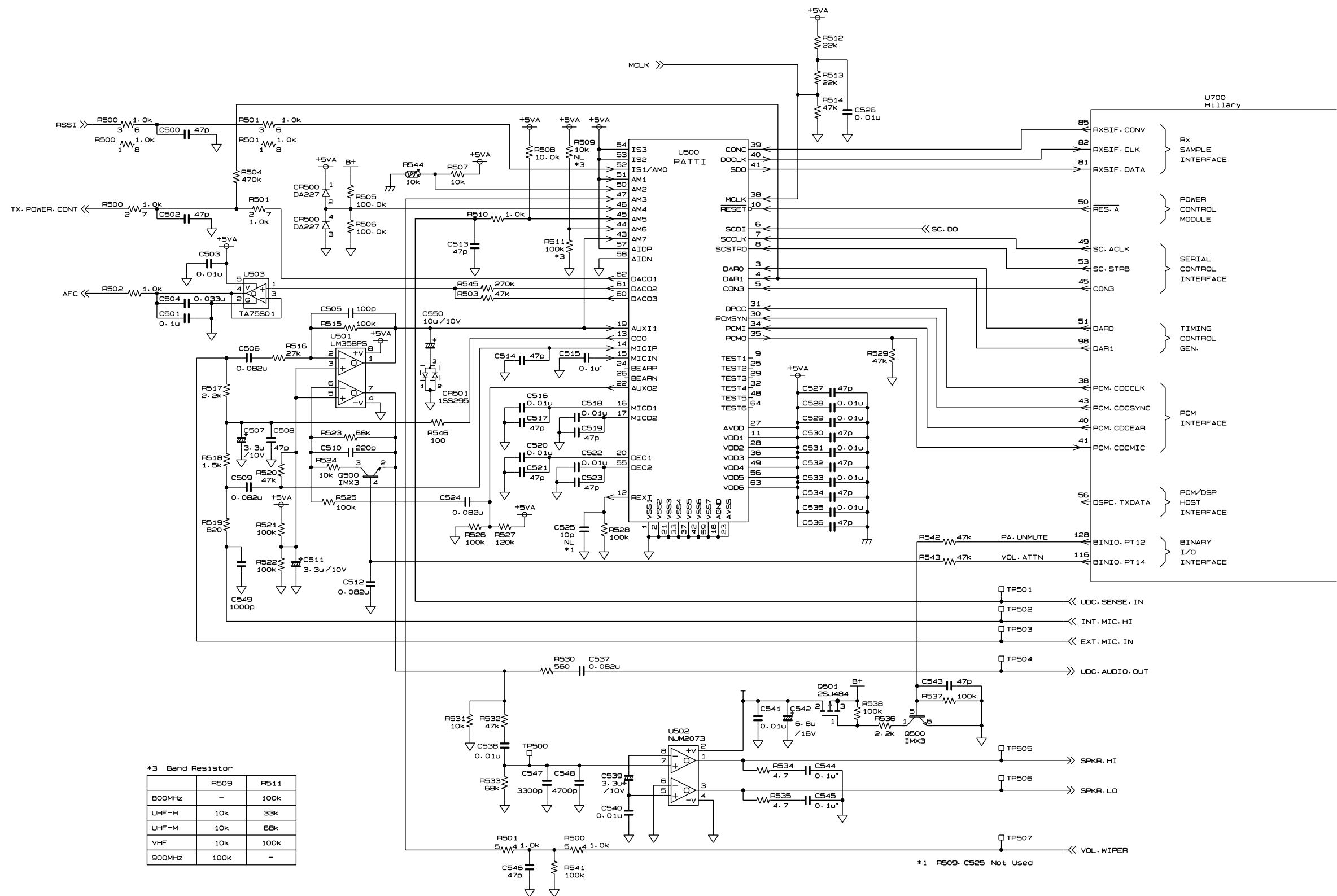
Jaguar 700P 900M MAin Logic Block Schematic Diagram(2/6)
