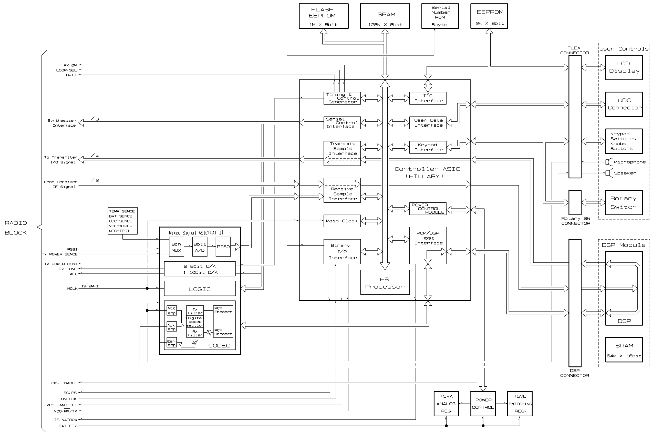
Jaguar 700P Logic Block Diagram
