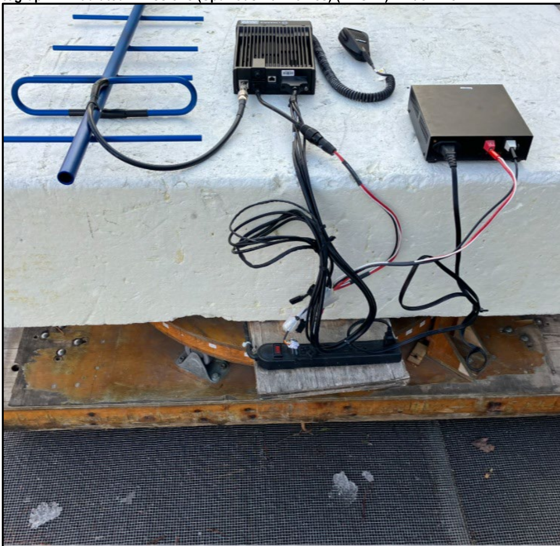
Photograph 2: Radiated Emissions (Spurious/Harmonics) (<1 GHz) – Back View
