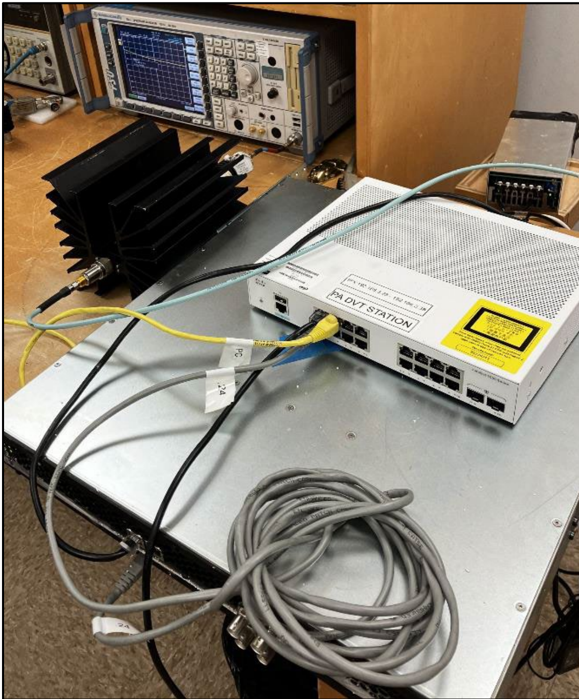
Photograph 3: RF Conducted Emissions
