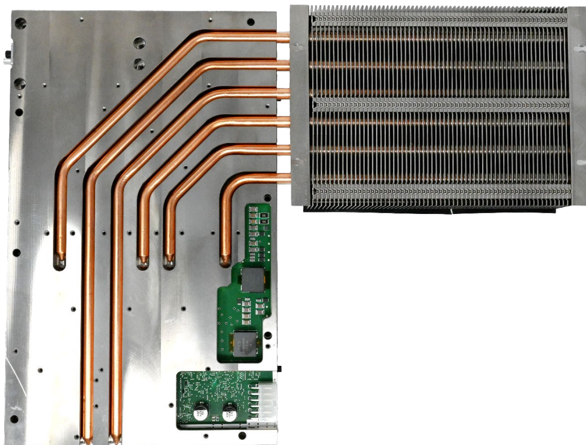
PA Assembly - Bottom
