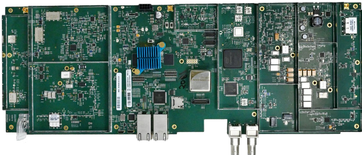
TRB Uncovered - Top View
