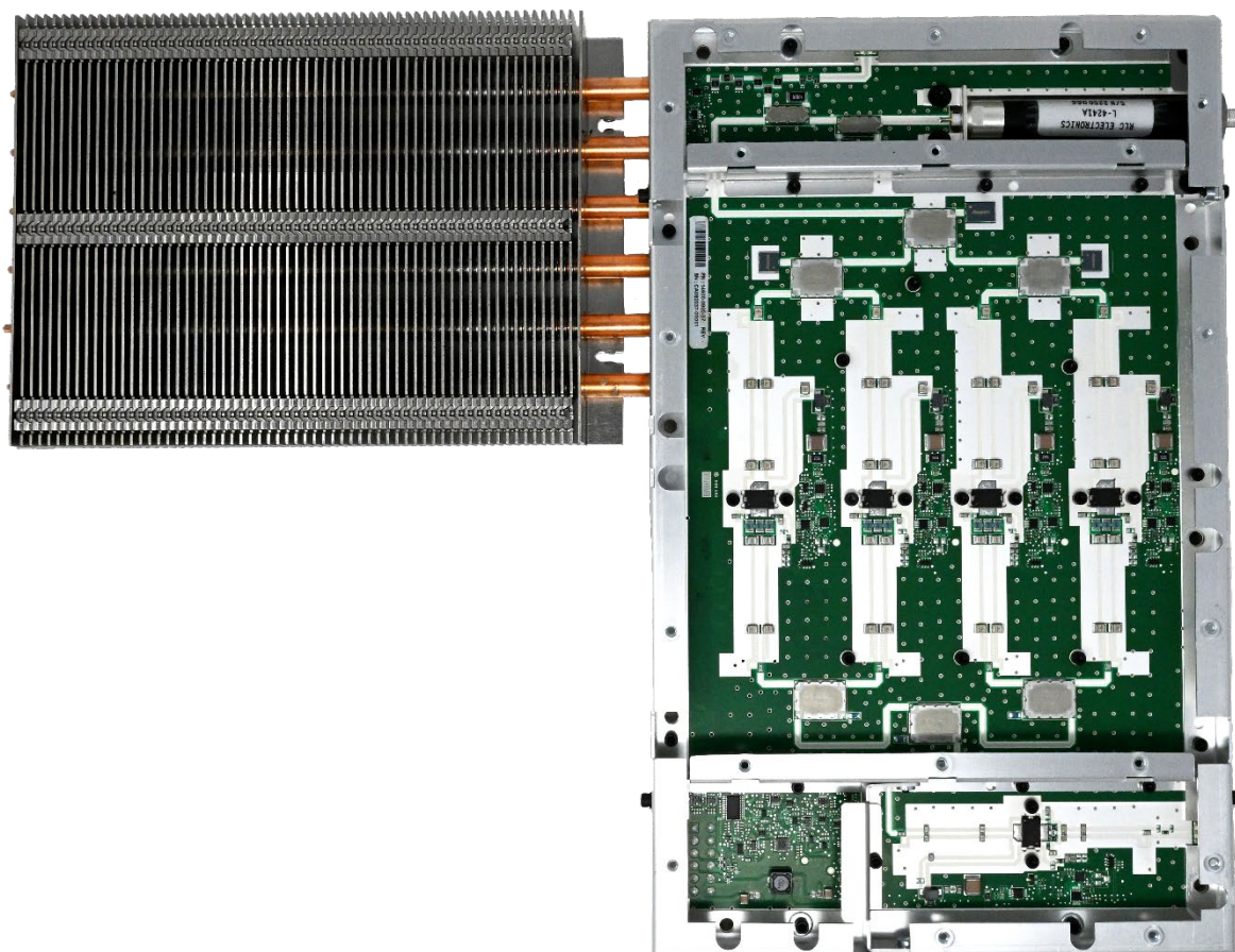
PA Assembly - Top
