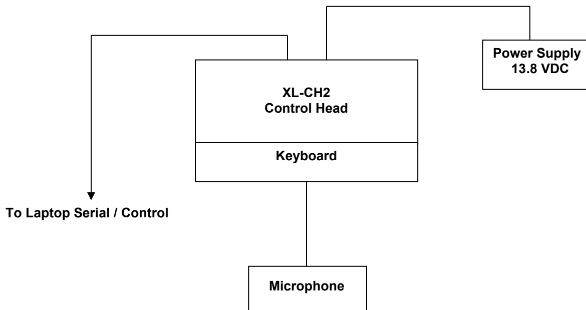
Figure 2-1: Configuration of Tested System
