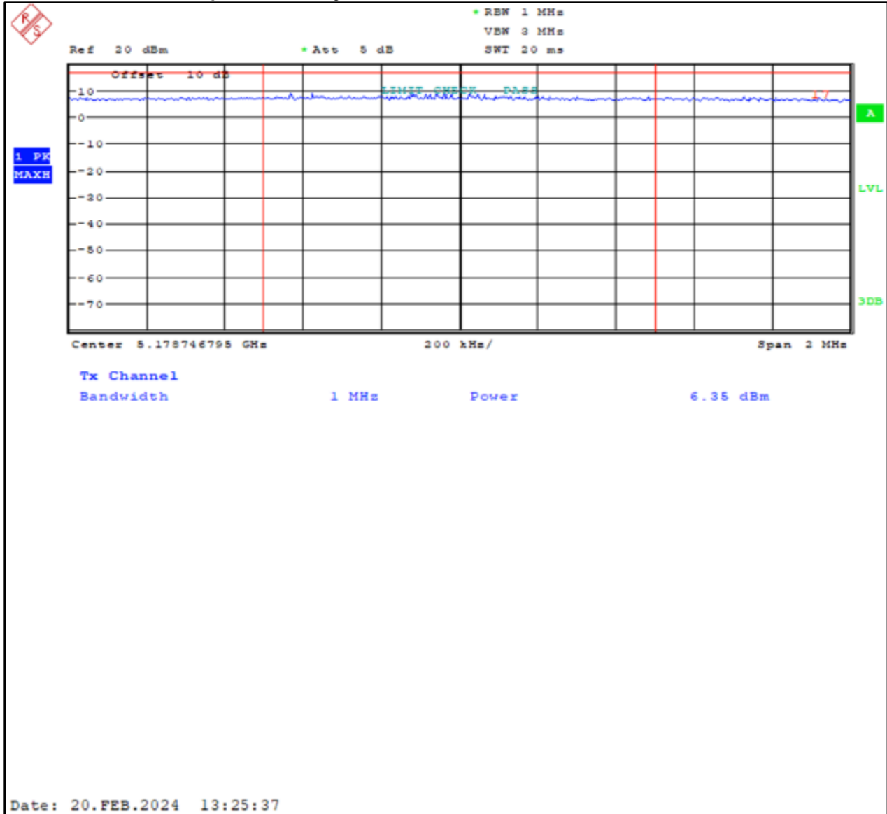
Plot 7-1: Power Spectral Density – 5180 MHz – 802.11a
