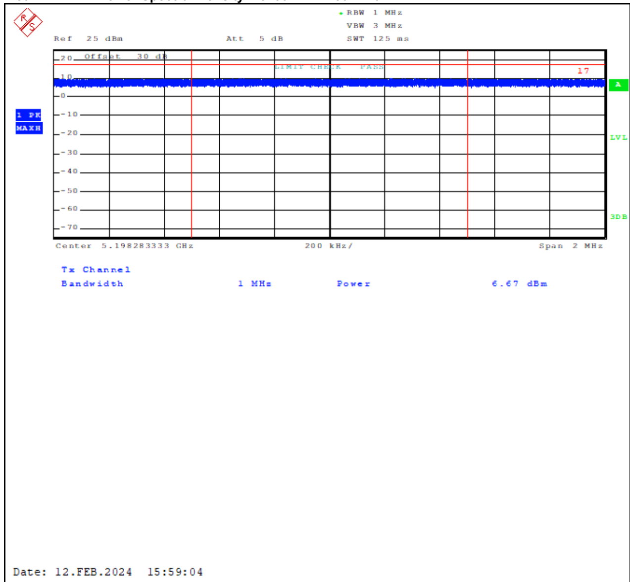
Plot 7-2: Power Spectral Density – 5200 MHz – 802.11a
