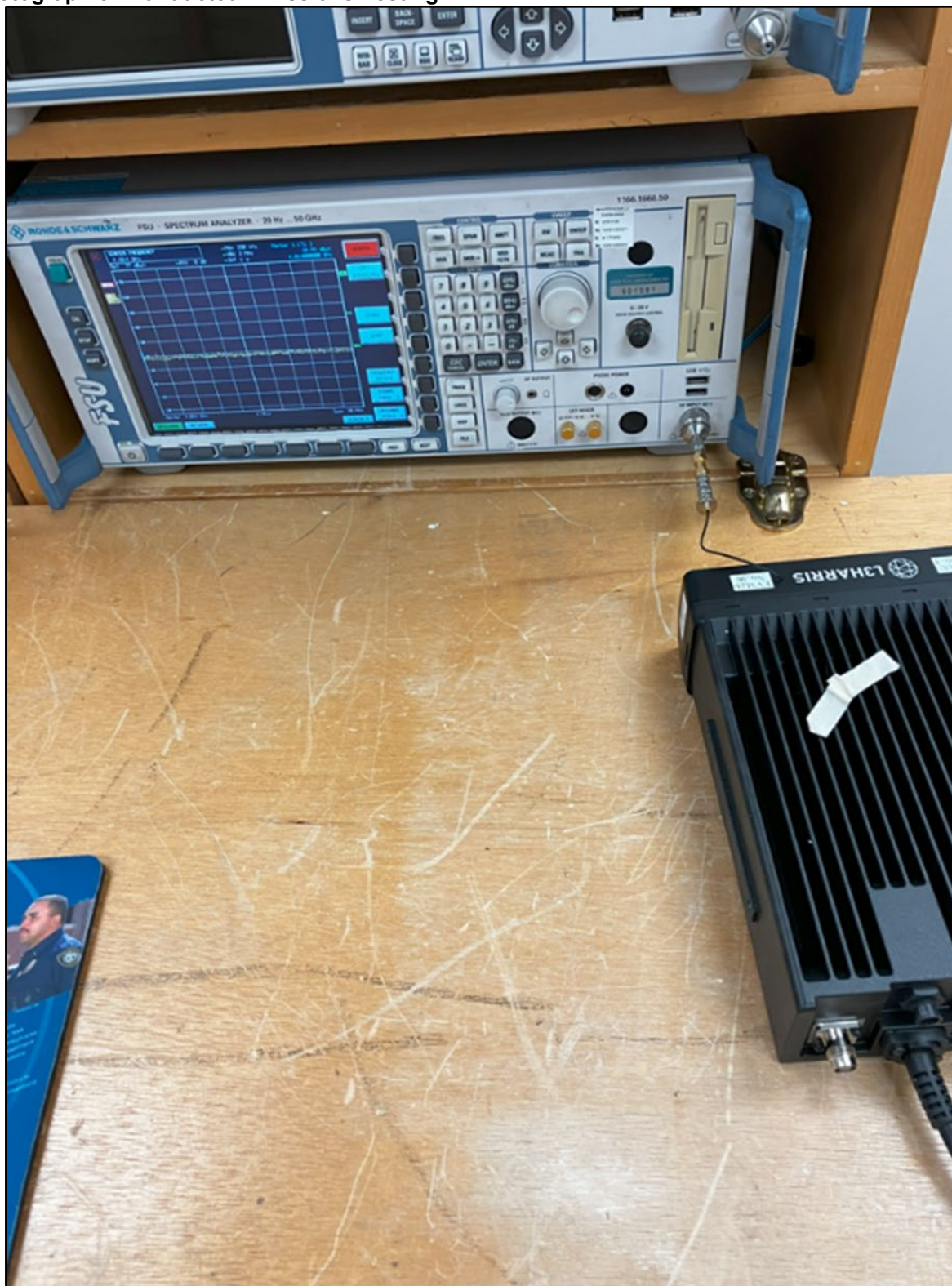
Photograph 5: Conducted Emissions Testing
