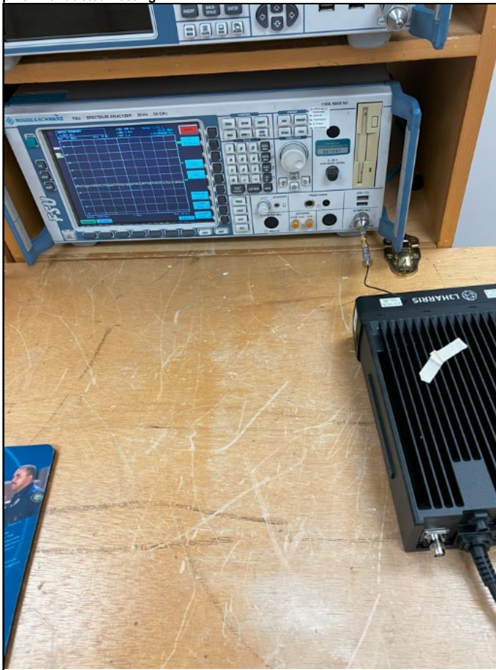
Photograph 5: Conducted Testing
