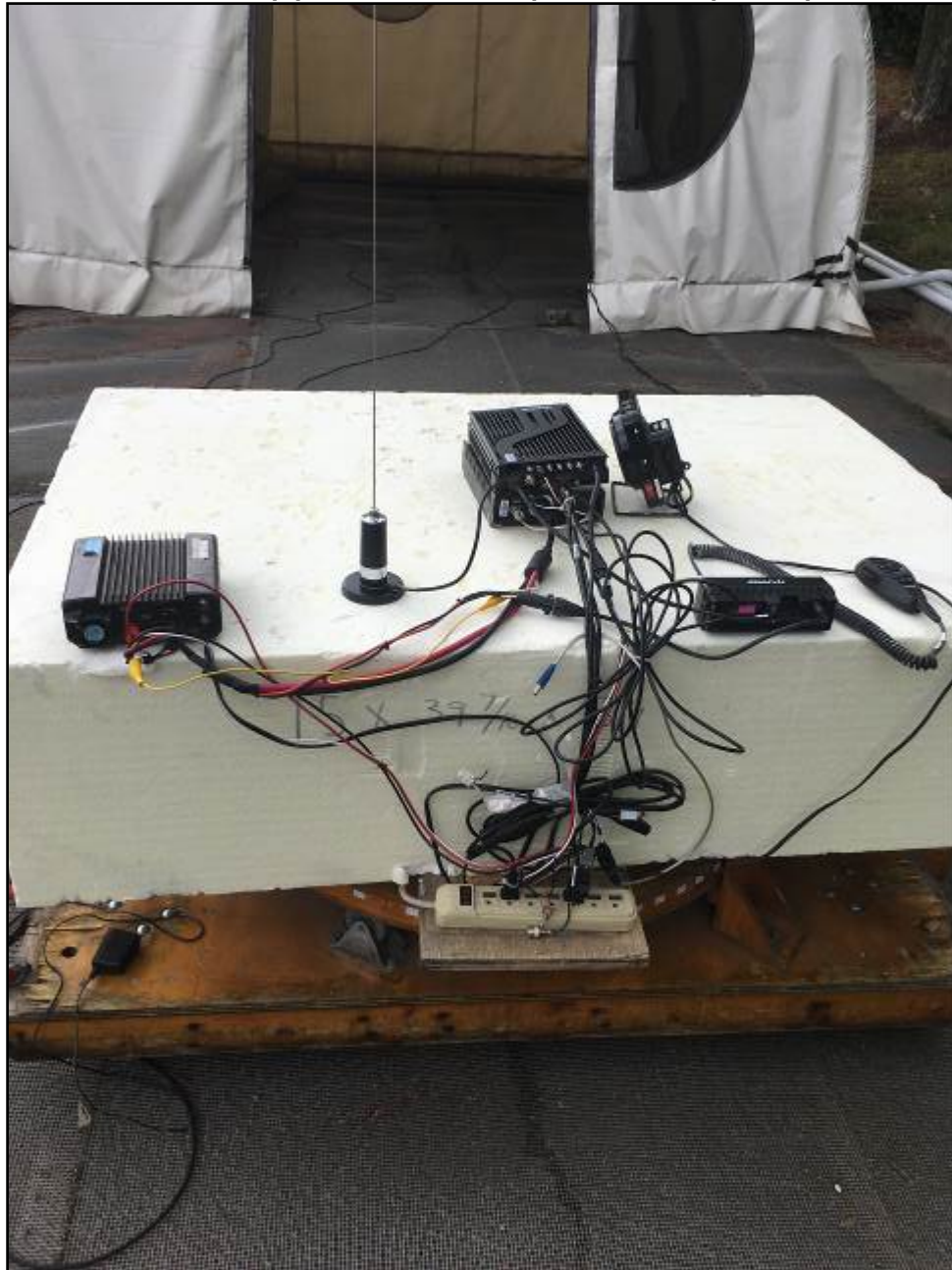
Photograph 2: Radiated Emissions (Spurious/Harmonics) – Back View (<1 GHz)
