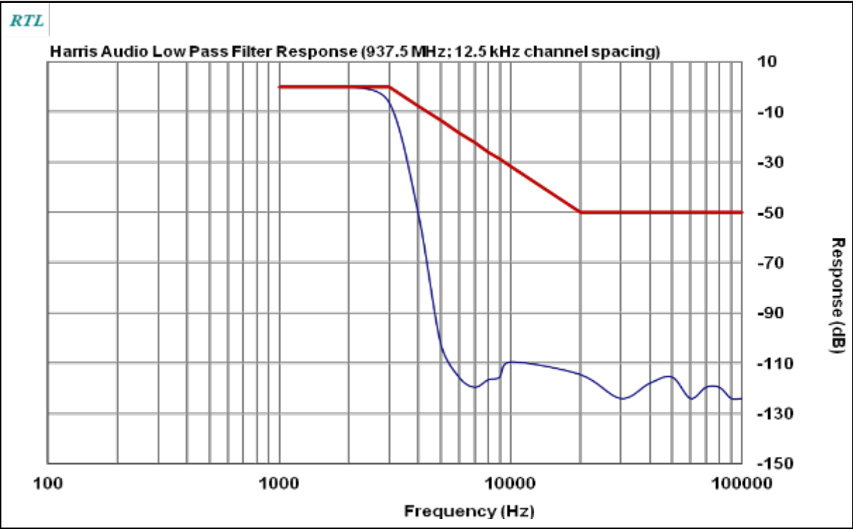
Plot 10-12: Modulation Characteristics – Audio Low Pass Filter – 937.5000 MHz (NB)
