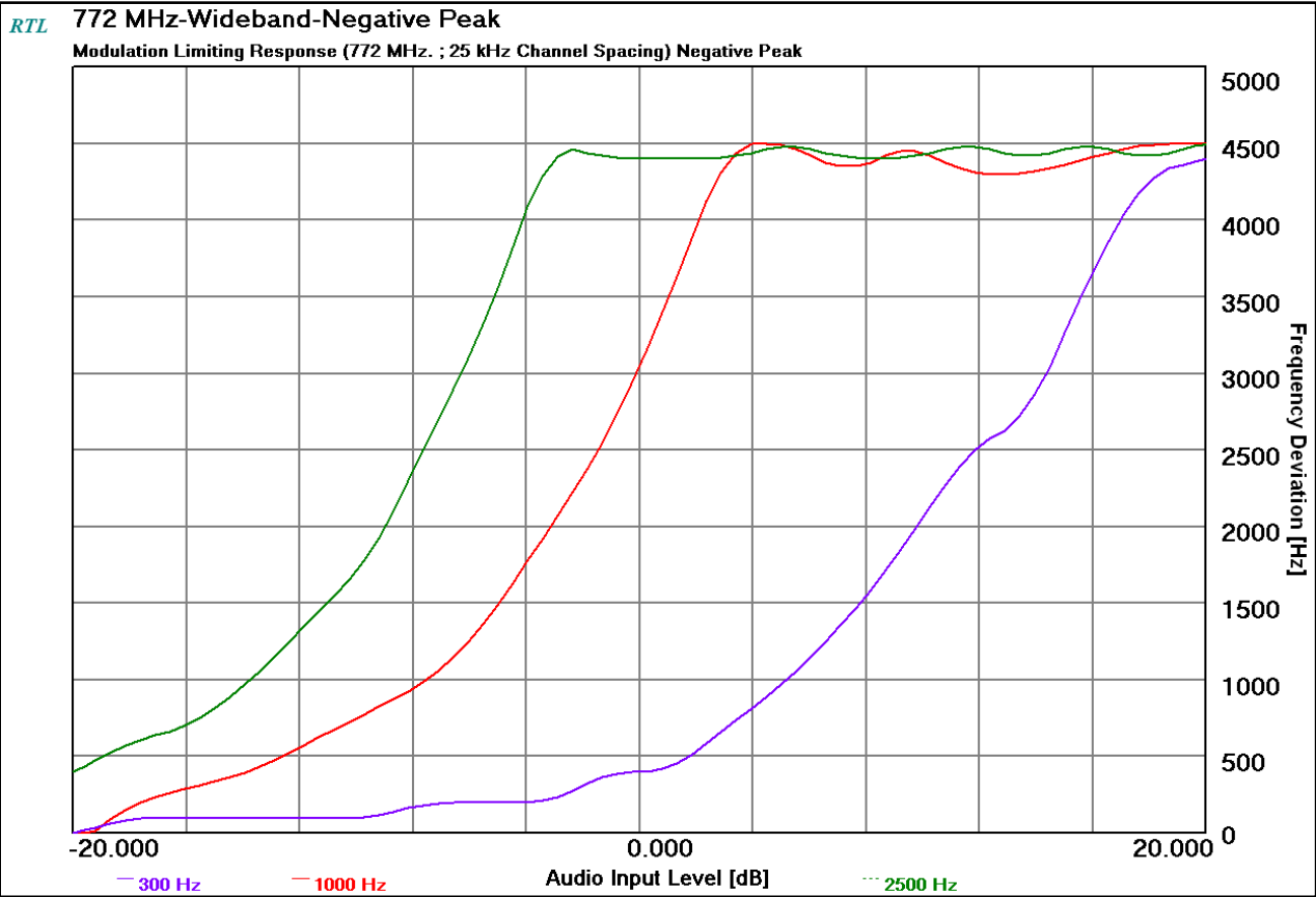
Plot 10-28: Modulation Characteristics – Modulation Limiting - 772.0000 MHz; (WB) Negative Peak
