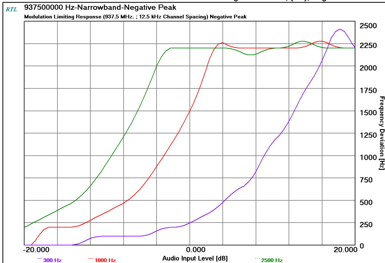
Plot 10-32: Modulation Characteristics – Modulation Limiting – 937.5 MHz; (NB); Negative Peak
