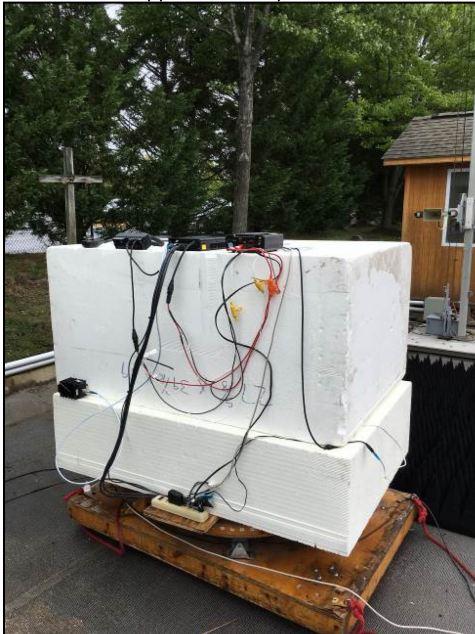
Photograph 2: Radiated Emissions (Spurious/Harmonics) – Back View
