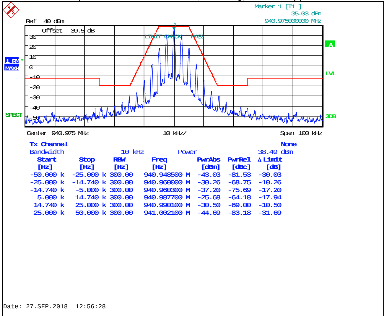
Plot 7-8: Occupied Bandwidth – 940.9750 MHz; NB Analog; Mask 24.133(2)
