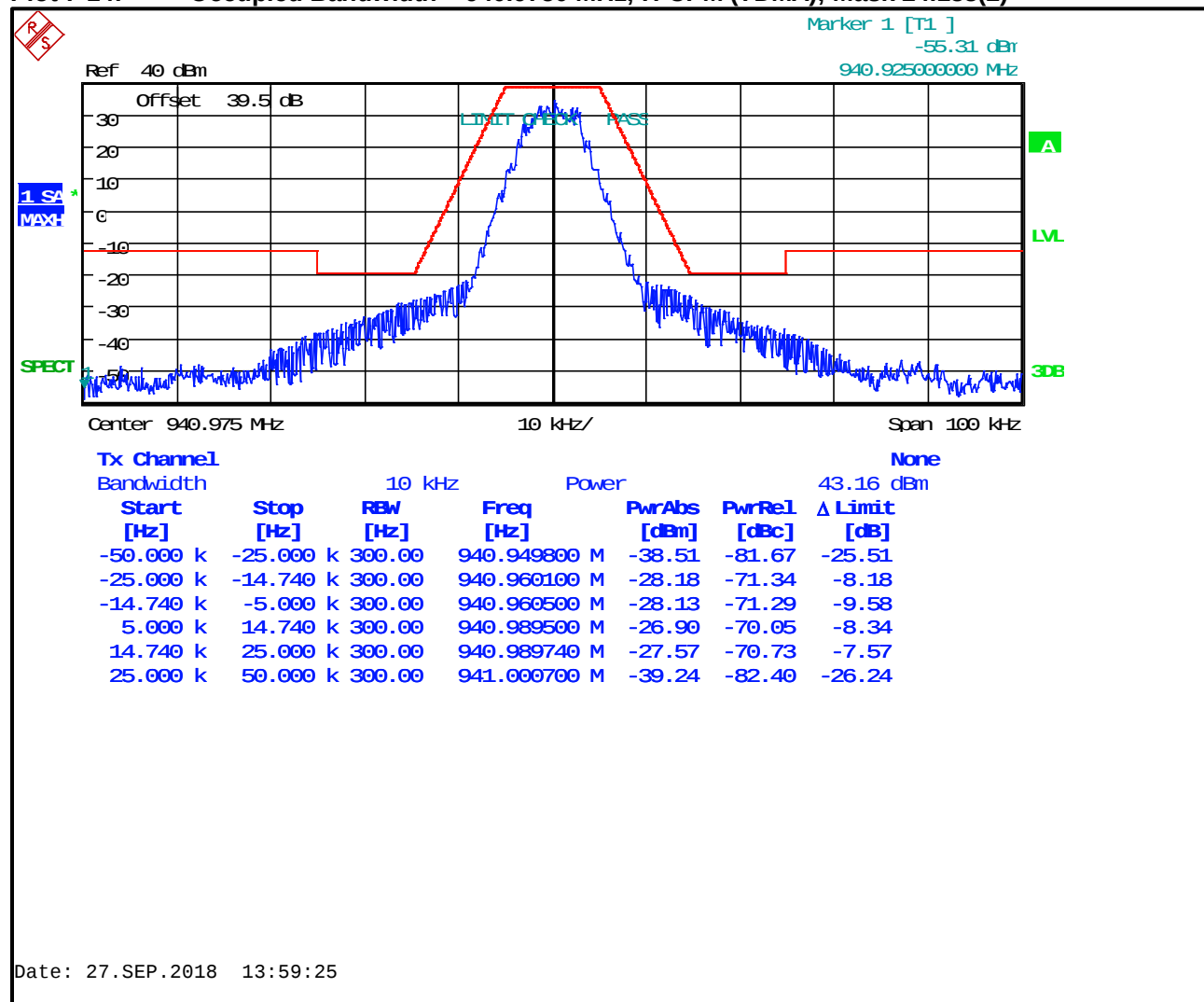
Plot 7-14: Occupied Bandwidth – 940.9750 MHz; H-CPM (TDMA); Mask 24.133(2)
