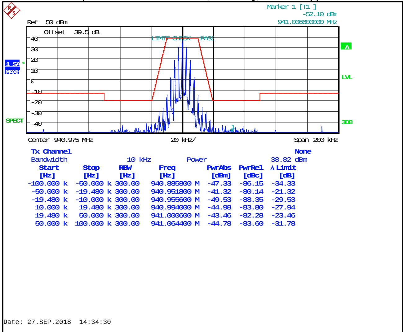
Plot 7-9: Occupied Bandwidth – 940.9750 MHz; WB Analog; Mask 24.133(1)
