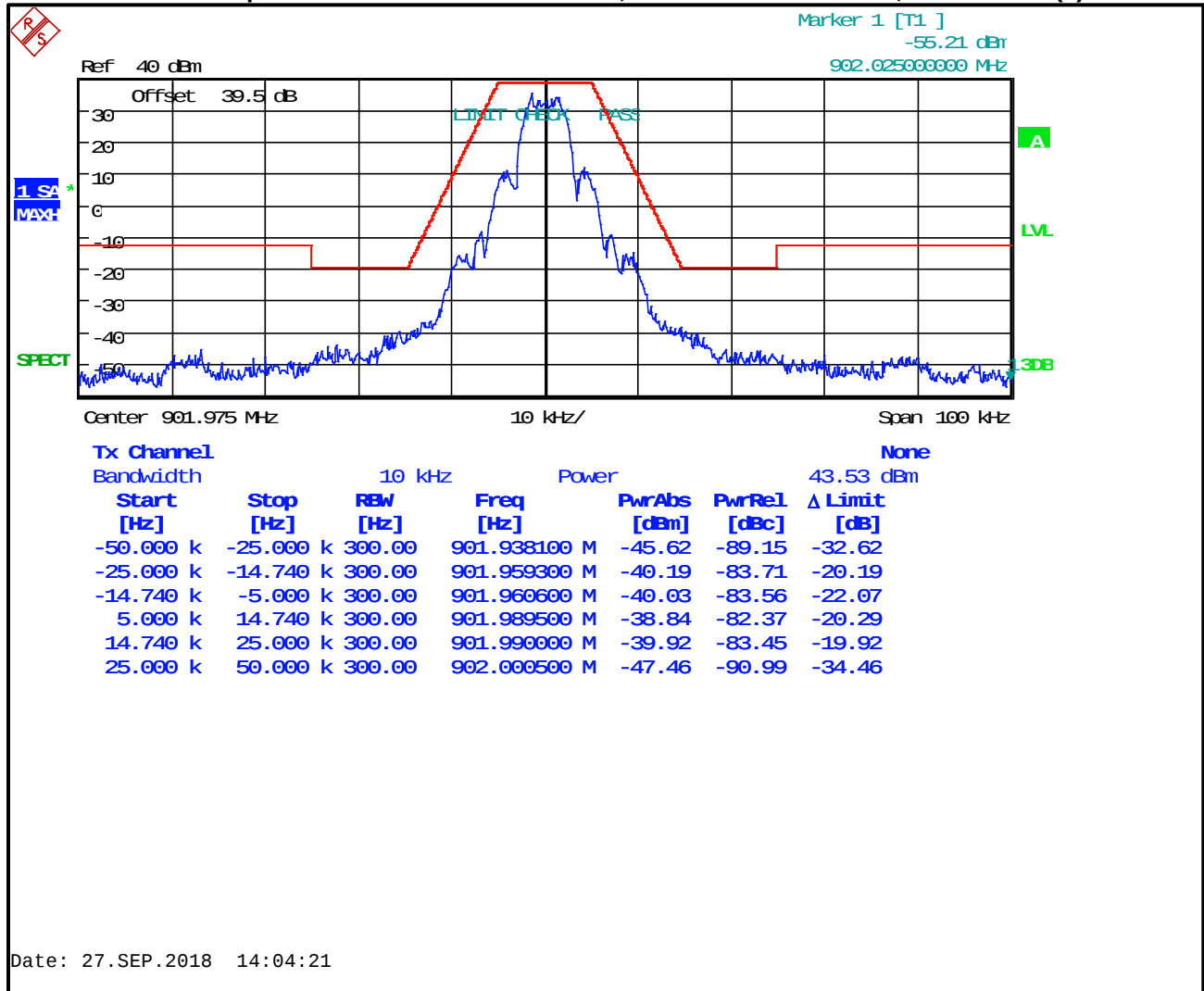
Plot 7-5: Occupied Bandwidth – 901.9750 MHz; 2-Level FSK 4800 XNB; Mask 24.133(2)
