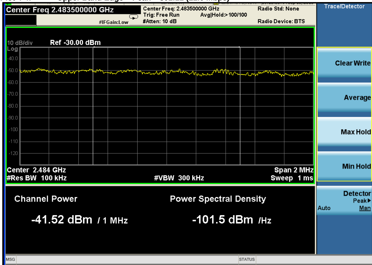
Plot 4-4: Upper Band Edge – Peak – 802.11 (11.0 Mbps)
