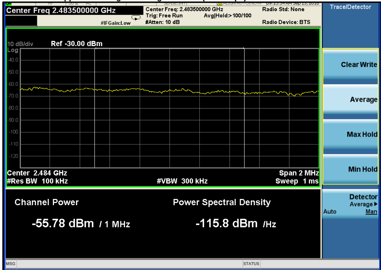
Plot 4-3: Upper Band Edge – Average – 802.11 (11.0 Mbps)
