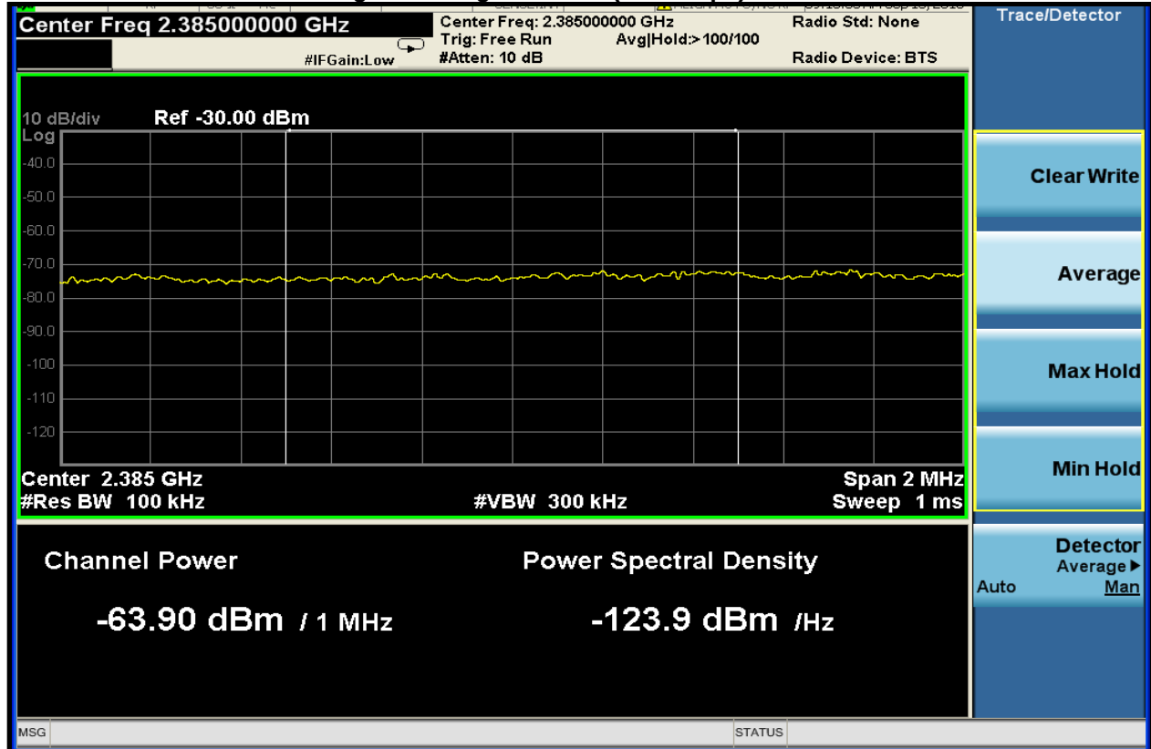
Plot 4-1: Lower Band Edge – Average – 802.11 (11.0 Mbps)
