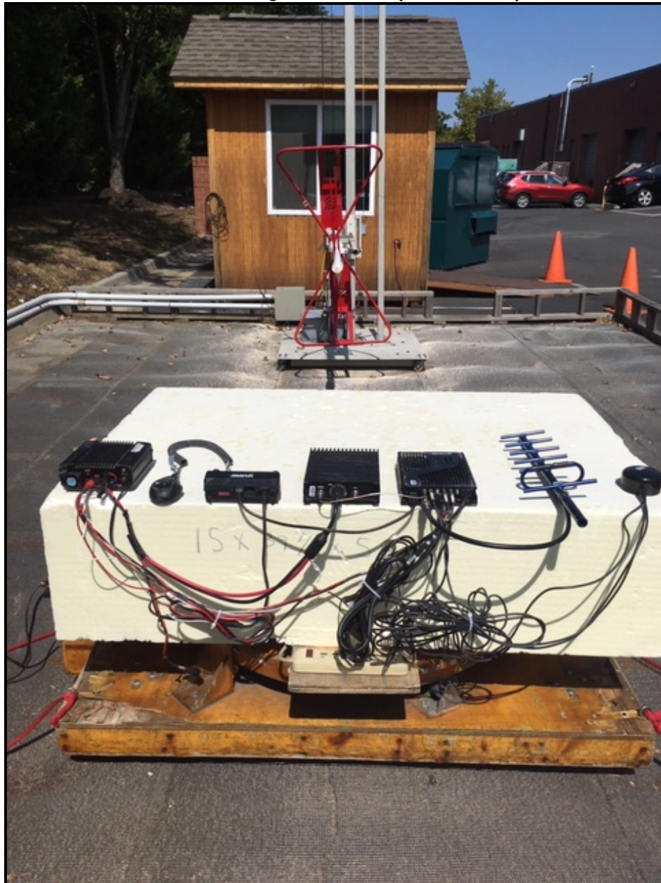
Photograph 4: Radiated Emissions Testing – Back View (Below 1 GHz)
