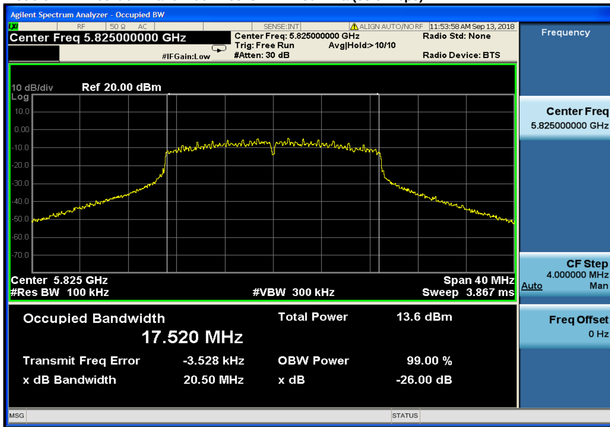
Plot 6-9: 99% dB Bandwidth – 5825 MHz – 802.11a (58.5 Mbps)
