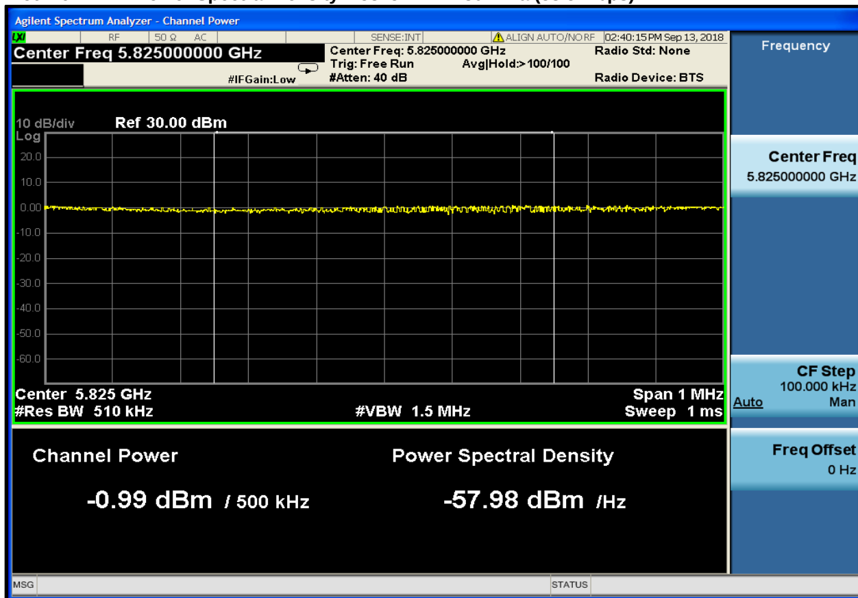
Plot 7-6: Power Spectral Density – 5825 MHz – 802.11a (58.5 Mbps)
