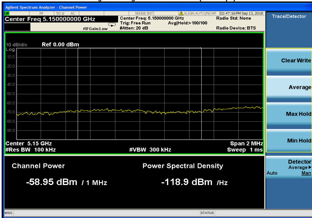
Plot 4-1: Lower Band Edge – Average – U-NII1 – 802.11a (58.5 Mbps)
