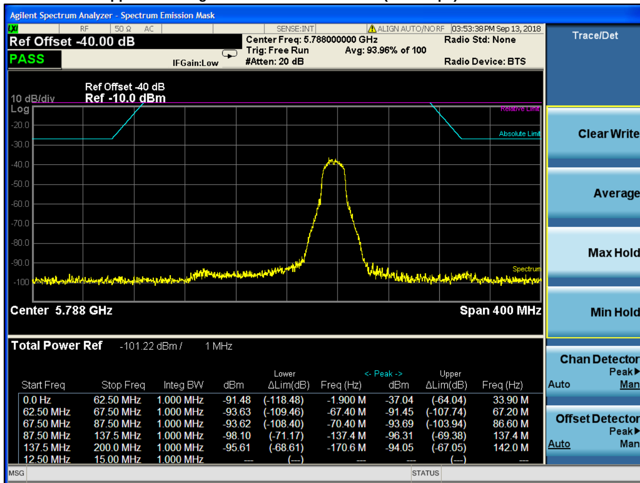
Plot 4-8: Upper Band Edge – Peak – U-NII3 – 802.11a (58.5 Mbps)
