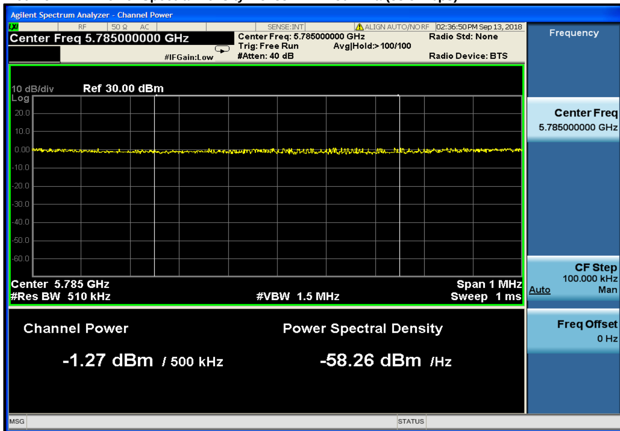
Plot 7-5: Power Spectral Density – 5785 MHz – 802.11a (58.5 Mbps)
