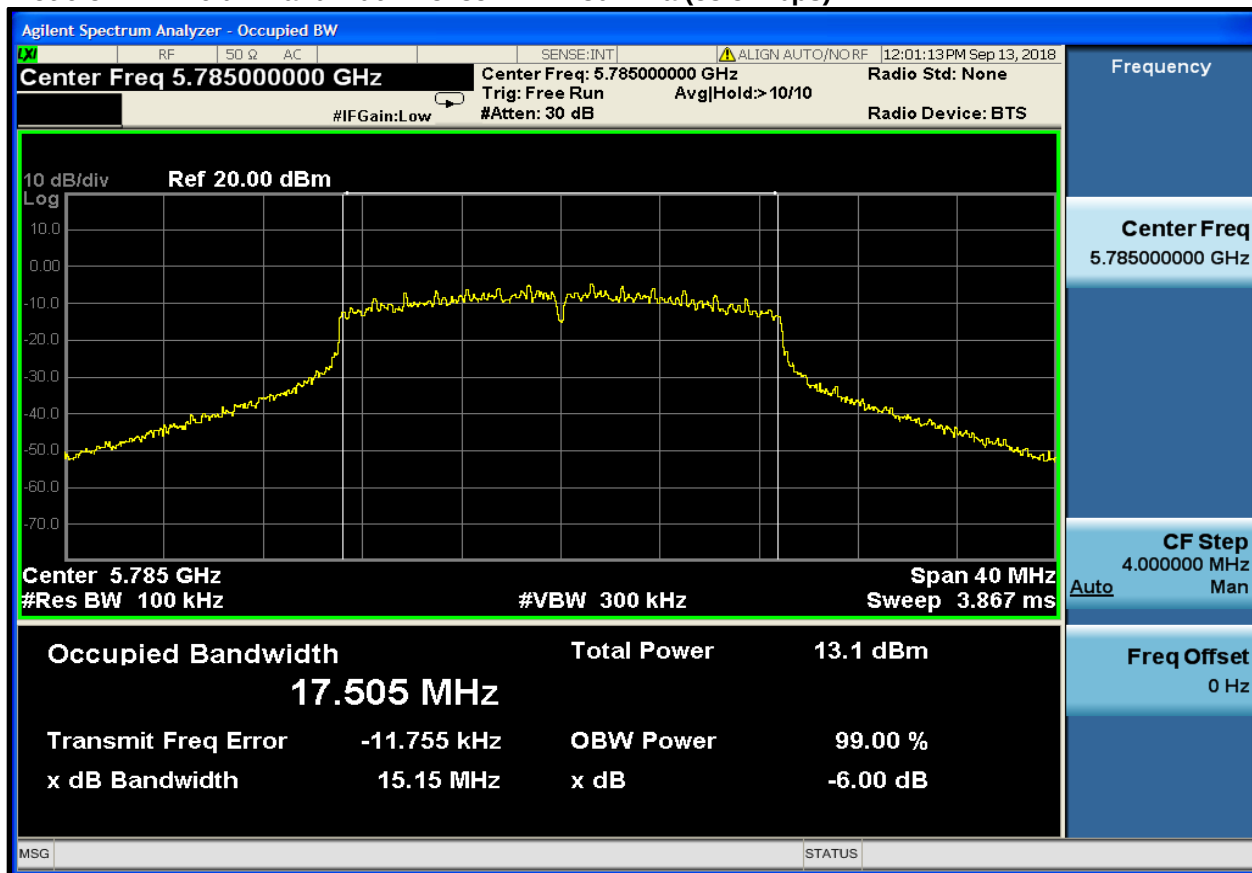
Plot 6-5: 6 dB Bandwidth – 5785 MHz – 802.11a (58.5 Mbps)
