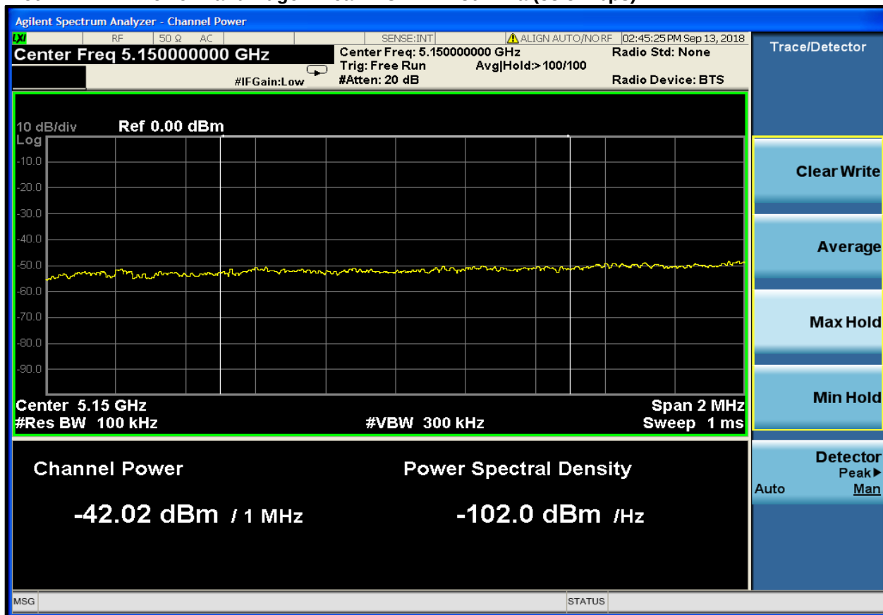
Plot 4-2: Lower Band Edge – Peak – U-NII1 – 802.11a (58.5 Mbps)
