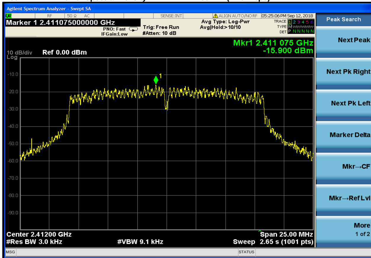
Plot 7-1: Power Spectral Density – 2412 MHz – 802.11 (11.0 Mbps)
