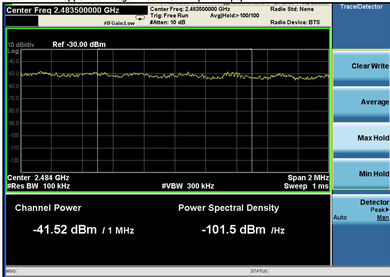
Plot 4-4: Upper Band Edge – Peak – 802.11 (11.0 Mbps)
