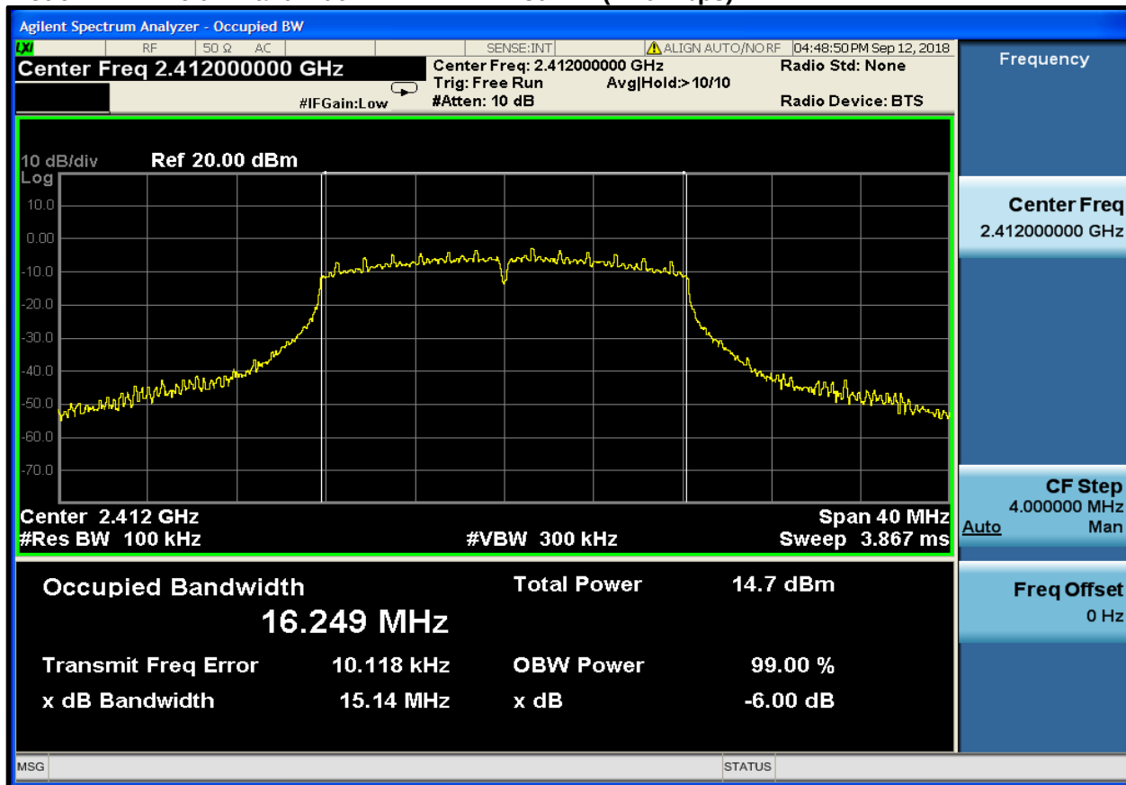
Plot 6-1: 6 dB Bandwidth – 2412 MHz – 802.11 (11.0 Mbps)
