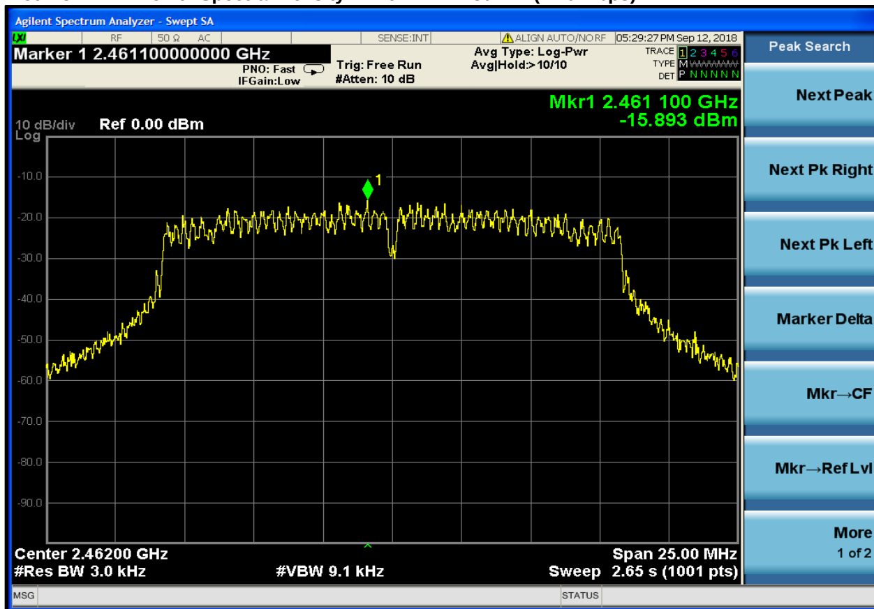
Plot 7-3: Power Spectral Density – 2462 MHz – 802.11 (11.0 Mbps)
