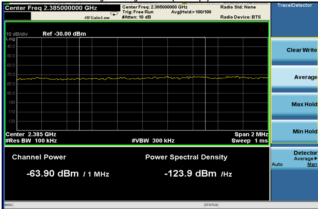
Plot 4-1: Lower Band Edge – Average – 802.11 (11.0 Mbps)
