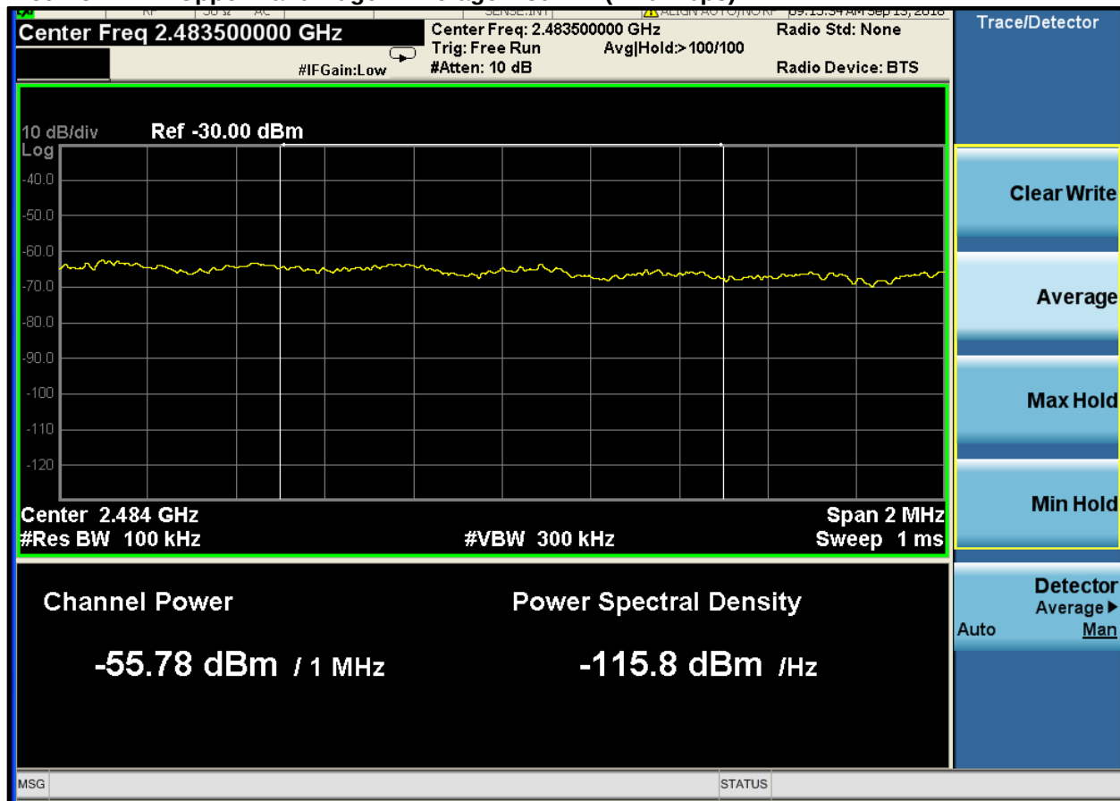
Plot 4-3: Upper Band Edge – Average – 802.11 (11.0 Mbps)
