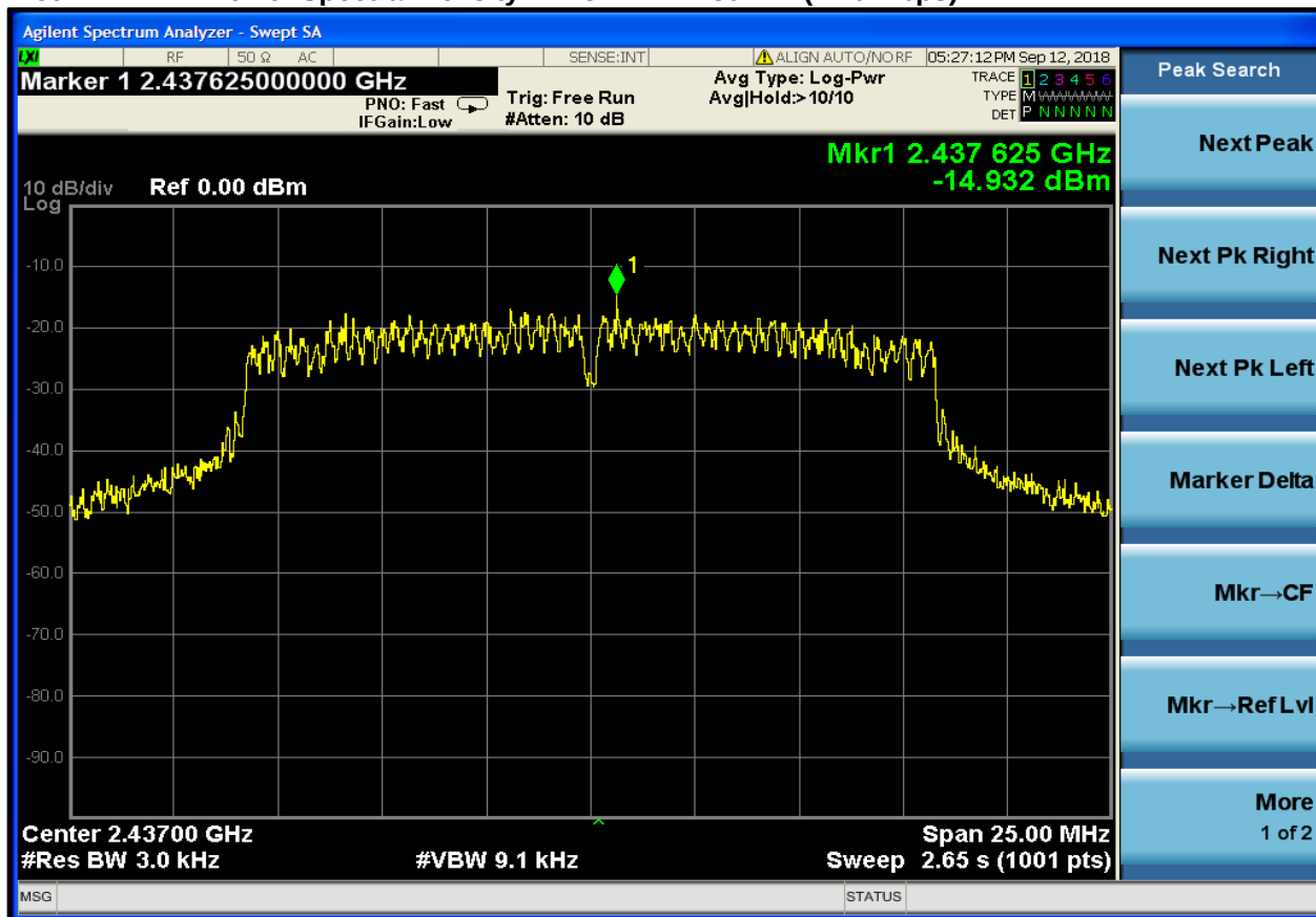
Plot 7-2: Power Spectral Density – 2437 MHz – 802.11 (11.0 Mbps)
