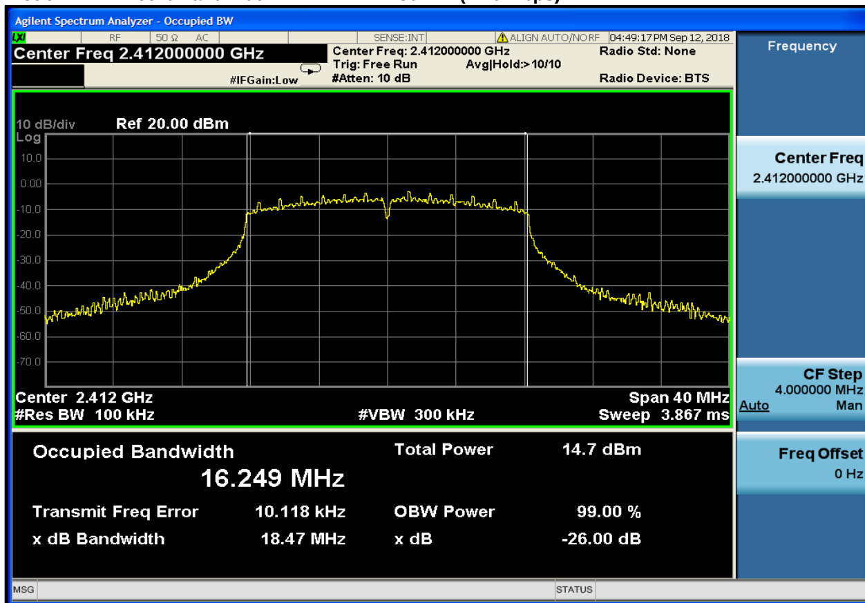
Plot 6-4: 99% Bandwidth – 2412 MHz – 802.11 (11.0 Mbps)
