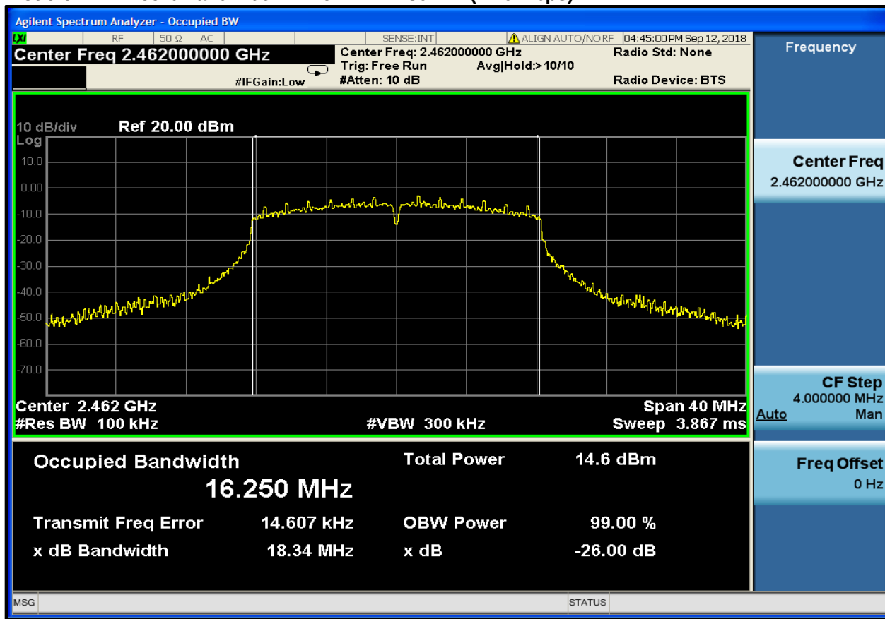
Plot 6-6: 99% Bandwidth – 2462 MHz – 802.11 (11.0 Mbps)
