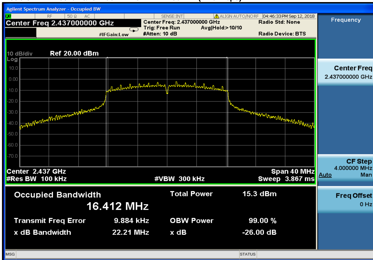
Plot 6-5: 99% Bandwidth – 2437 MHz – 802.11 (11.0 Mbps)
