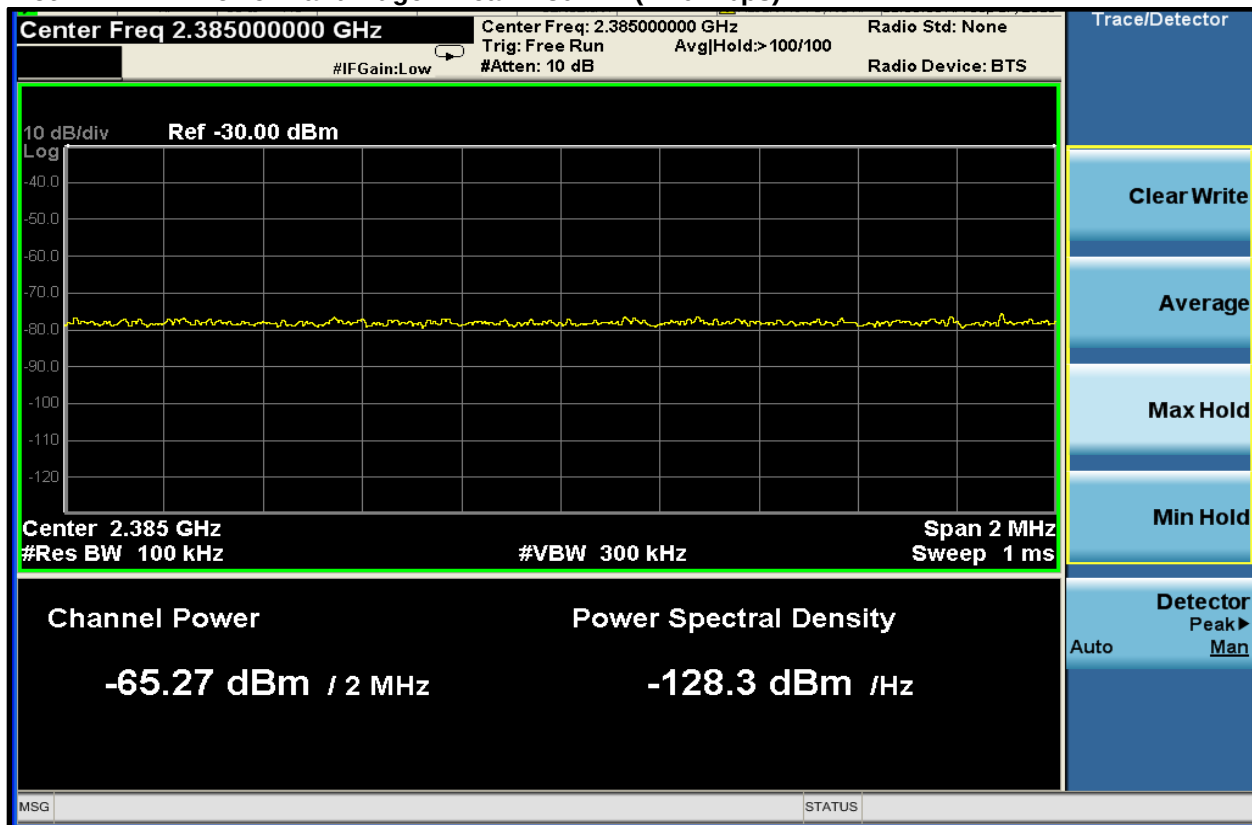
Plot 4-2: Lower Band Edge – Peak – 802.11 (11.0 Mbps)
