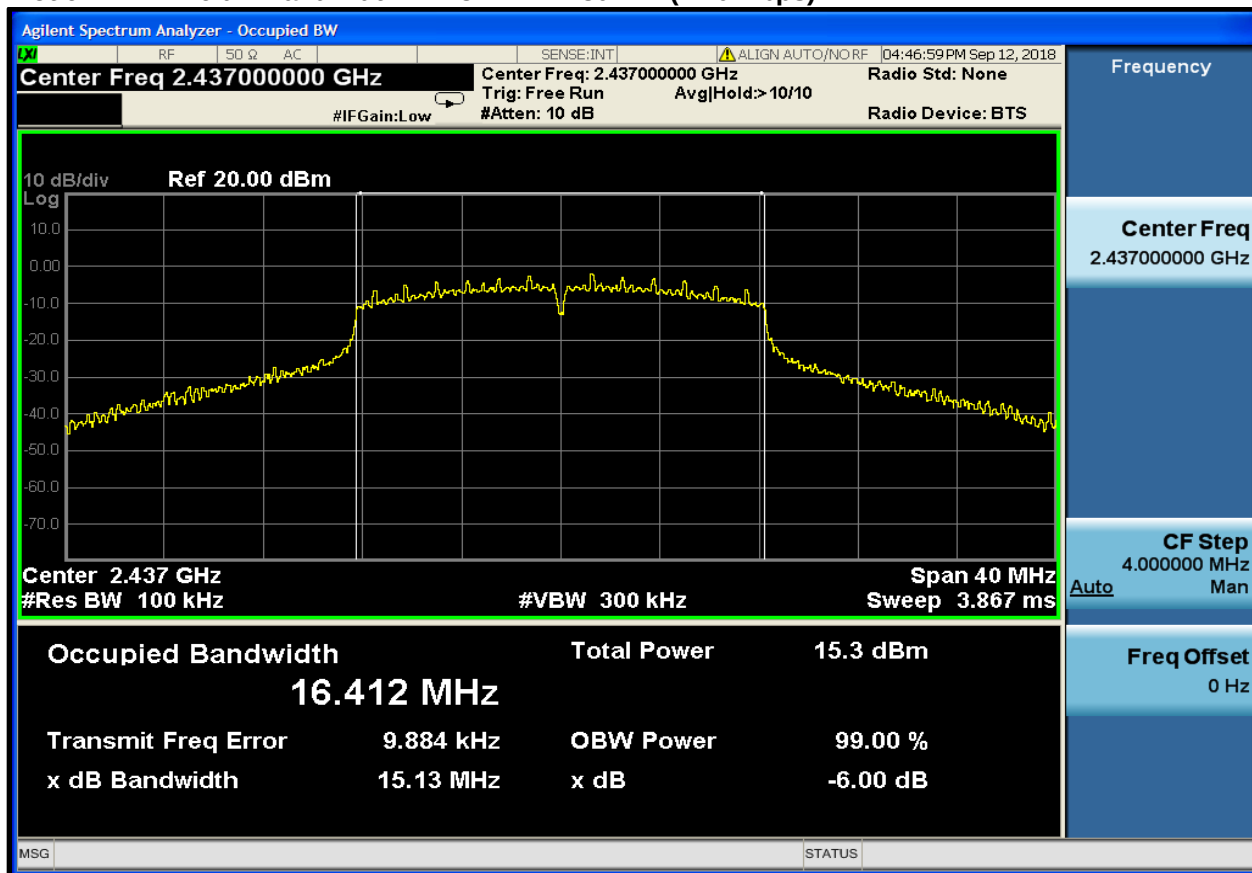
Plot 6-2: 6 dB Bandwidth – 2437 MHz – 802.11 (11.0 Mbps)
