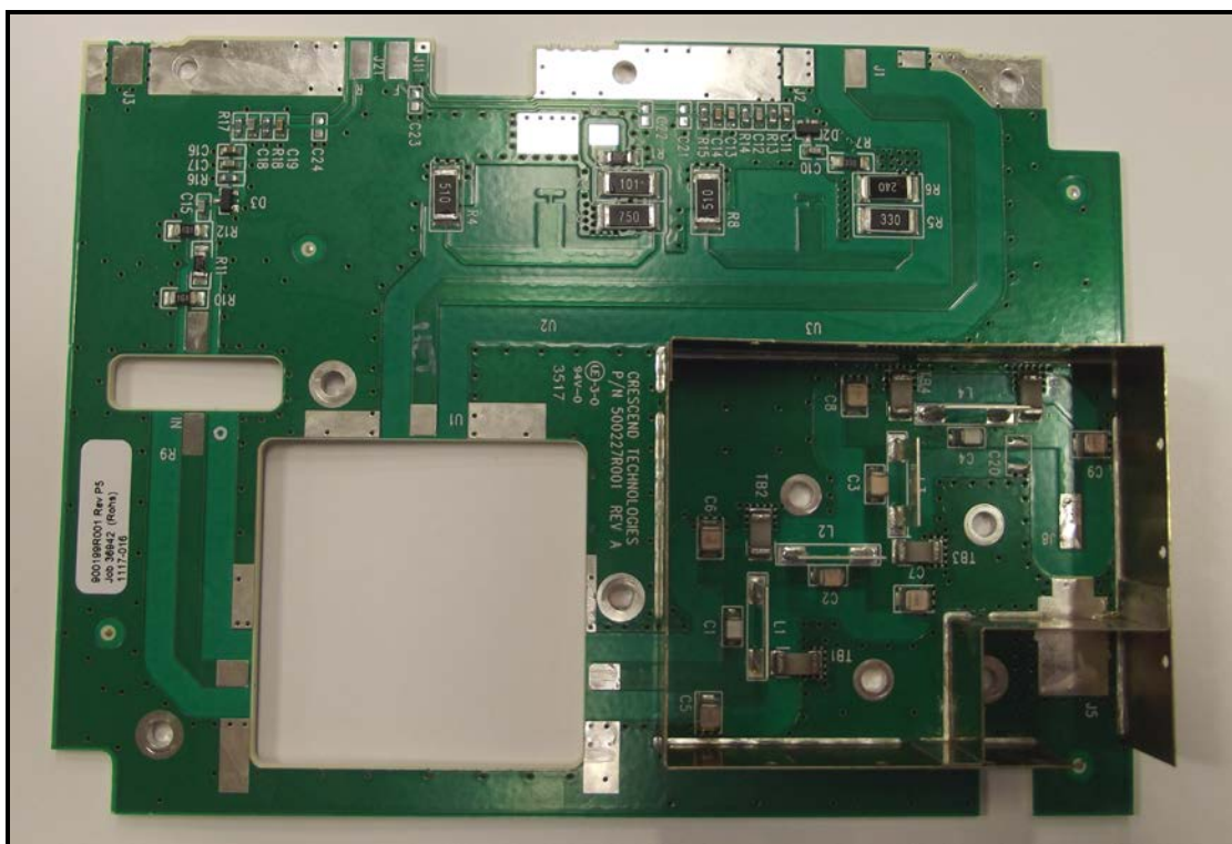
Power Amplifier Output Assembly Top View
