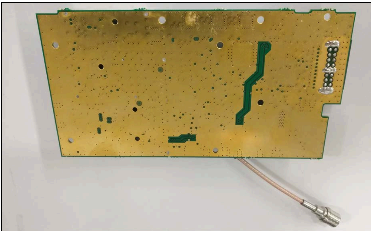
Power Amplifier Driver Assembly Bottom View
