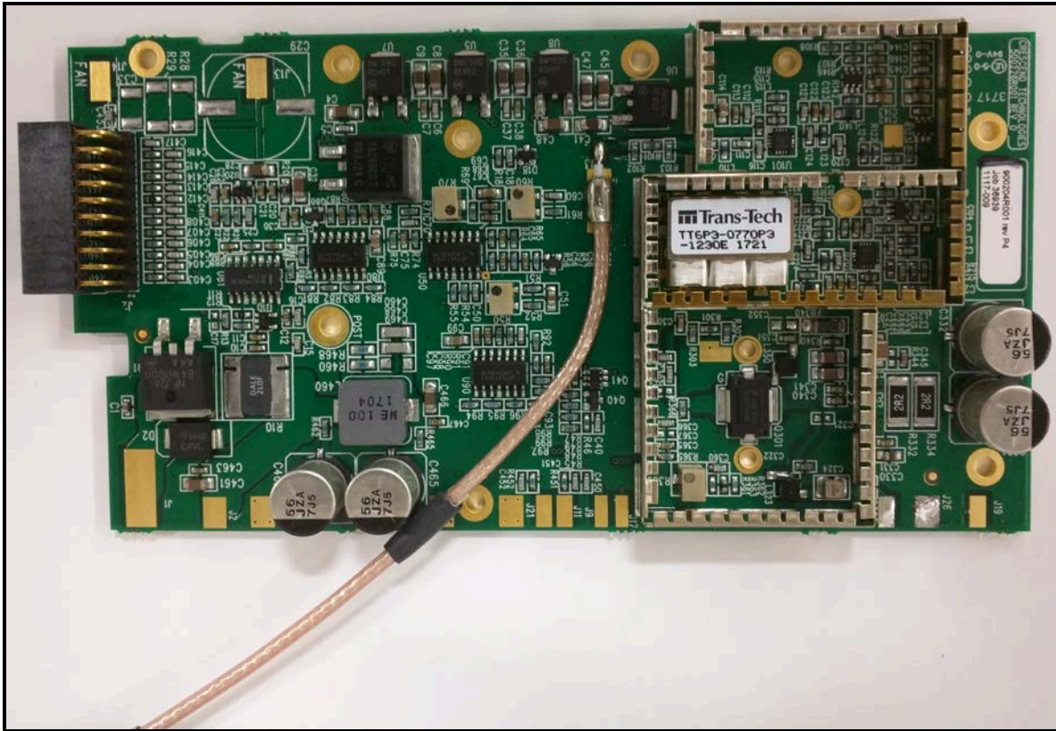
Power Amplifier Driver Assembly Top View
