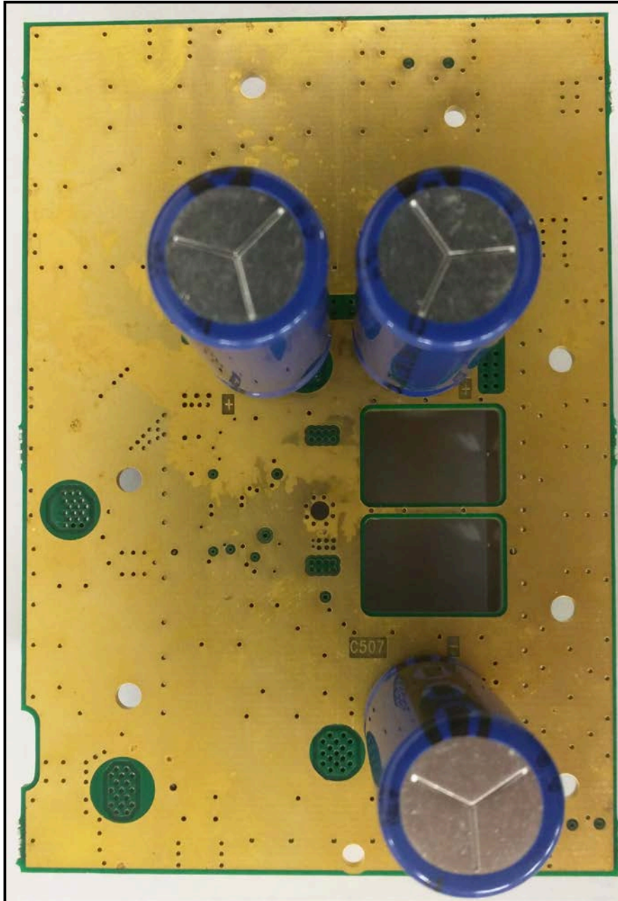
Power Amplifier Switcher Assembly Bottom View
