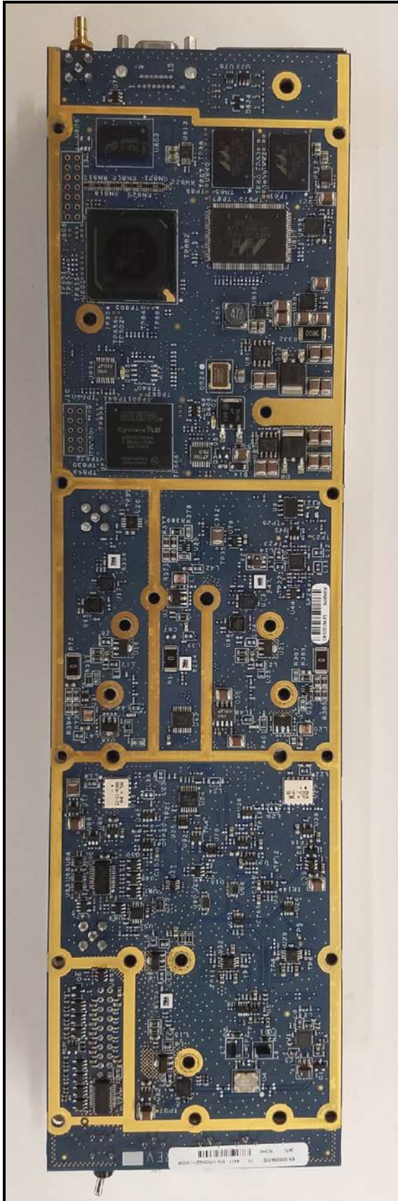
Linearizer Module Top View
