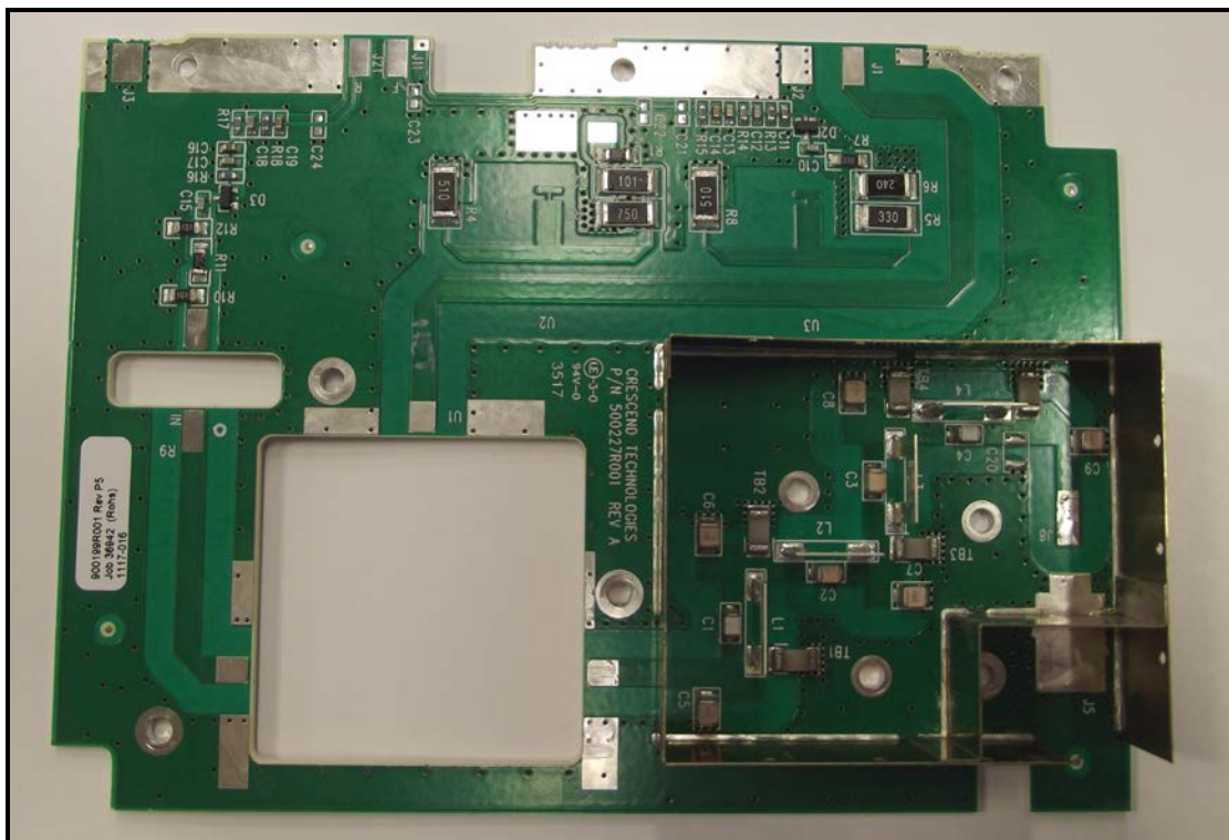
Power Amplifier Output Assembly Top View
