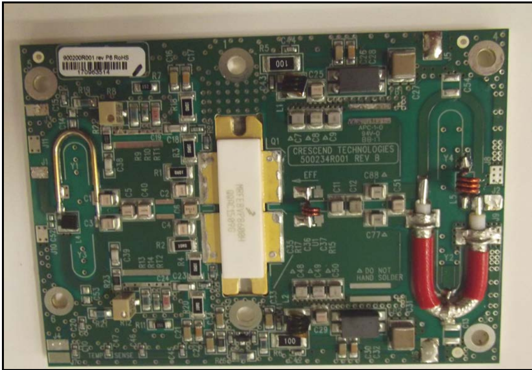
Power Amplifier Final Assembly Top View
