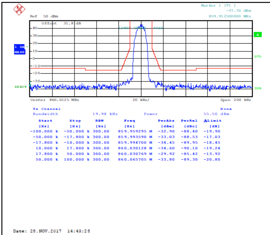
Plot 7-6: Occupied Bandwidth – 860.0125 MHz; WCQPSK; Mask G
