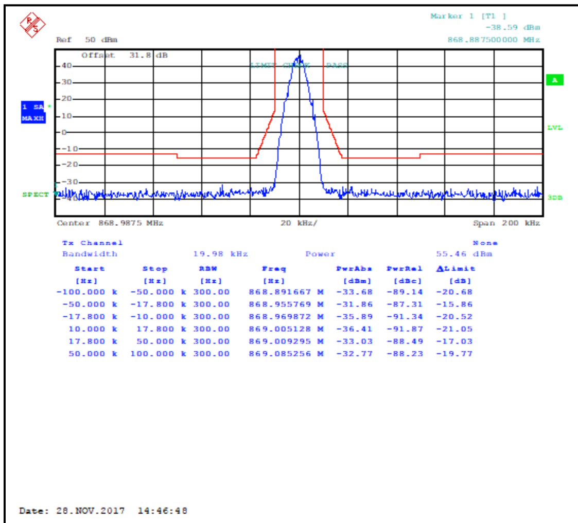
Plot 7-4: Occupied Bandwidth – 868.9875 MHz; C4FM; Mask G
