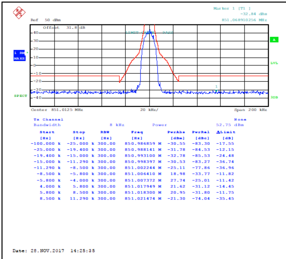
Plot 7-9: Occupied Bandwidth – 851.0125 MHz; HDQPSK; Mask H
