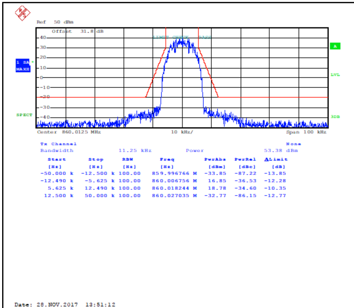
Plot 7-22: Occupied Bandwidth – 860.0125 MHz; HDQPSK; Mask D
