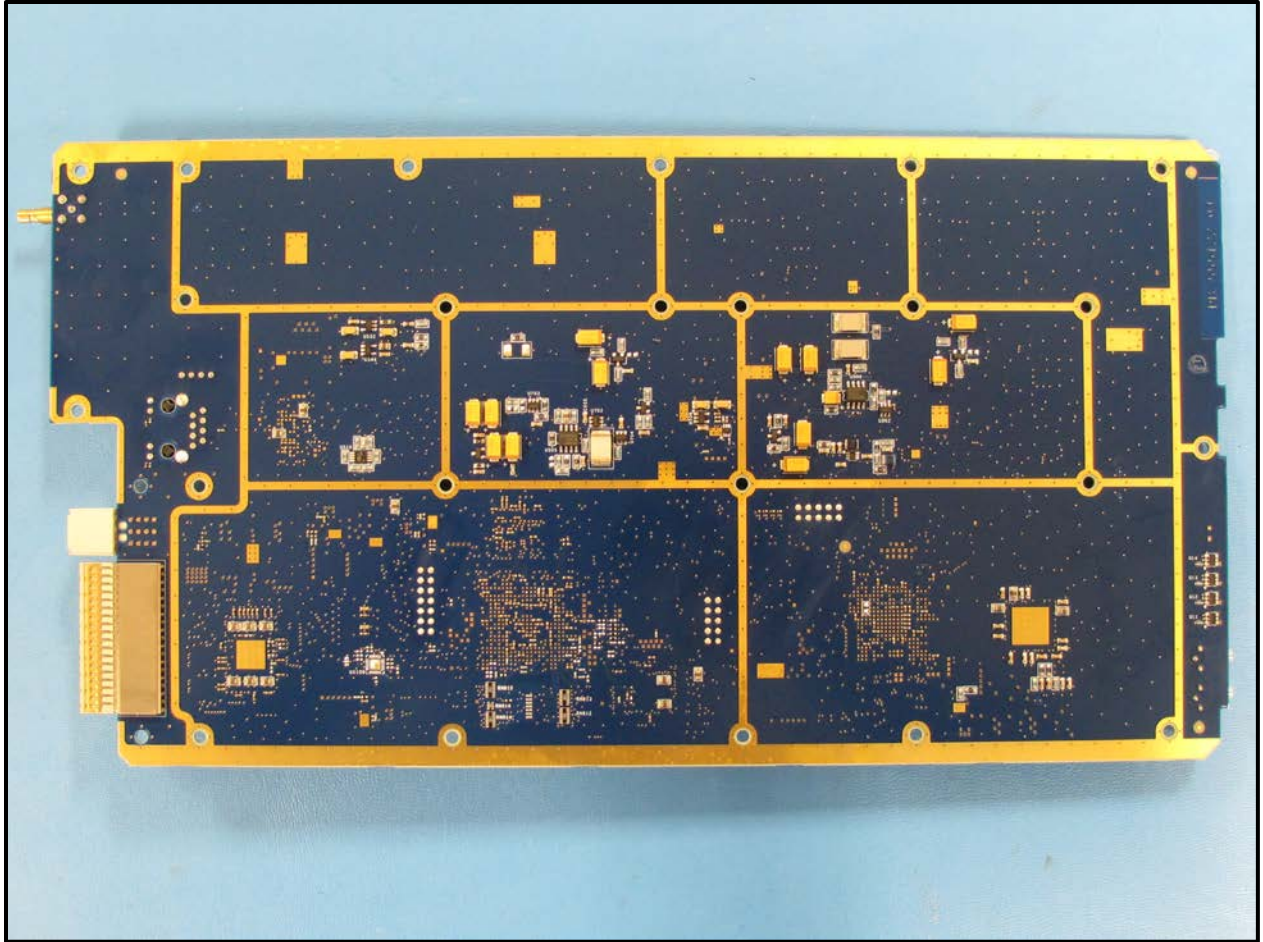
TX Module PCB Bottom View
