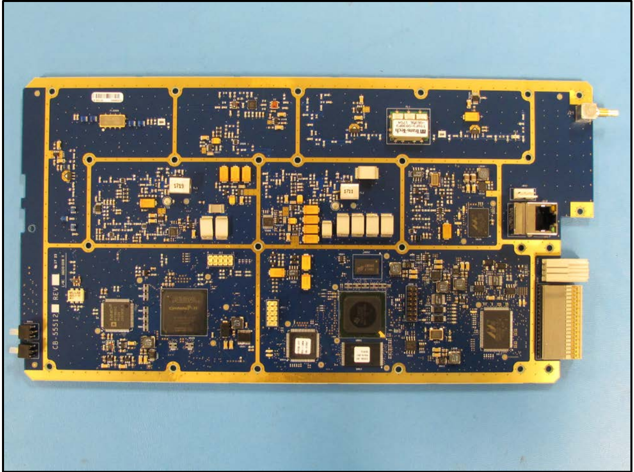
TX Module PCB Top View
