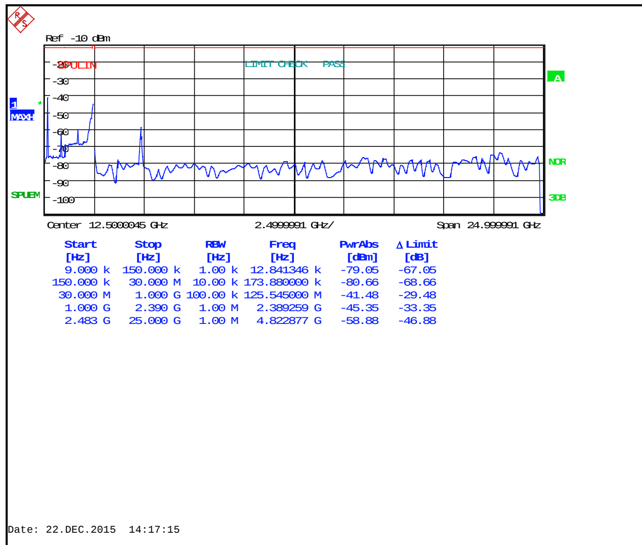
Plot 5-2: Antenna Conducted Spurious Emissions – 2440 MHz
