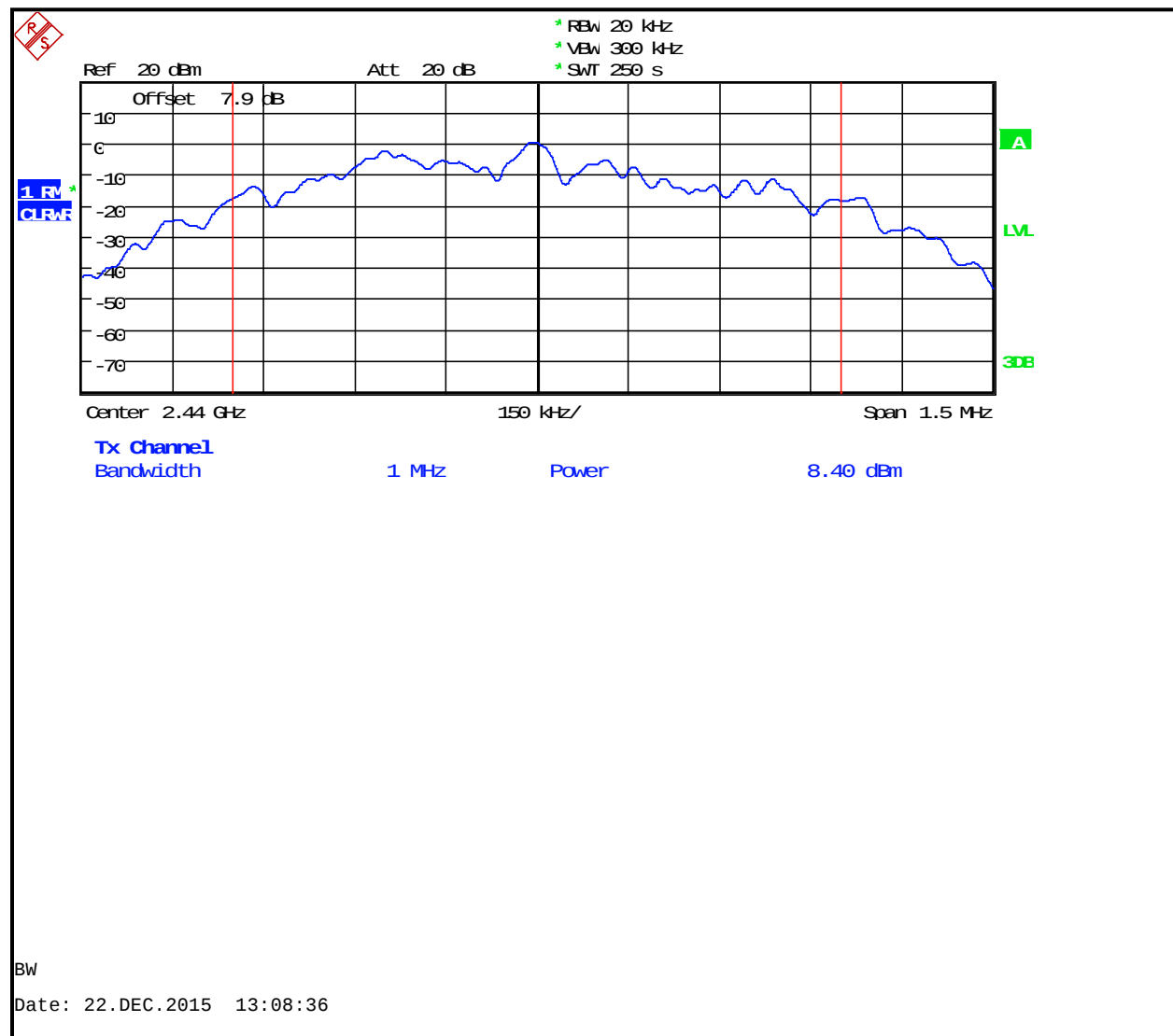
Plot 3-2: Peak Output Power – 2440 MHz
