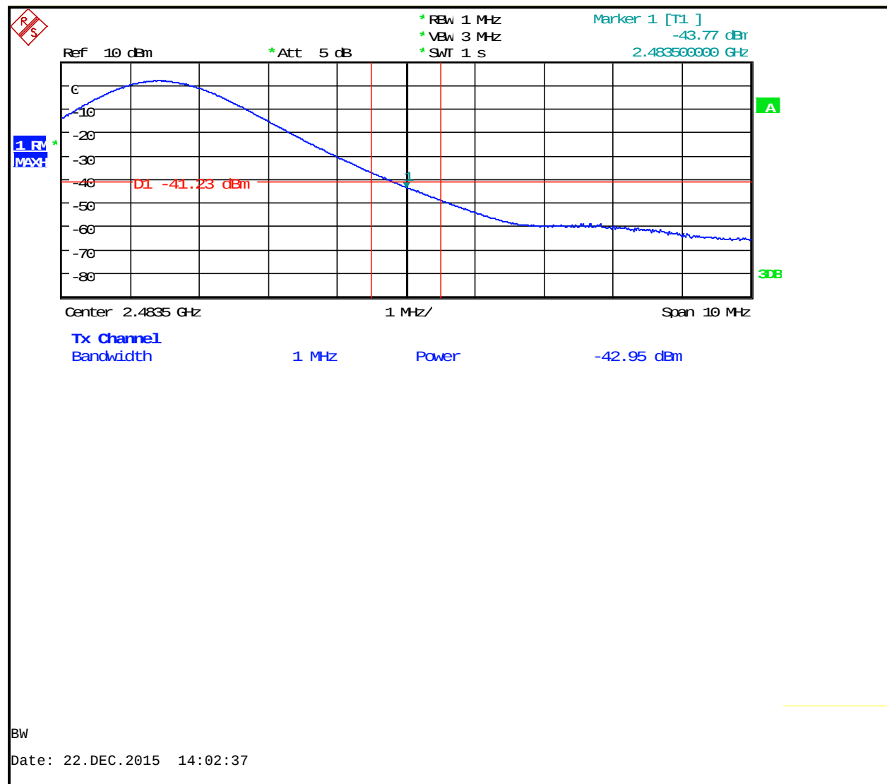
Plot 6-4: Upper Band Edge - Average
