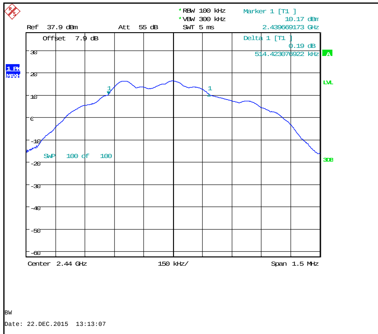
Plot 7-2: 6 dB Bandwidth – 2440 MHz
