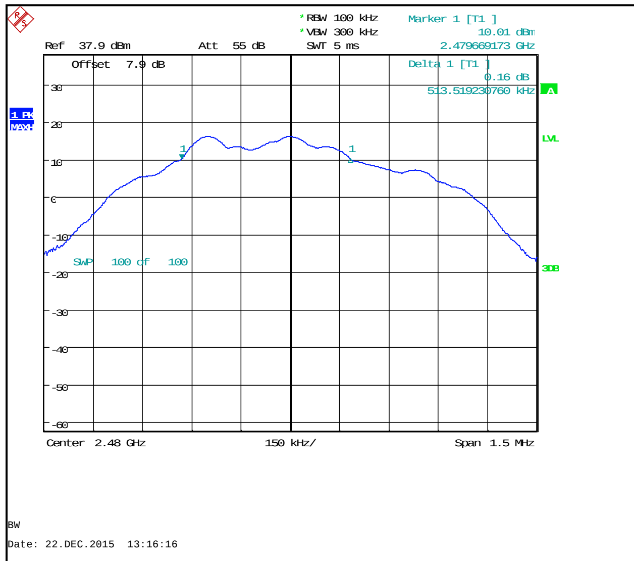
Plot 7-3: 6 dB Bandwidth – 2480 MHz
