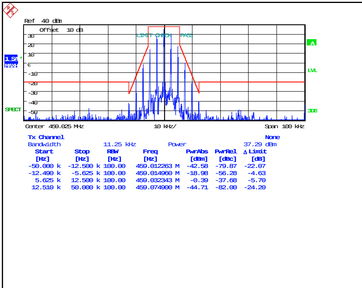
Plot 7-12: Occupied Bandwidth – 459.025 MHz; Narrowband Analog; Mask D
