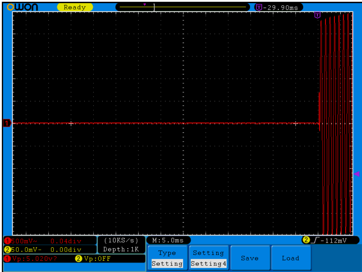
Plot 10-4: Transient Frequency Behavior – 512 MHz; High Power; Wideband; Carrier OFF Time
