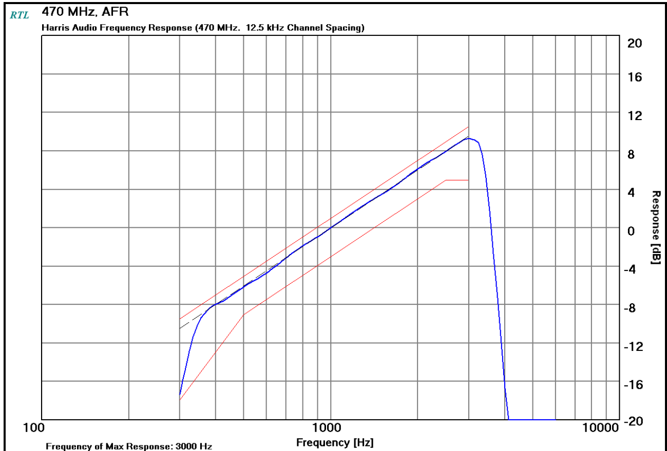
Plot 9-2: Modulation Characteristics - Audio Frequency Response - 470 MHz
