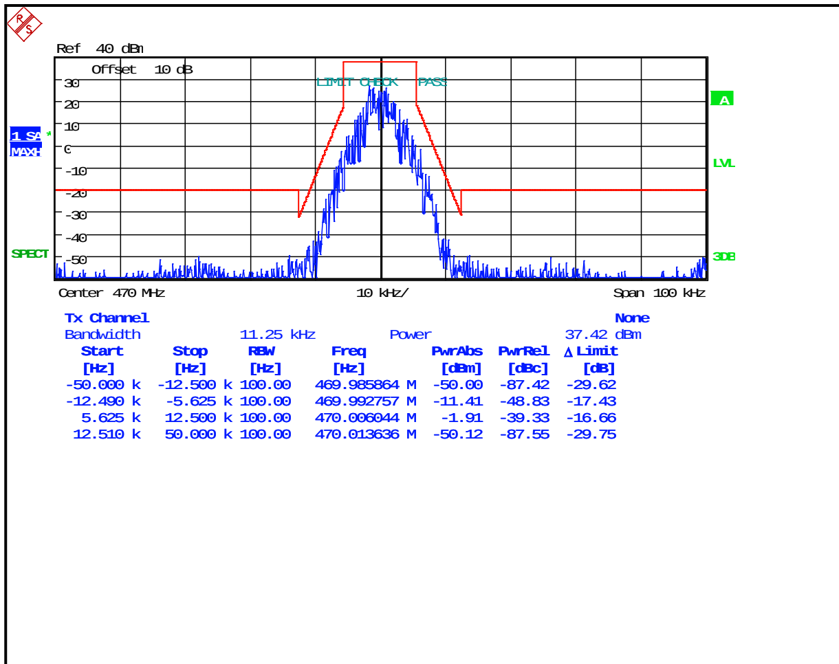
Plot 7-21: Occupied Bandwidth – 470 MHz; P25; Mask D
