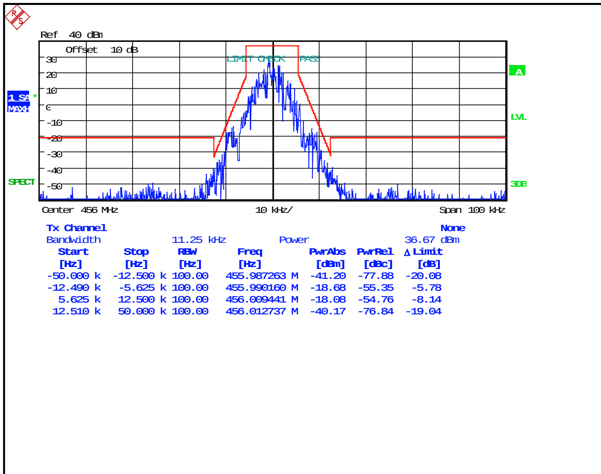
Plot 7-32: Occupied Bandwidth – 456 MHz; (2-level FSK 9600; NB) EDACS; Mask D
