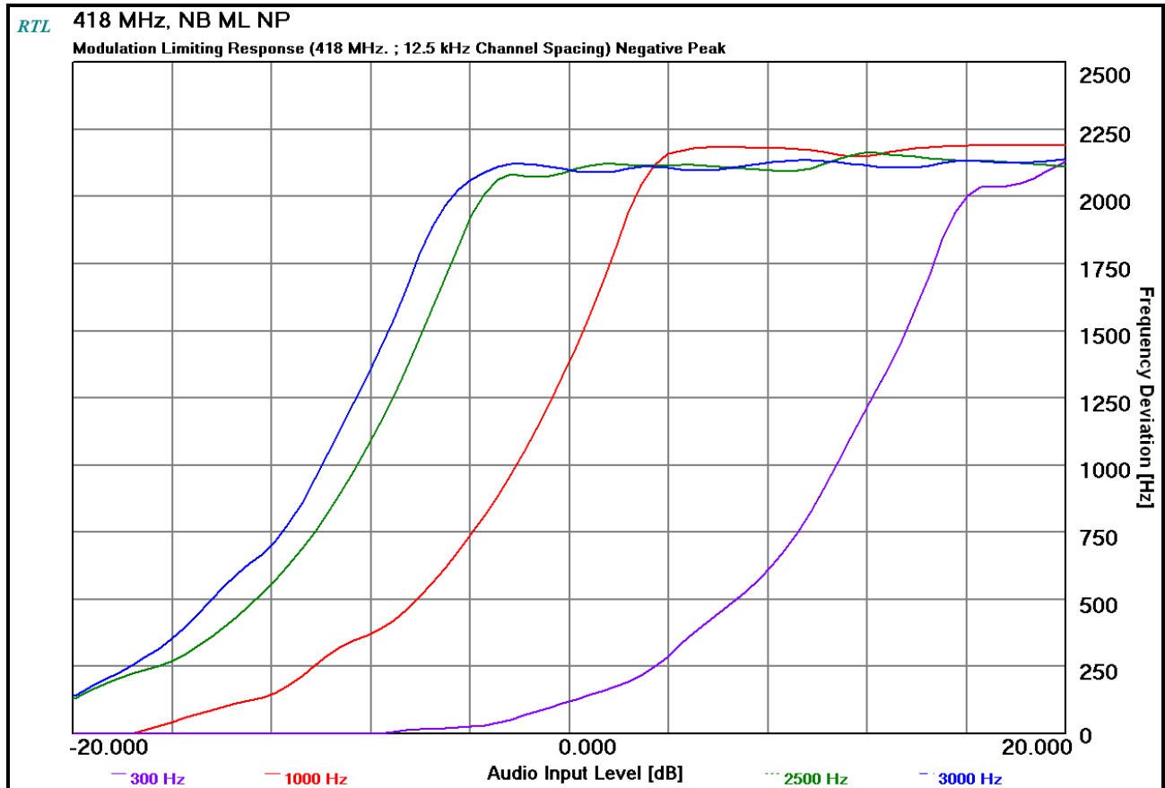
Plot 9-9: Modulation Characteristics – Modulation Limiting - 418 MHz; Negative Peak; NB
