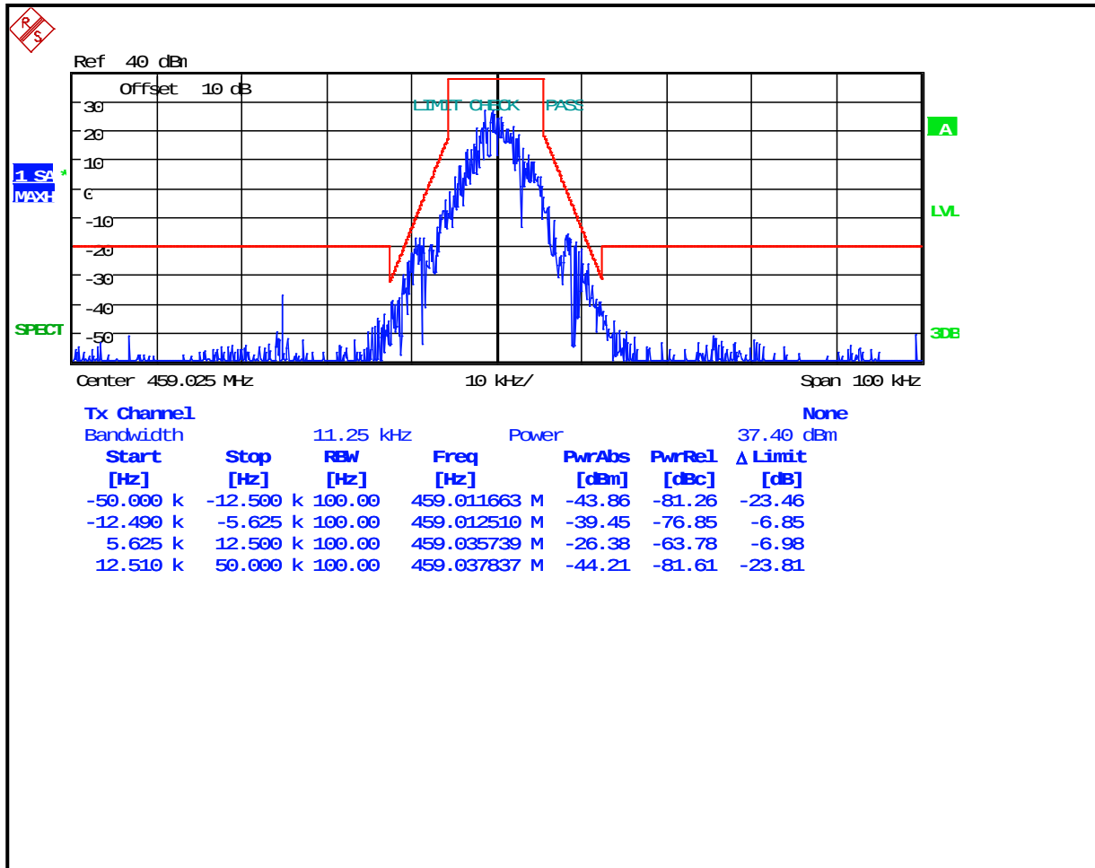
Plot 7-33: Occupied Bandwidth – 459.025 MHz; (2-level FSK 9600; NB) EDACS; Mask D
