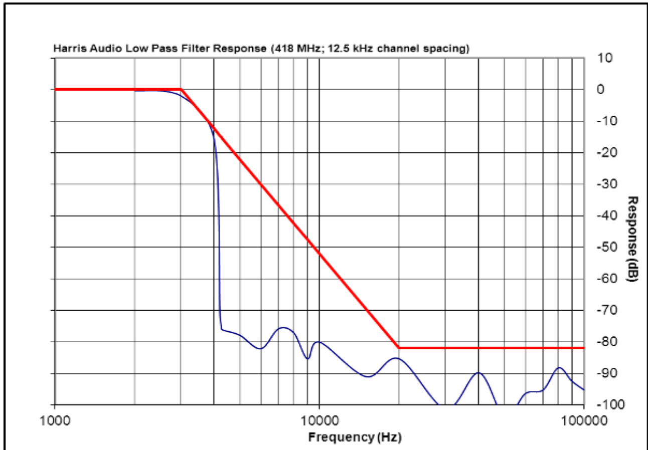
Plot 9-5: Modulation Characteristics – Audio Low Pass Filter - 418 MHz (NB)
