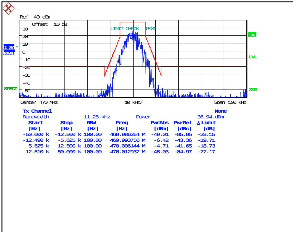
Plot 7-28: Occupied Bandwidth – 470 MHz; CPM TDMA; Mask D
