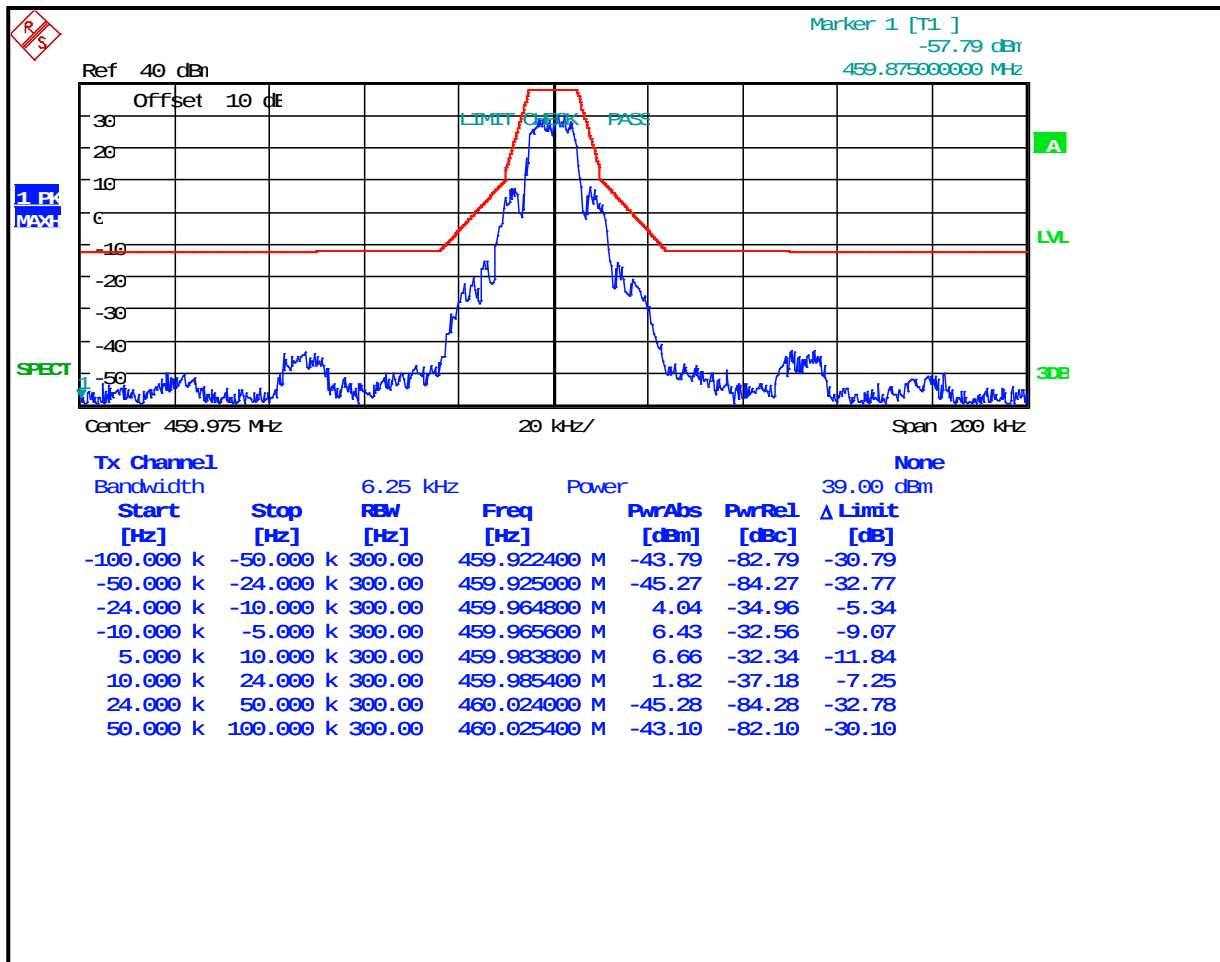
Plot 7-41: Occupied Bandwidth – 459.975MHz; (2-level FSK 9600; WB) EDACS; Mask C
