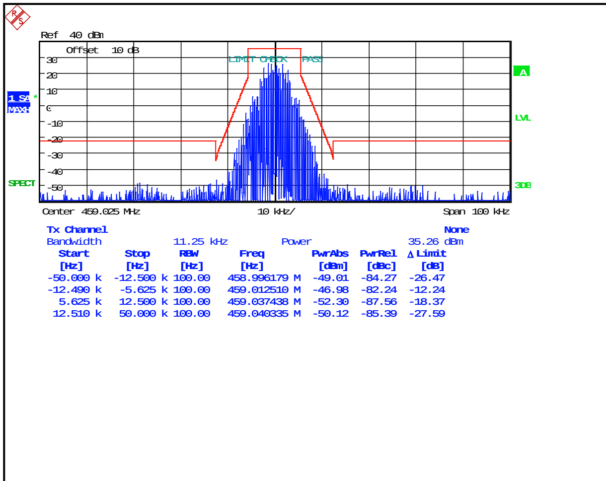
Plot 7-26: Occupied Bandwidth – 459.025 MHz; CPM TDMA; Mask D
