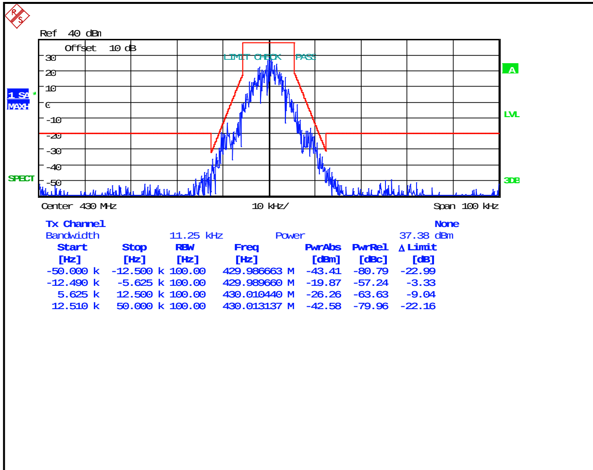
Plot 7-29: Occupied Bandwidth – 430 MHz; (2-level FSK 9600; NB) EDACS; Mask D
