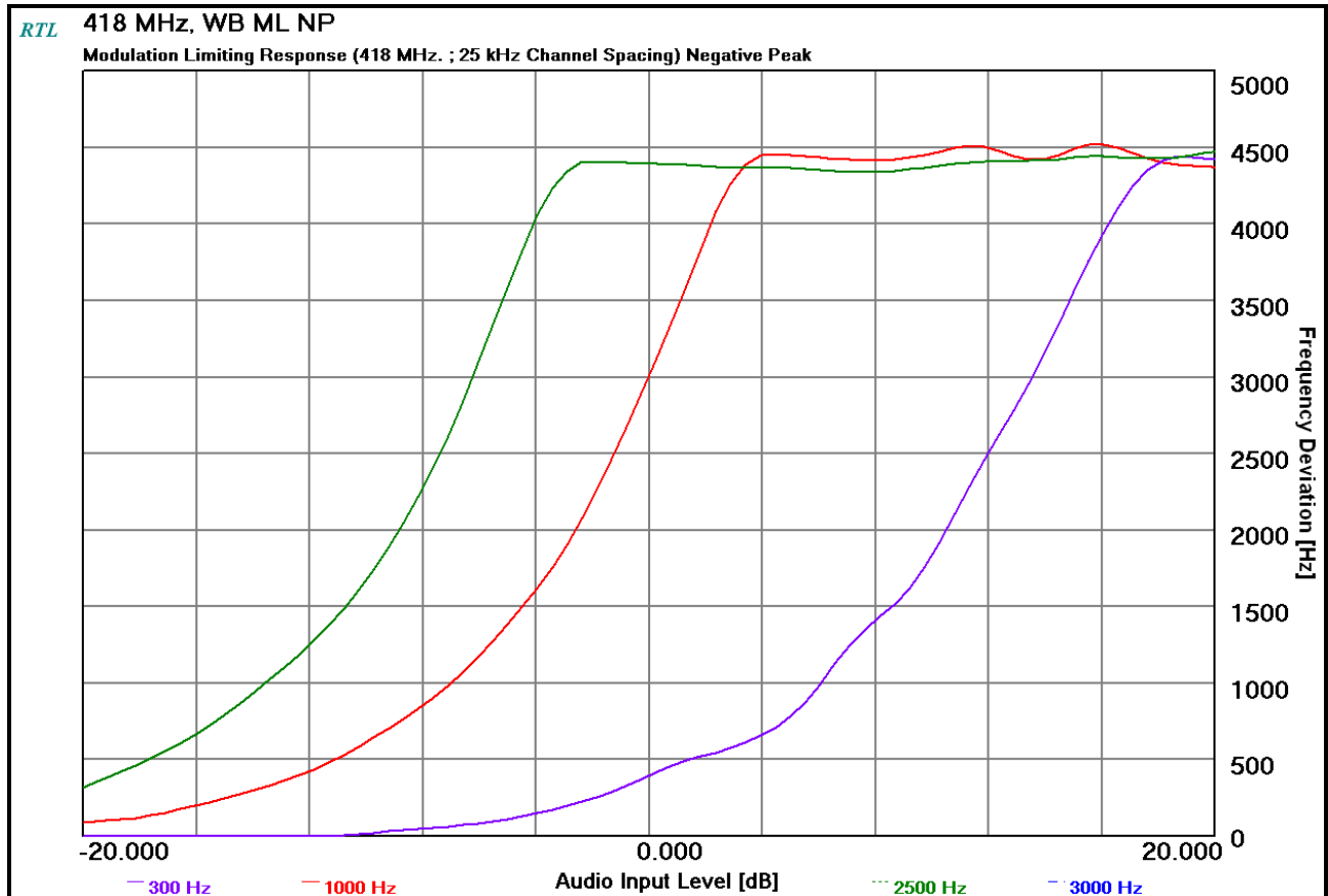
Plot 9-11: Modulation Characteristics – Modulation Limiting - 418 MHz; Negative Peak; WB
