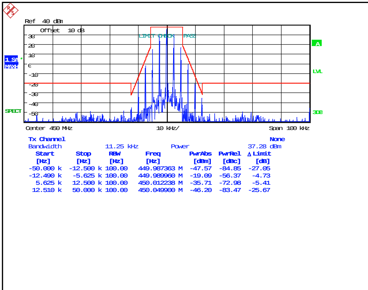
Plot 7-9: Occupied Bandwidth – 450 MHz; Narrowband Analog; Mask D
