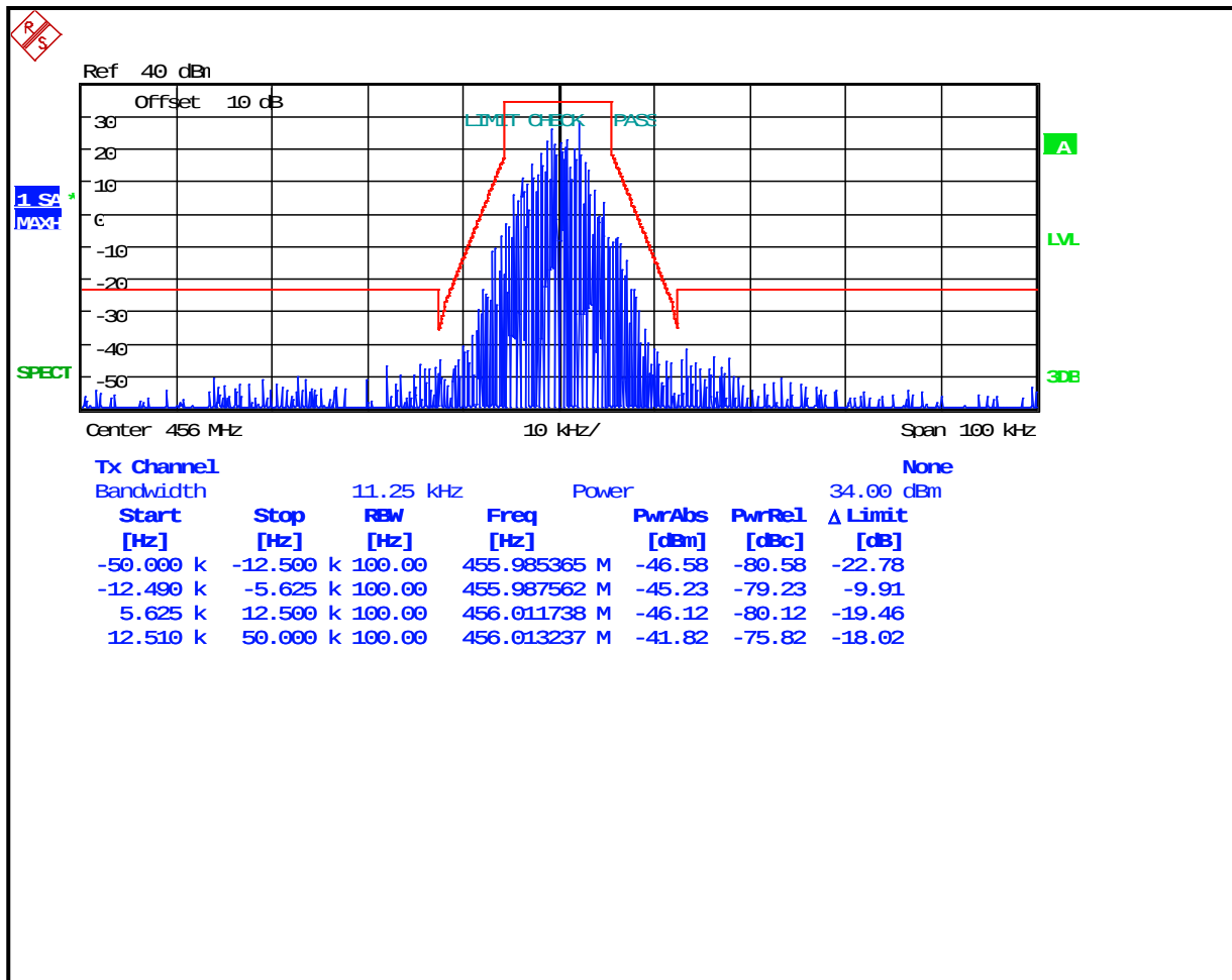
Plot 7-25: Occupied Bandwidth – 456 MHz; CPM TDMA; Mask D
