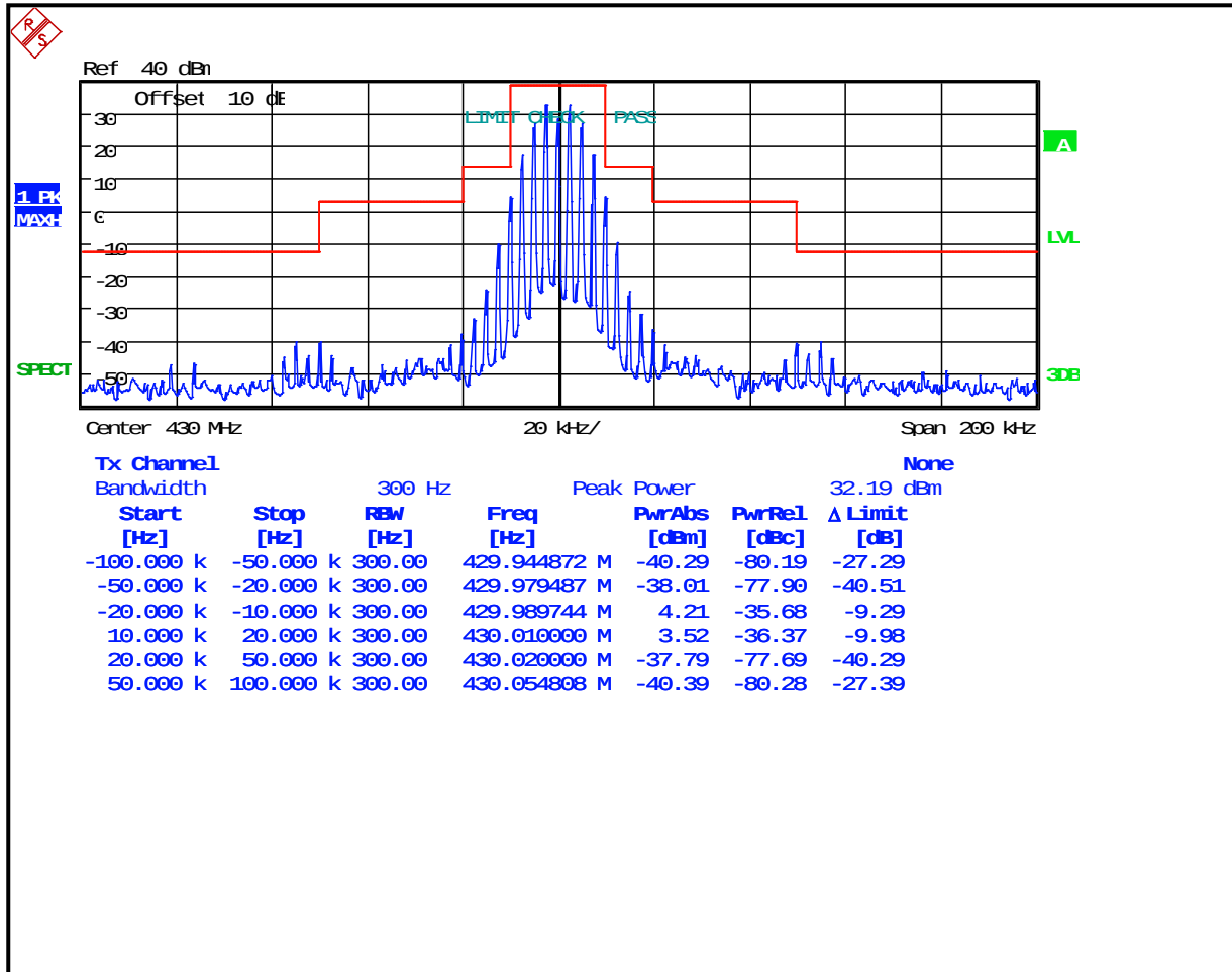
Plot 7-1: Occupied Bandwidth – 430 MHz; Wideband Analog; Mask B
