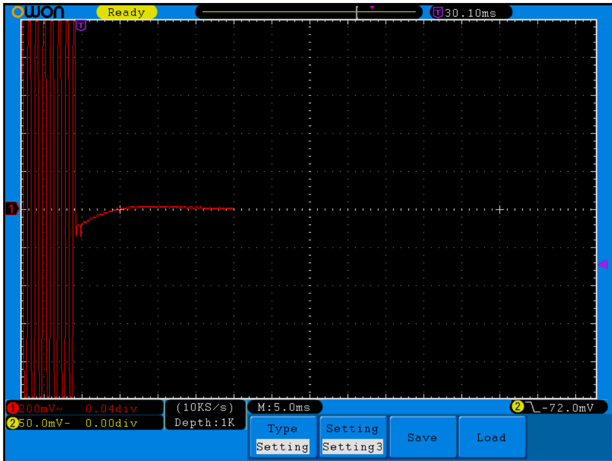
Plot 10-3: Transient Frequency Behavior – 512 MHz; High Power; Wideband; Carrier ON Time
