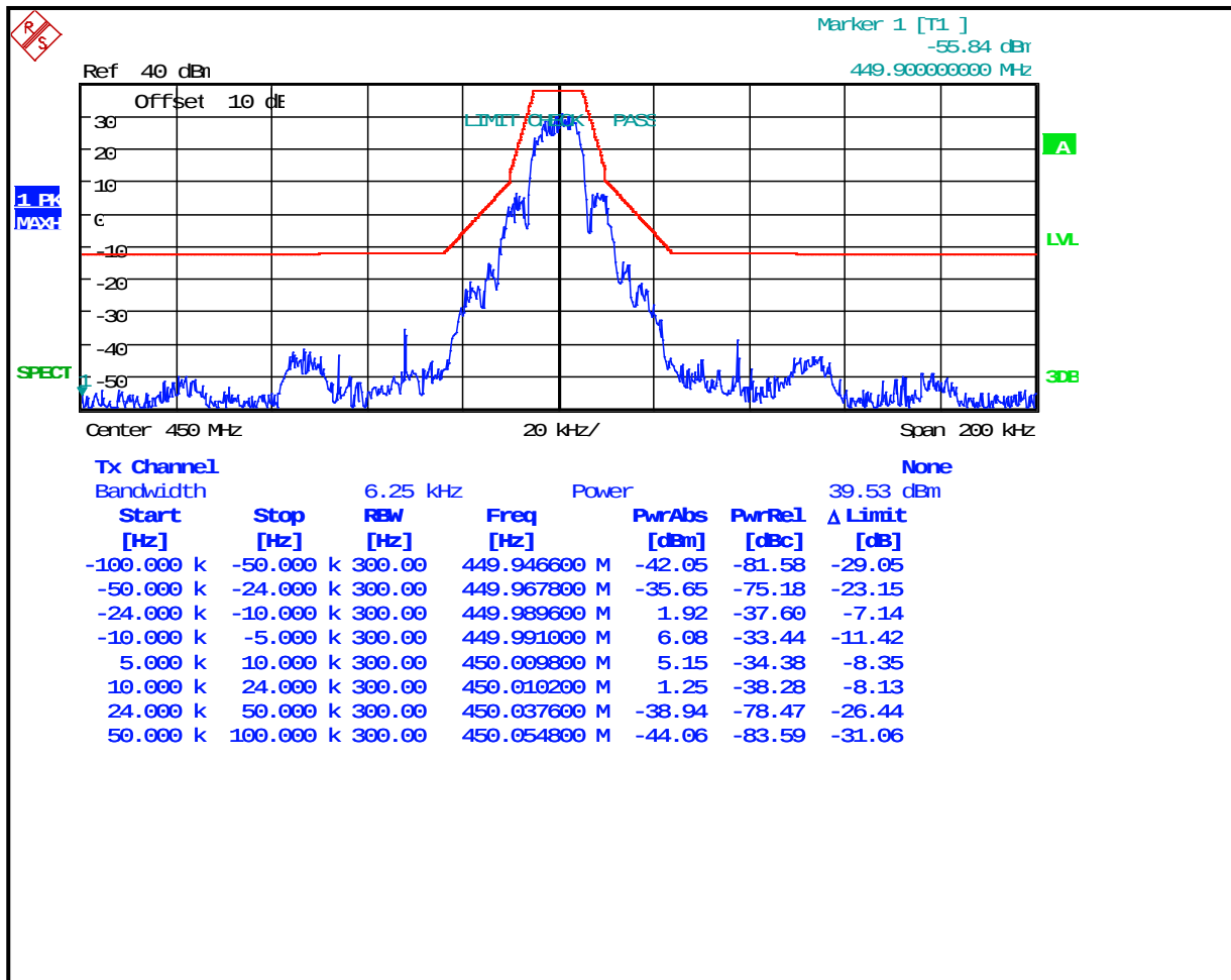
Plot 7-37: Occupied Bandwidth – 450 MHz; (2-level FSK 9600; WB) EDACS; Mask C
