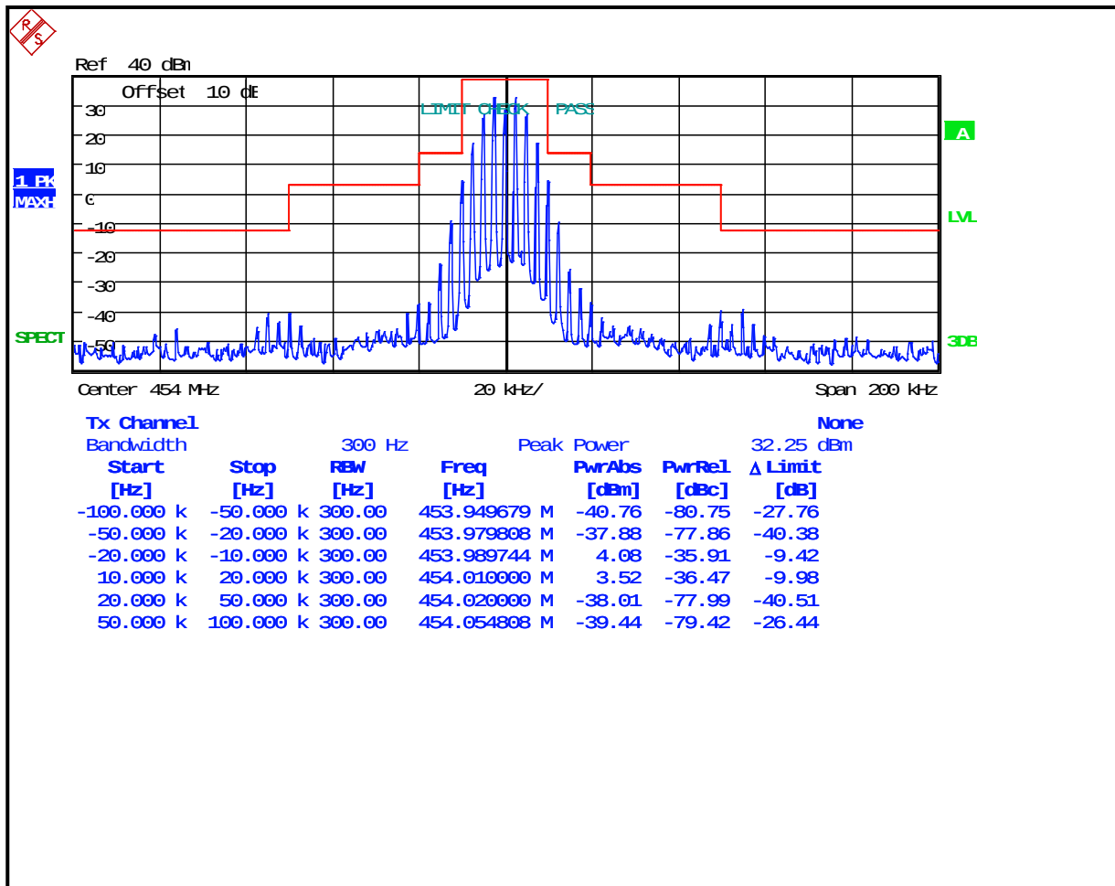
Plot 7-3: Occupied Bandwidth – 454 MHz; Wideband Analog; Mask B
