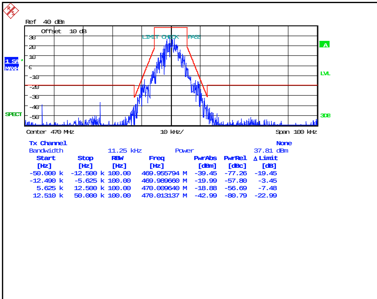
Plot 7-35: Occupied Bandwidth – 470 MHz; (2-level FSK 9600; NB) EDACS; Mask D
