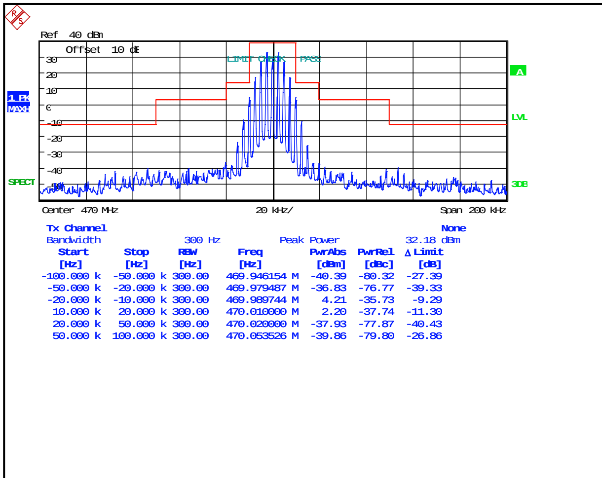
Plot 7-7: Occupied Bandwidth – 470 MHz; Wideband Analog; Mask B
