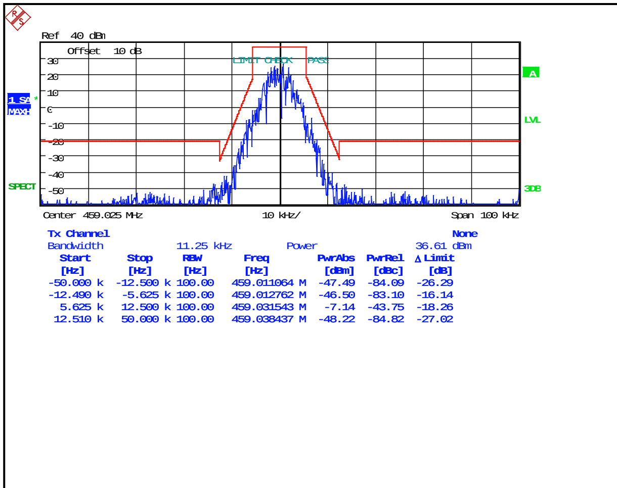
Plot 7-47: Occupied Bandwidth – 459.025 MHz; (4-level FSK Data/Voice; NB) OpenSky; Mask D
