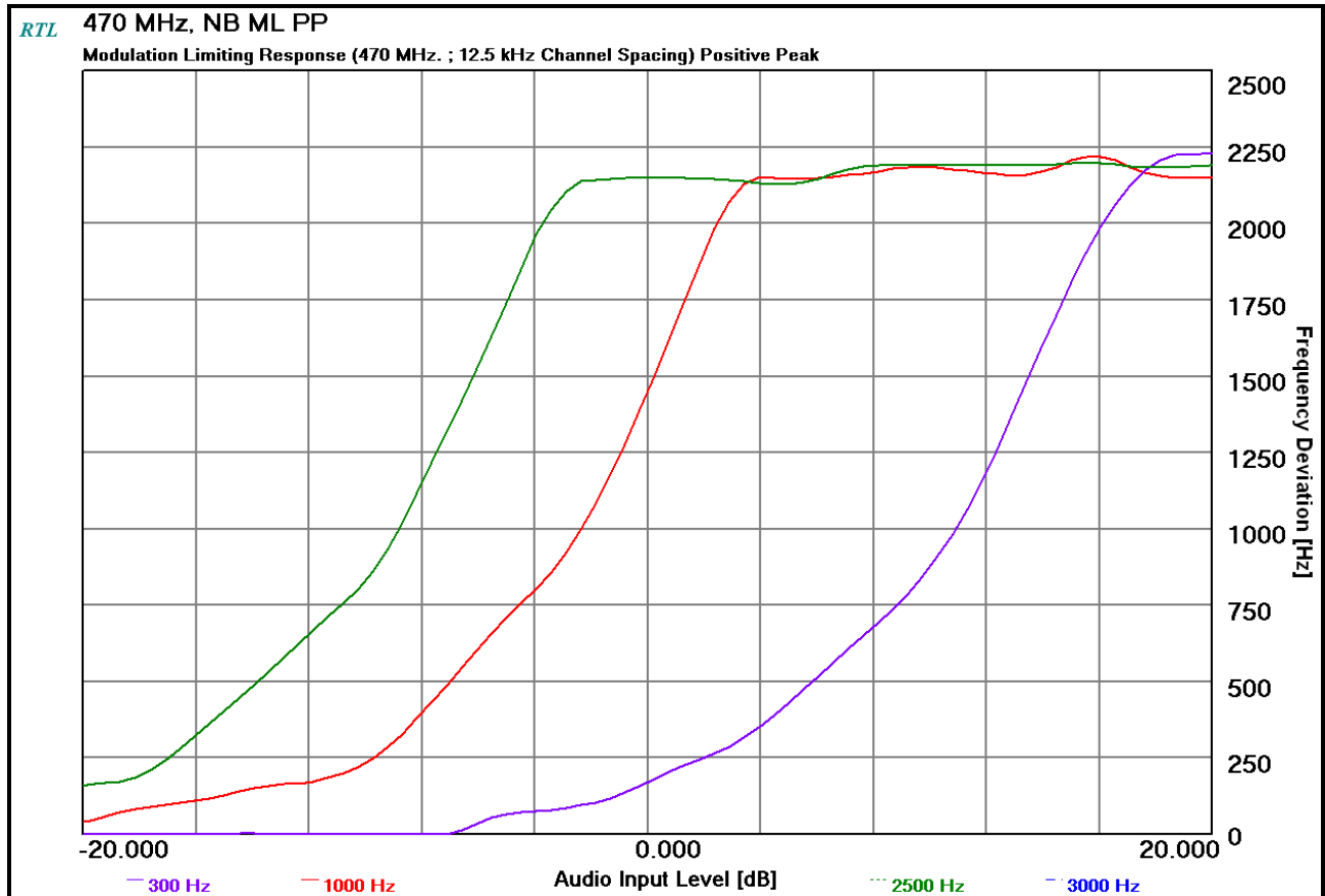
Plot 9-12: Modulation Characteristics – Modulation Limiting - 470 MHz; Positive Peak; NB
