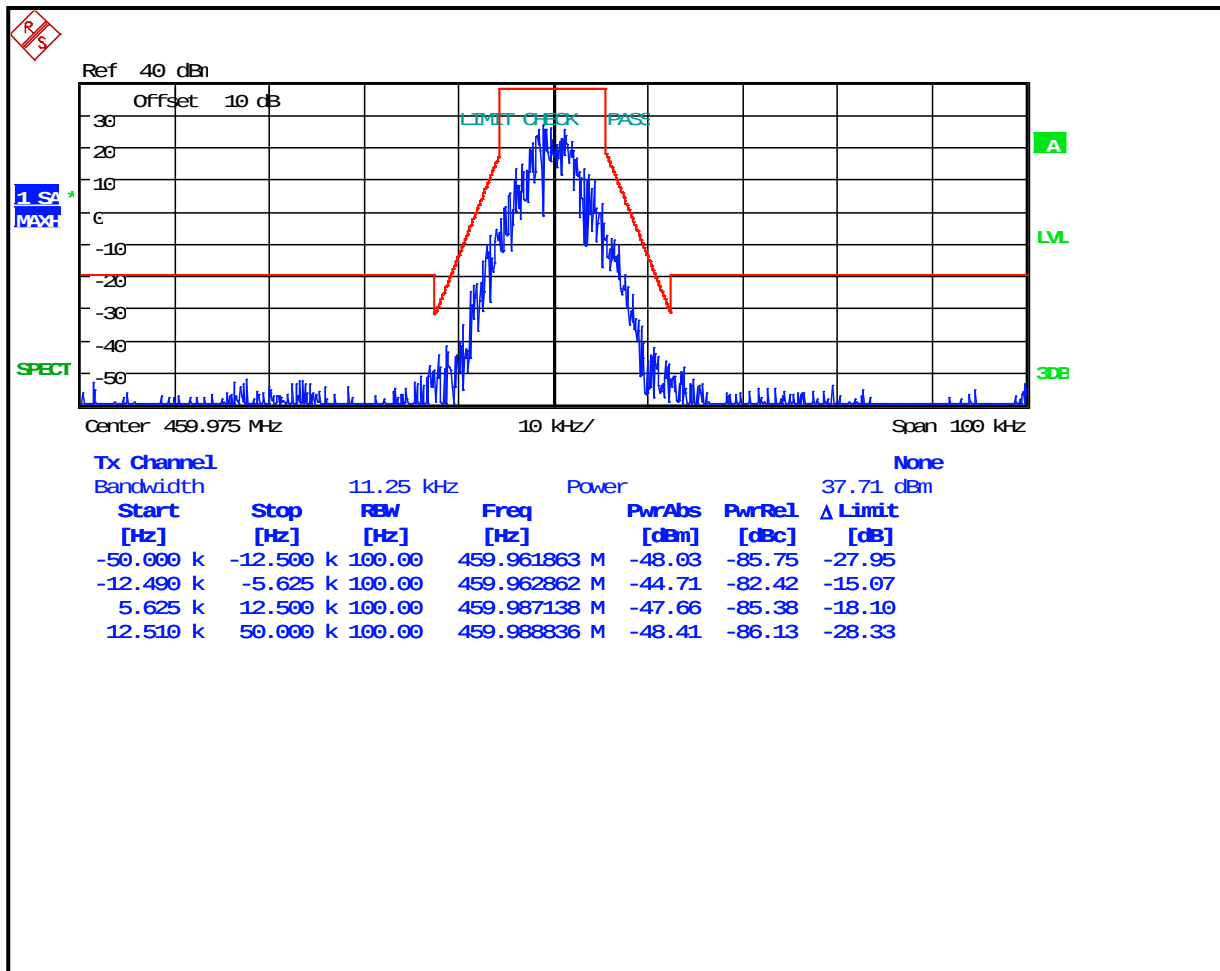
Plot 7-48: Occupied Bandwidth – 459.975MHz; (4-level FSK Data/Voice; NB) OpenSky; Mask D
