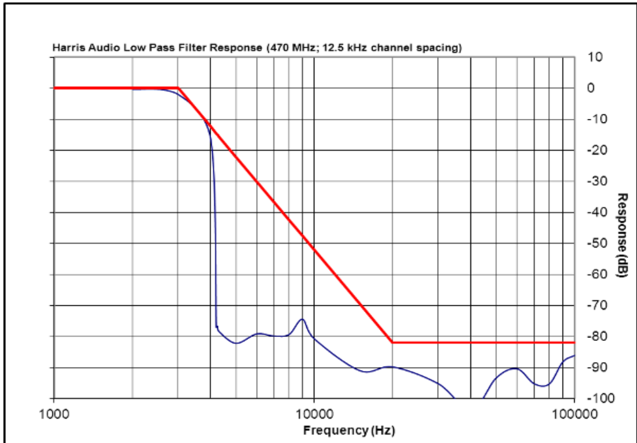
Plot 9-7: Modulation Characteristics – Audio Low Pass Filter - 470 MHz (NB)
