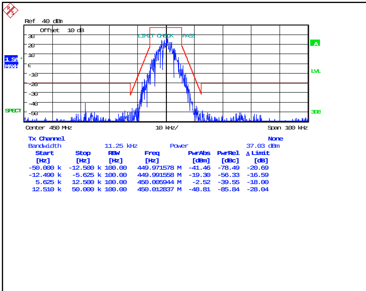
Plot 7-44: Occupied Bandwidth – 450 MHz; (4-level FSK Data/Voice; NB) OpenSky; Mask D
