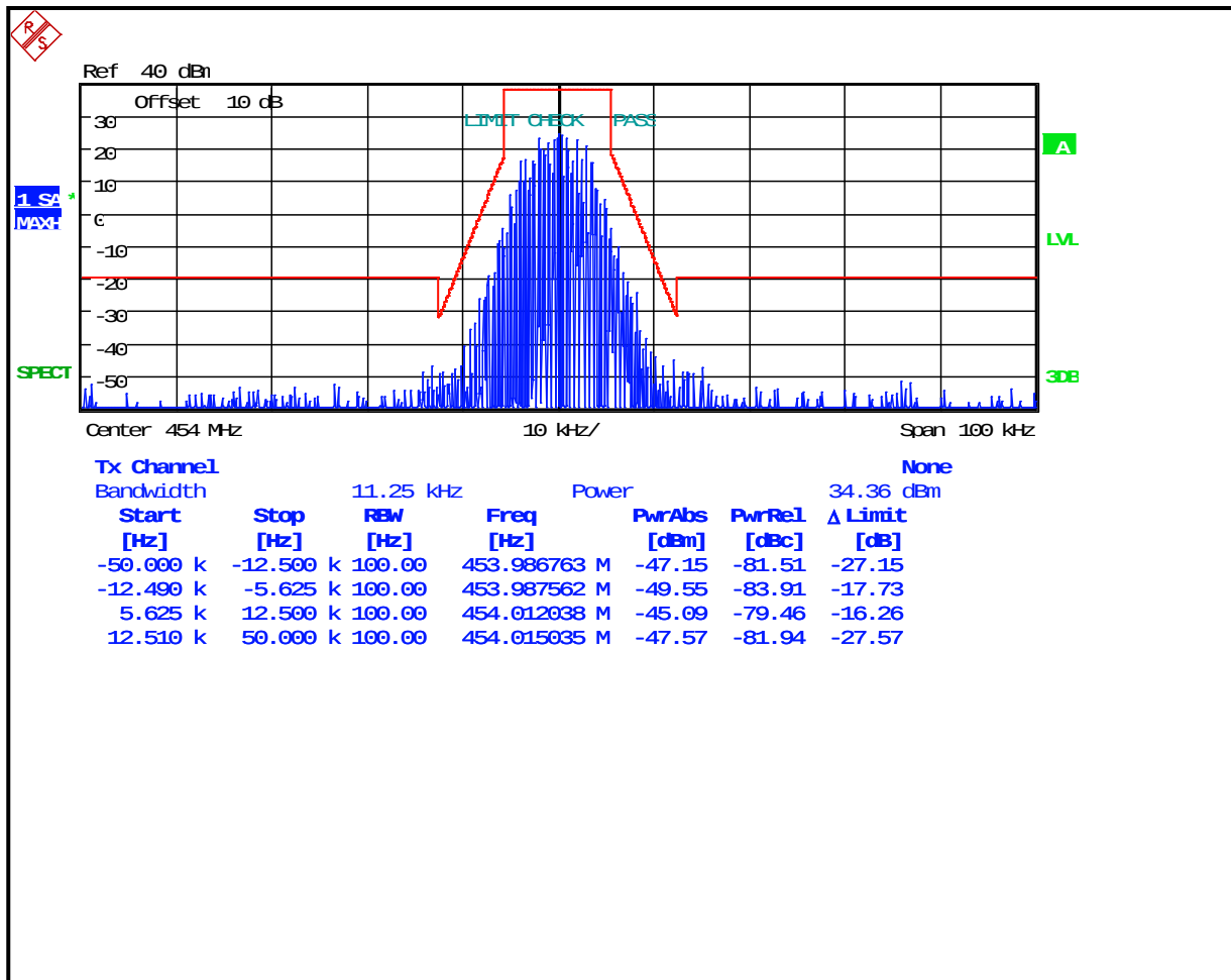
Plot 7-24: Occupied Bandwidth – 454 MHz; CPM TDMA; Mask D
