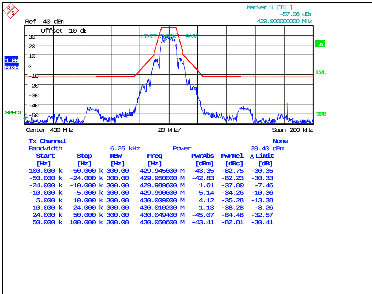
Plot 7-36: Occupied Bandwidth – 430 MHz; (2-level FSK 9600; WB) EDACS; Mask C
