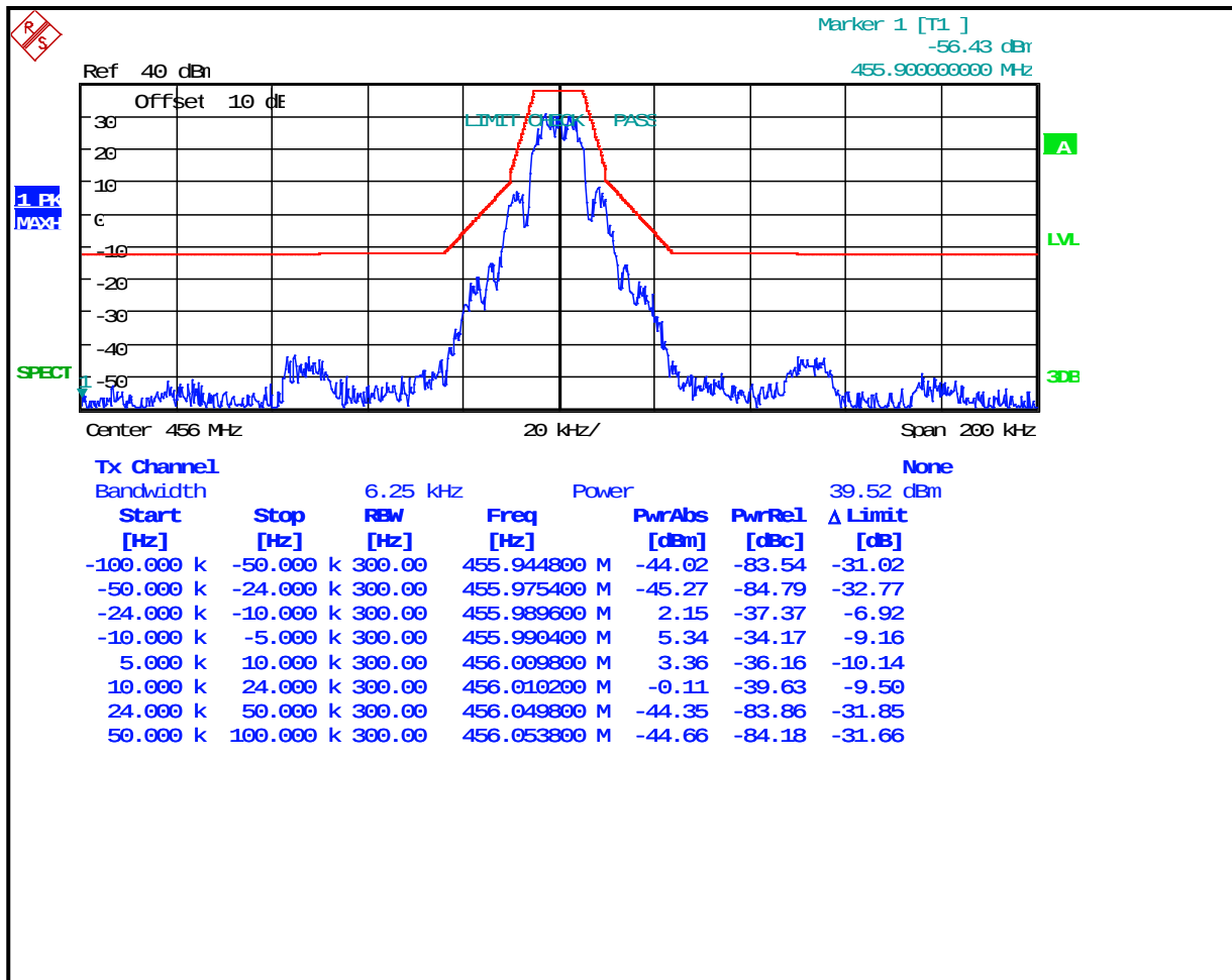
Plot 7-39: Occupied Bandwidth – 456 MHz; (2-level FSK 9600; WB) EDACS; Mask C
