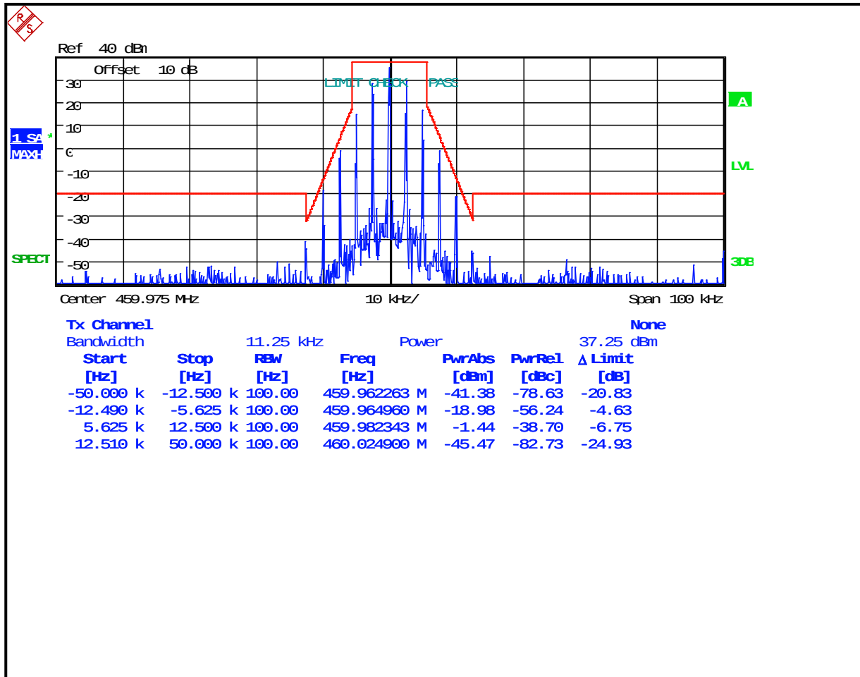
Plot 7-13: Occupied Bandwidth – 459.975 MHz; Narrowband Analog; Mask D
