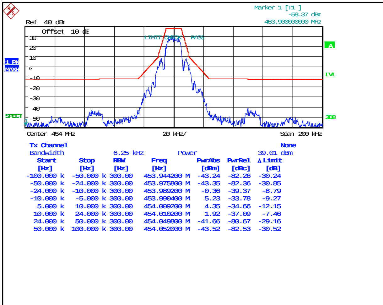
Plot 7-38: Occupied Bandwidth – 454 MHz; (2-level FSK 9600; WB) EDACS; Mask C
