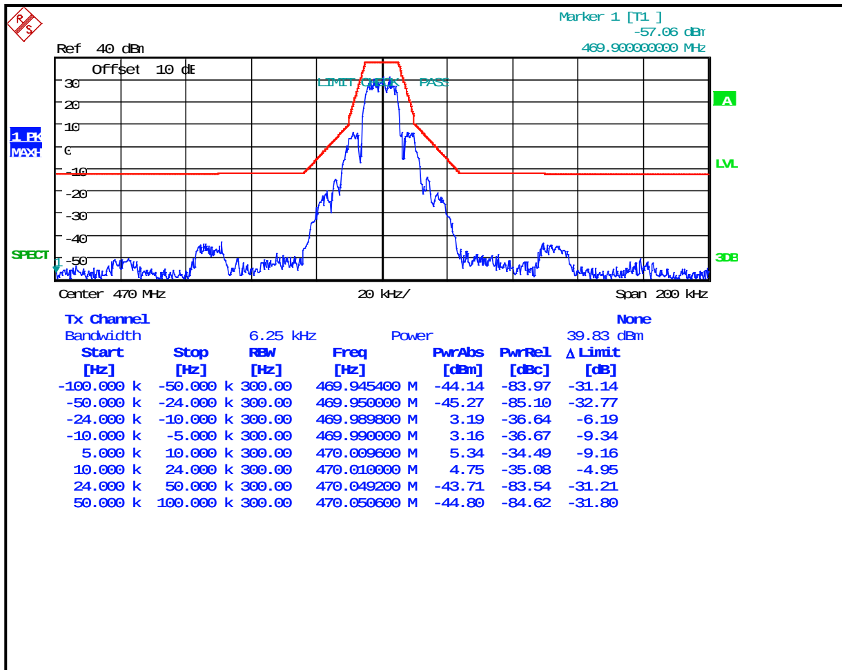
Plot 7-42: Occupied Bandwidth – 470 MHz; (2-level FSK 9600; WB) EDACS; Mask C
