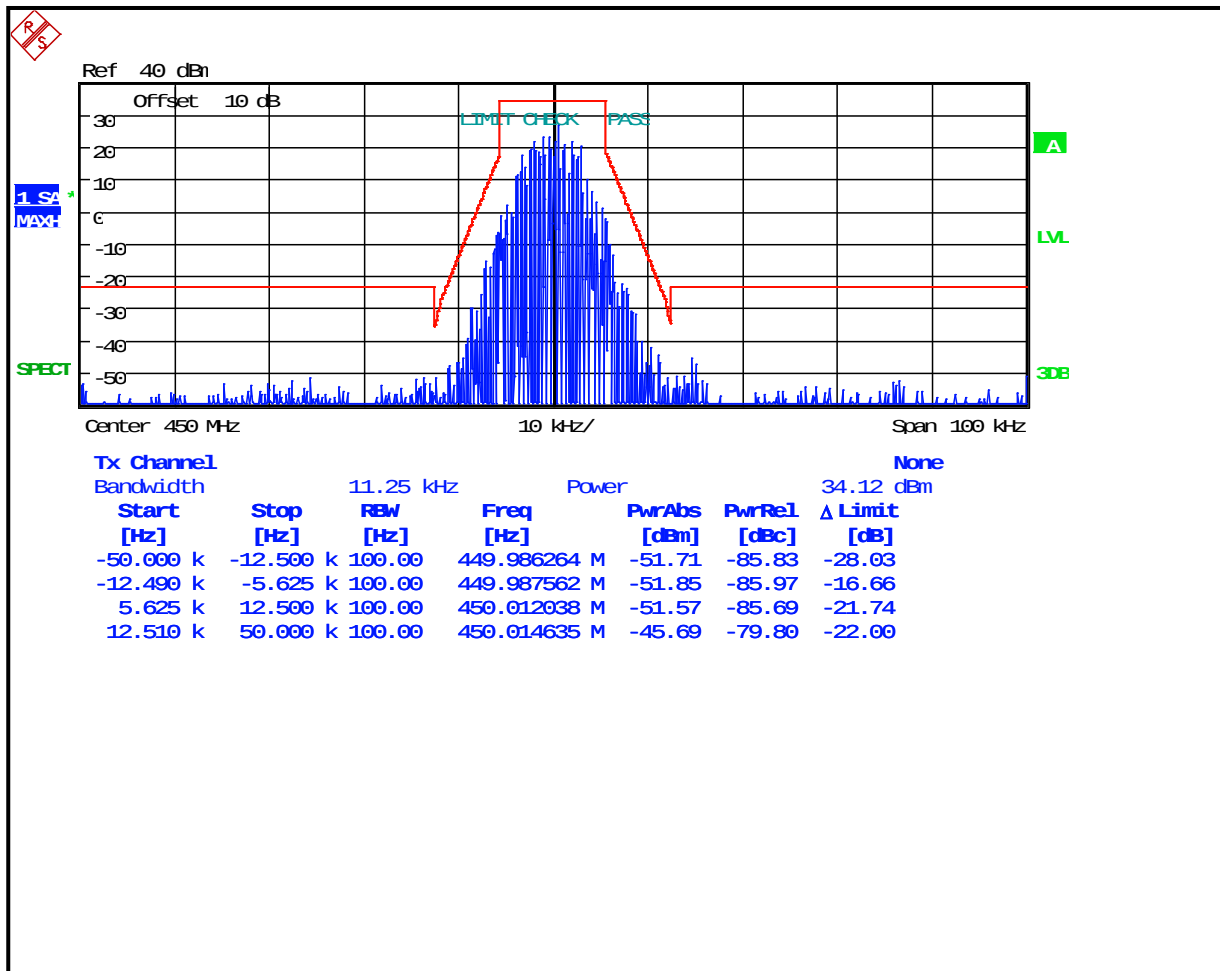
Plot 7-23: Occupied Bandwidth – 450 MHz; CPM TDMA; Mask D
