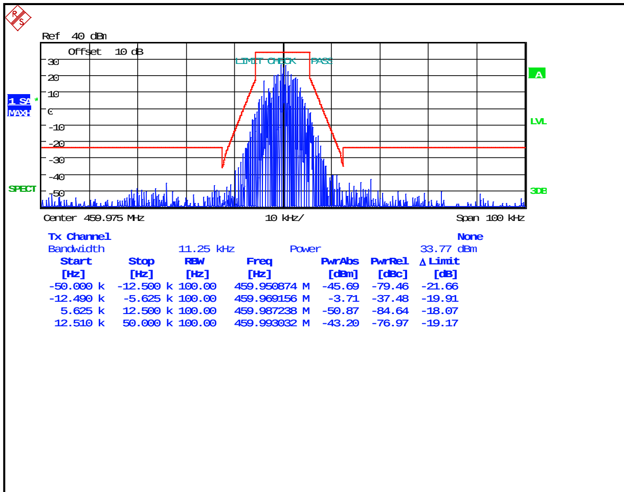
Plot 7-27: Occupied Bandwidth – 459.975 MHz; CPM TDMA; Mask D
