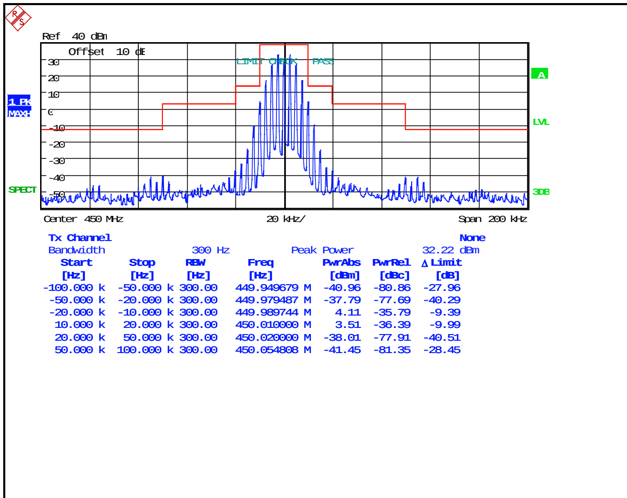
Plot 7-2: Occupied Bandwidth – 450 MHz; Wideband Analog; Mask B
