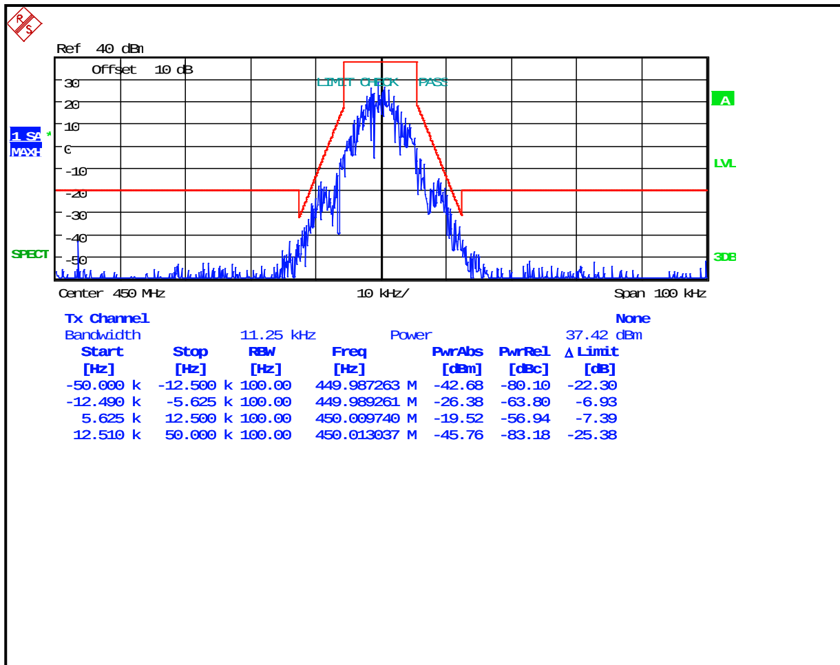
Plot 7-30: Occupied Bandwidth – 450 MHz; (2-level FSK 9600; NB) EDACS; Mask D
