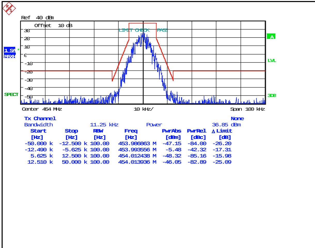
Plot 7-45: Occupied Bandwidth – 454 MHz; (4-level FSK Data/Voice; NB) OpenSky; Mask D
