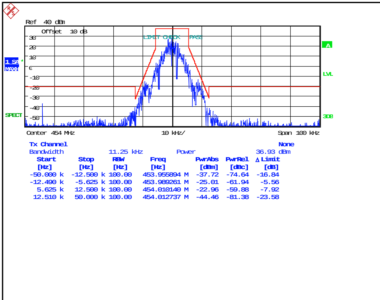
Plot 7-31: Occupied Bandwidth – 454 MHz; (2-level FSK 9600; NB) EDACS; Mask D
