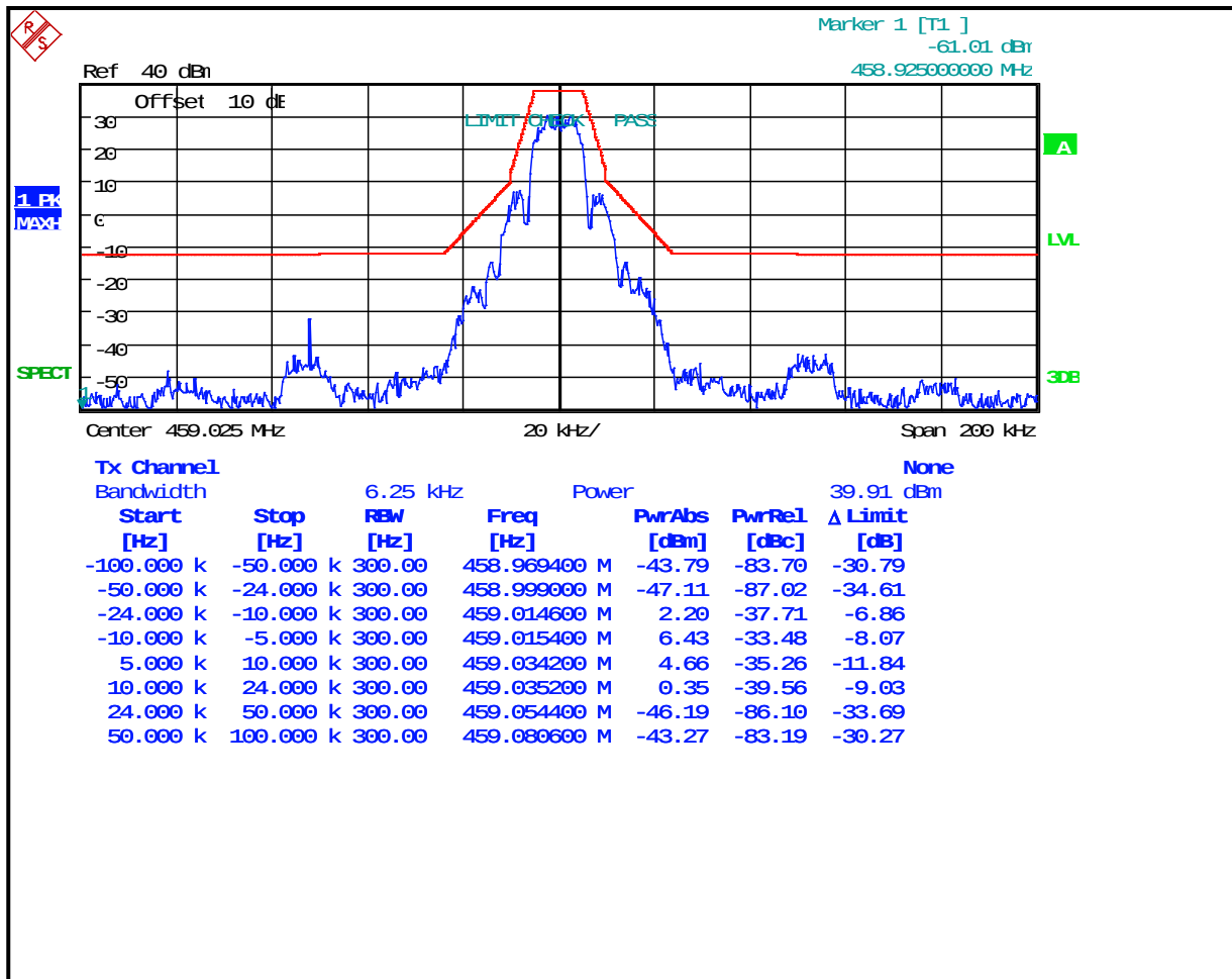
Plot 7-40: Occupied Bandwidth – 459.025 MHz; (2-level FSK 9600; WB) EDACS; Mask C
