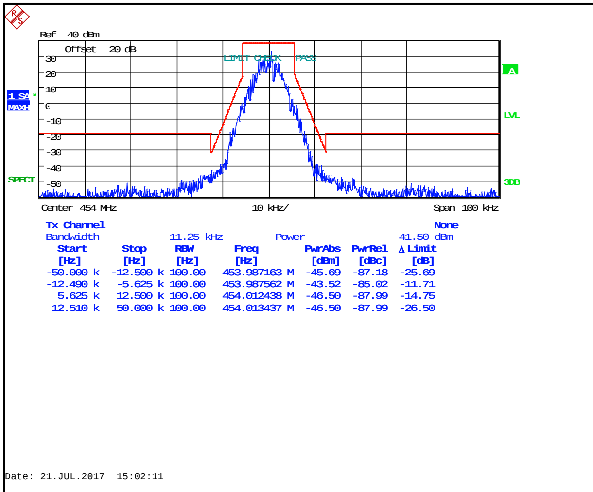
Plot 7-17: Occupied Bandwidth – 454 MHz; P25; Mask D
