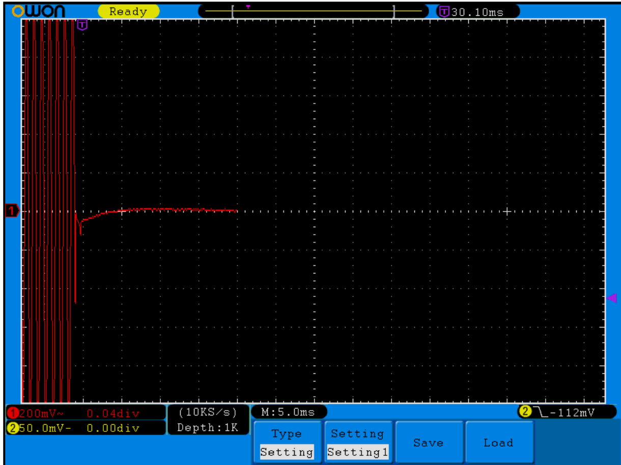
Plot 10-1: Transient Frequency Behavior – 430 MHz; High Power; Narrowband; Carrier ON Time
