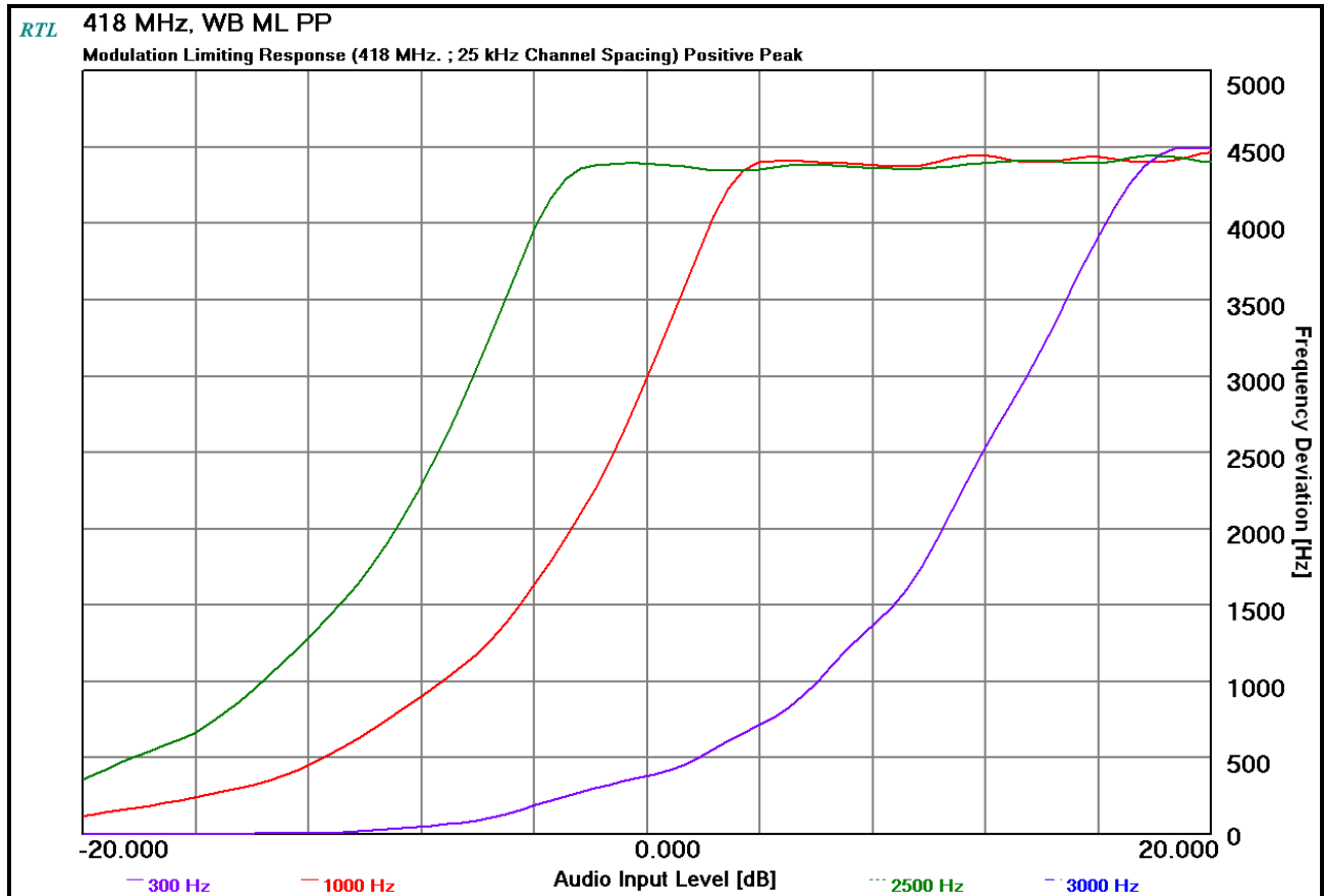
Plot 9-10: Modulation Characteristics – Modulation Limiting - 418 MHz; Positive Peak; WB
