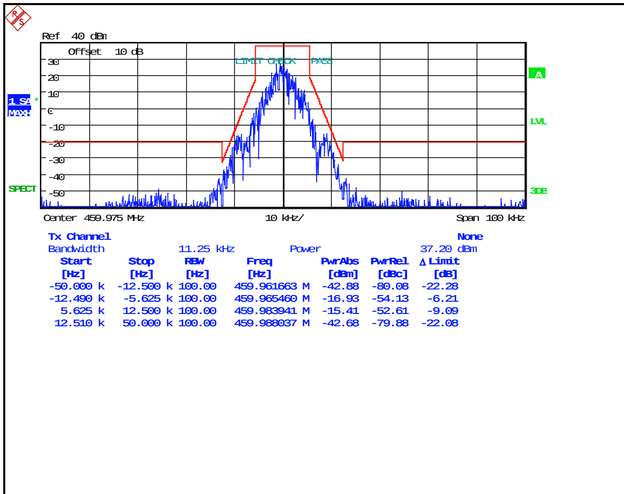
Plot 7-34: Occupied Bandwidth – 459.975 MHz; (2-level FSK 9600; NB) EDACS; Mask D
