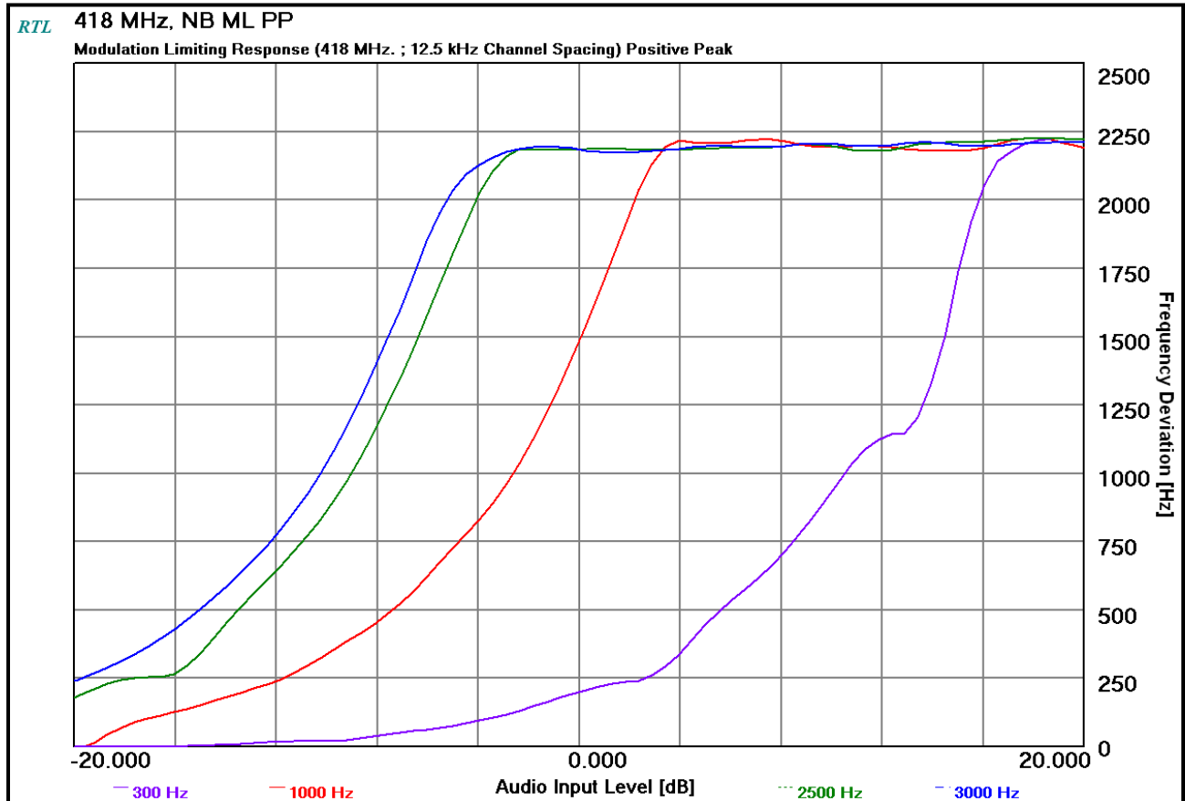
Plot 9-8: Modulation Characteristics – Modulation Limiting - 418 MHz; Positive Peak; NB
