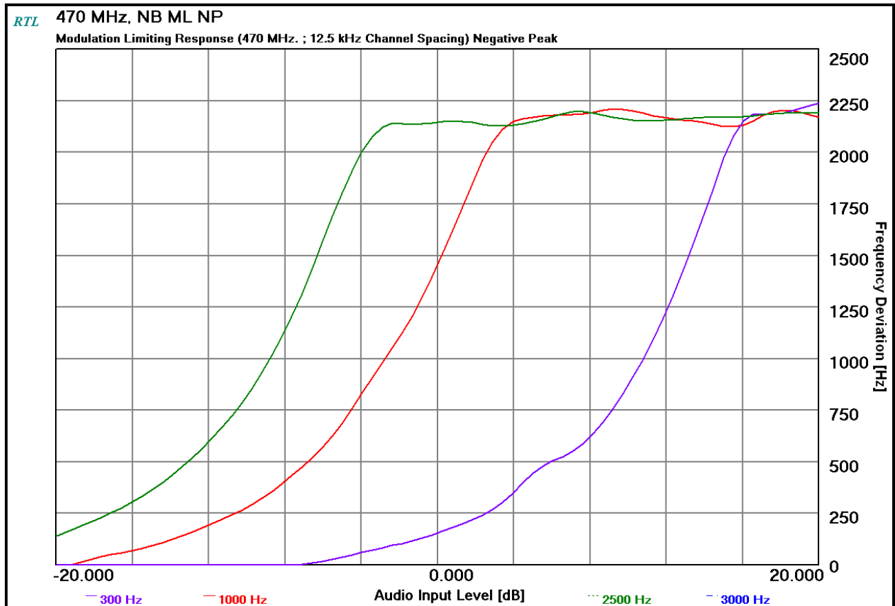
Plot 9-13: Modulation Characteristics – Modulation Limiting - 470 MHz; Negative Peak; NB
