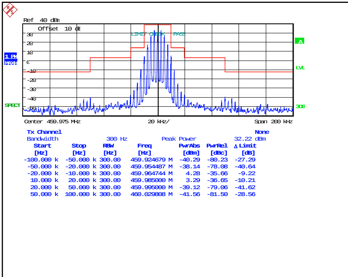
Plot 7-6: Occupied Bandwidth – 459.975MHz; Wideband Analog; Mask B
