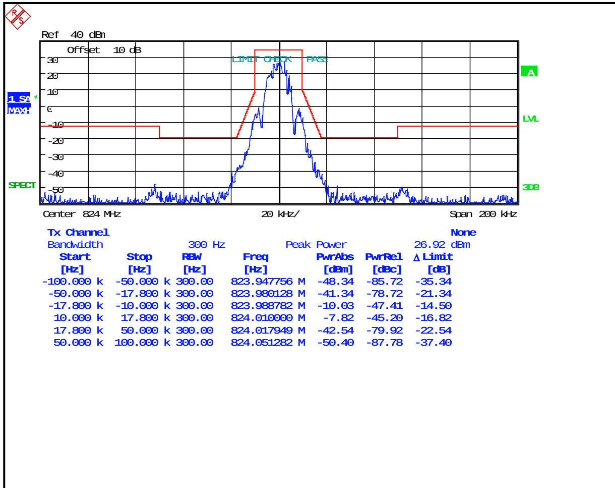
Plot 8-45: Occupied Bandwidth – 824 MHz; 4-level FSK Data/Voice; NB NPSPAC EDACS; Mask G
