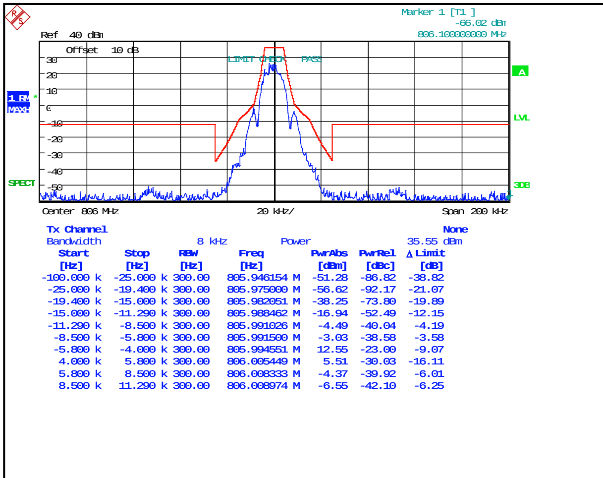
Plot 8-43: Occupied Bandwidth – 806 MHz; 4-level FSK Data/Voice; NB NPSPAC EDACS; Mask H
