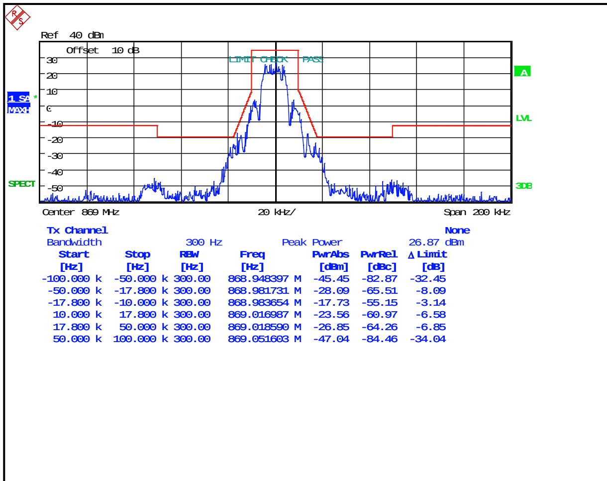
Plot 8-42: Occupied Bandwidth – 869 MHz; 2-level FSK 9600; WB EDACS; Mask G
