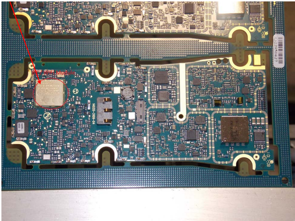
Main Board Bottom without Shields
