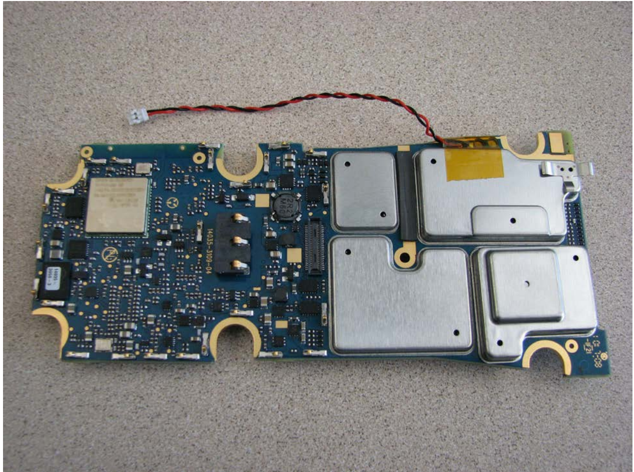
Main Board Bottom with Shields
