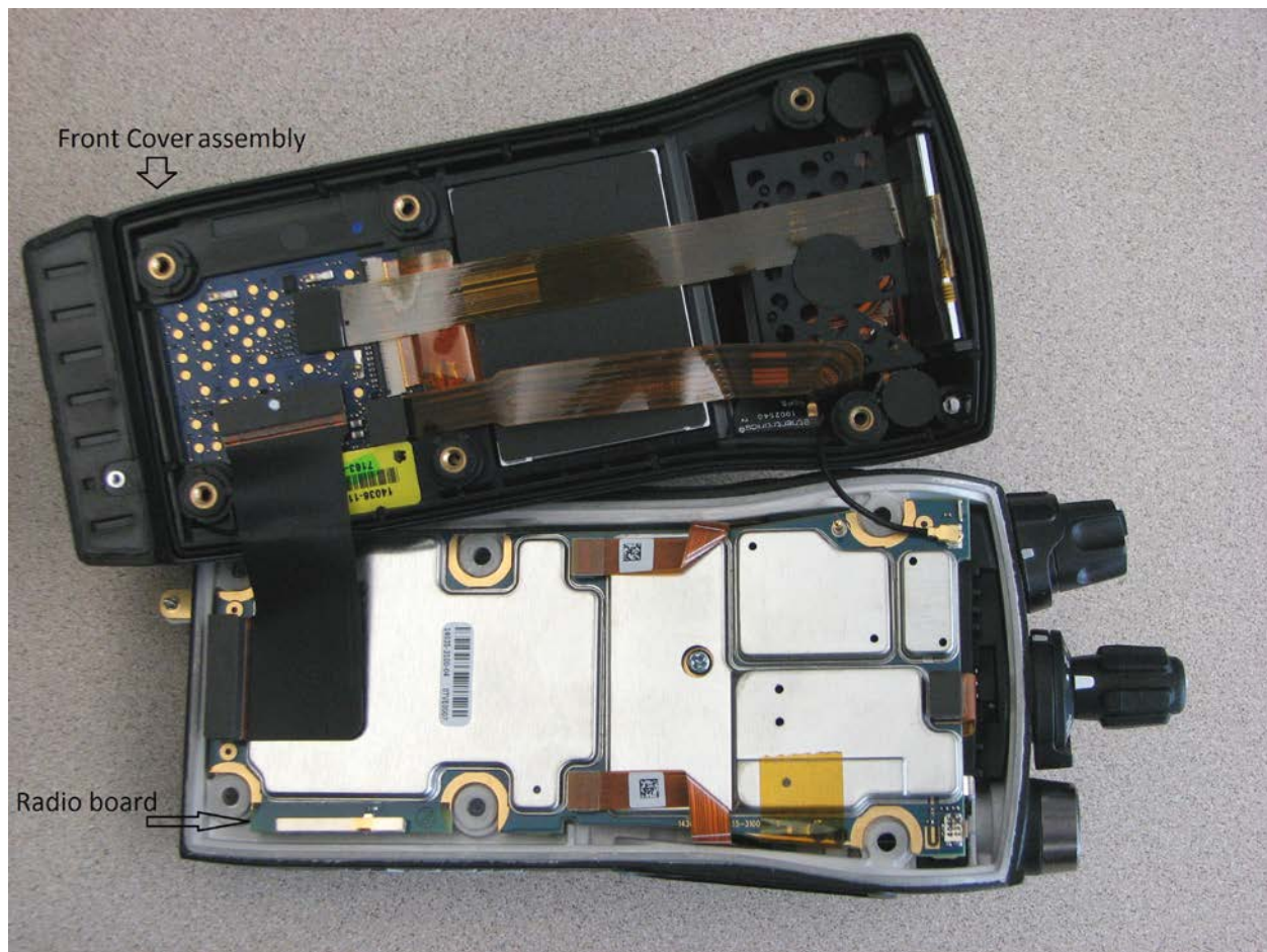
Main Board in Chassis
