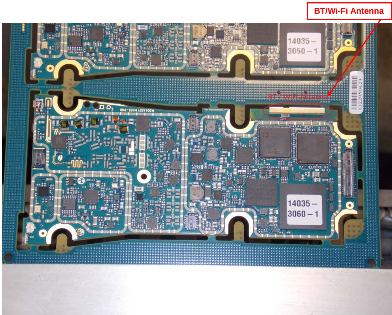
Main Board Top without Shields
