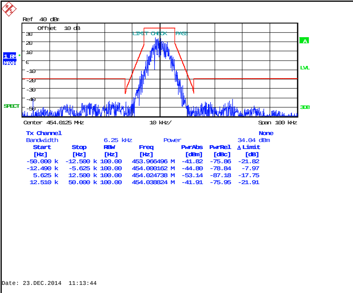
Plot 7-78: Occupied Bandwidth – 454.0125 MHz; C4FM Phase 2 (Mask D)
