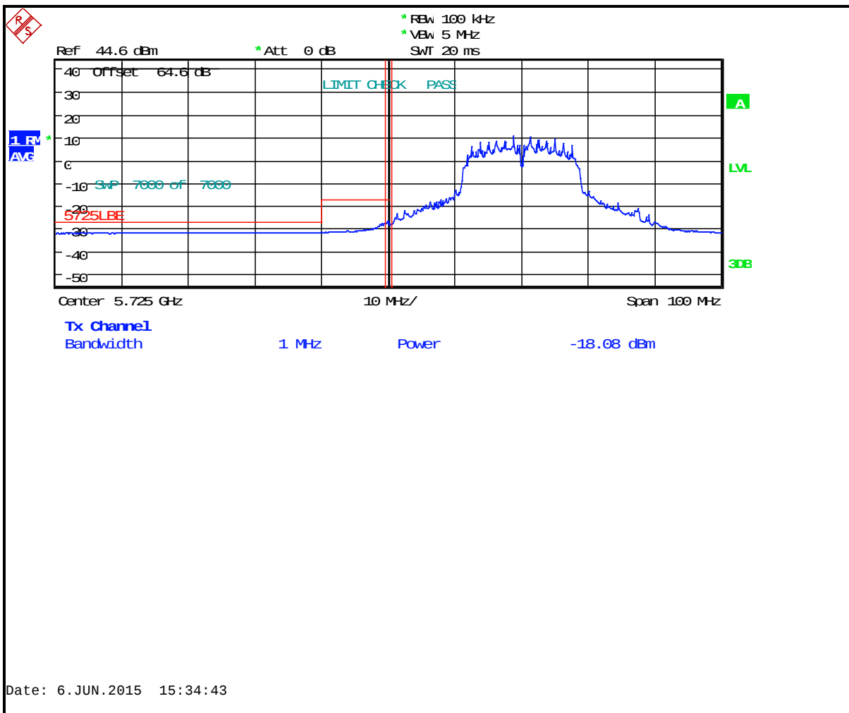
Plot 6-12: Lower Band Edge: Measurement Channel 149 (5745 MHz, 802.11n, Average)
