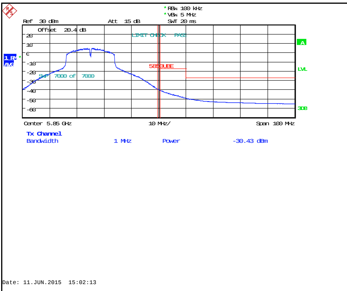
Plot 6-20: Upper Band Edge: Measurement Channel 165 (5825 MHz, 802.11n, Average)
