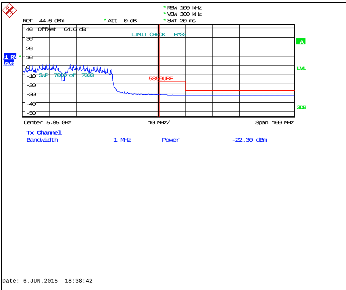
Plot 6-22: Upper Band Edge: Measurement Channel 165 (5825 MHz, 40 MHz BW, 802.11a, Average)
