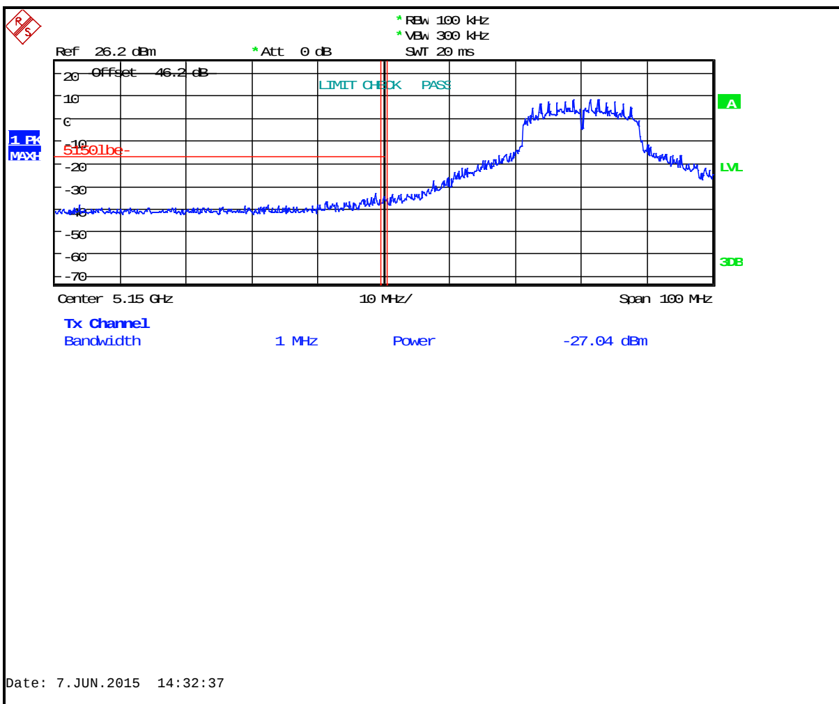
Plot 6-3: Lower Band Edge: Measurement Channel 36 (5180 MHz, 802.11n, Peak)
