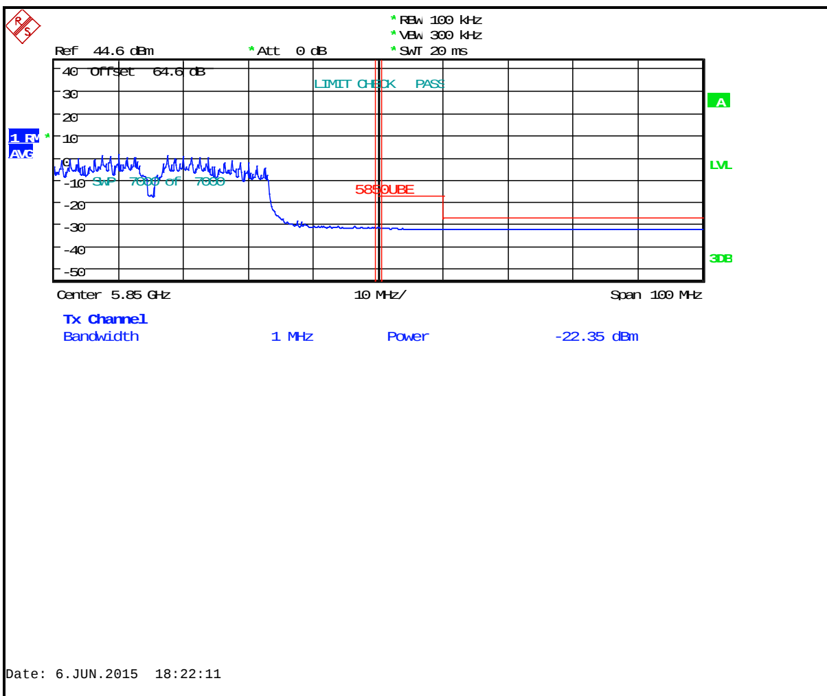
Plot 6-24: Upper Band Edge: Measurement Channel 165 (5825 MHz, 40 MHz BW, 802.11n, Average)
