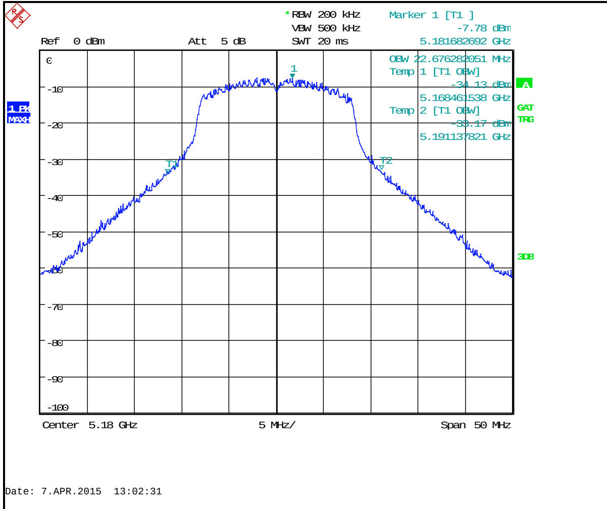
Plot 8-8: 26 dB Bandwidth Channel 36 (TX Frequency 5180 MHz) - 802.11n
