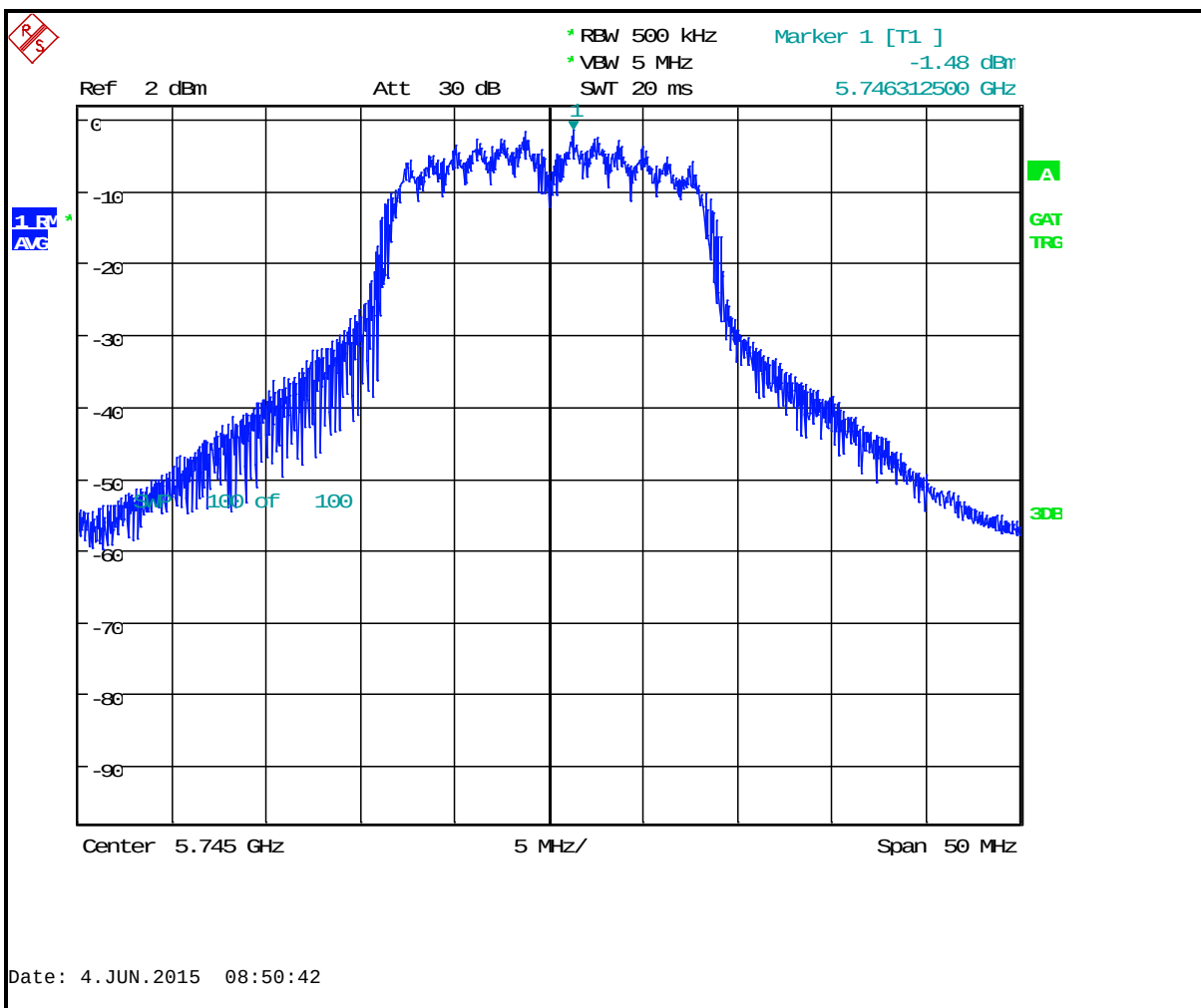
Plot 4-12: Power Spectral Density: Channel 149 (5745 MHz) 802.11n 65 Mbps
