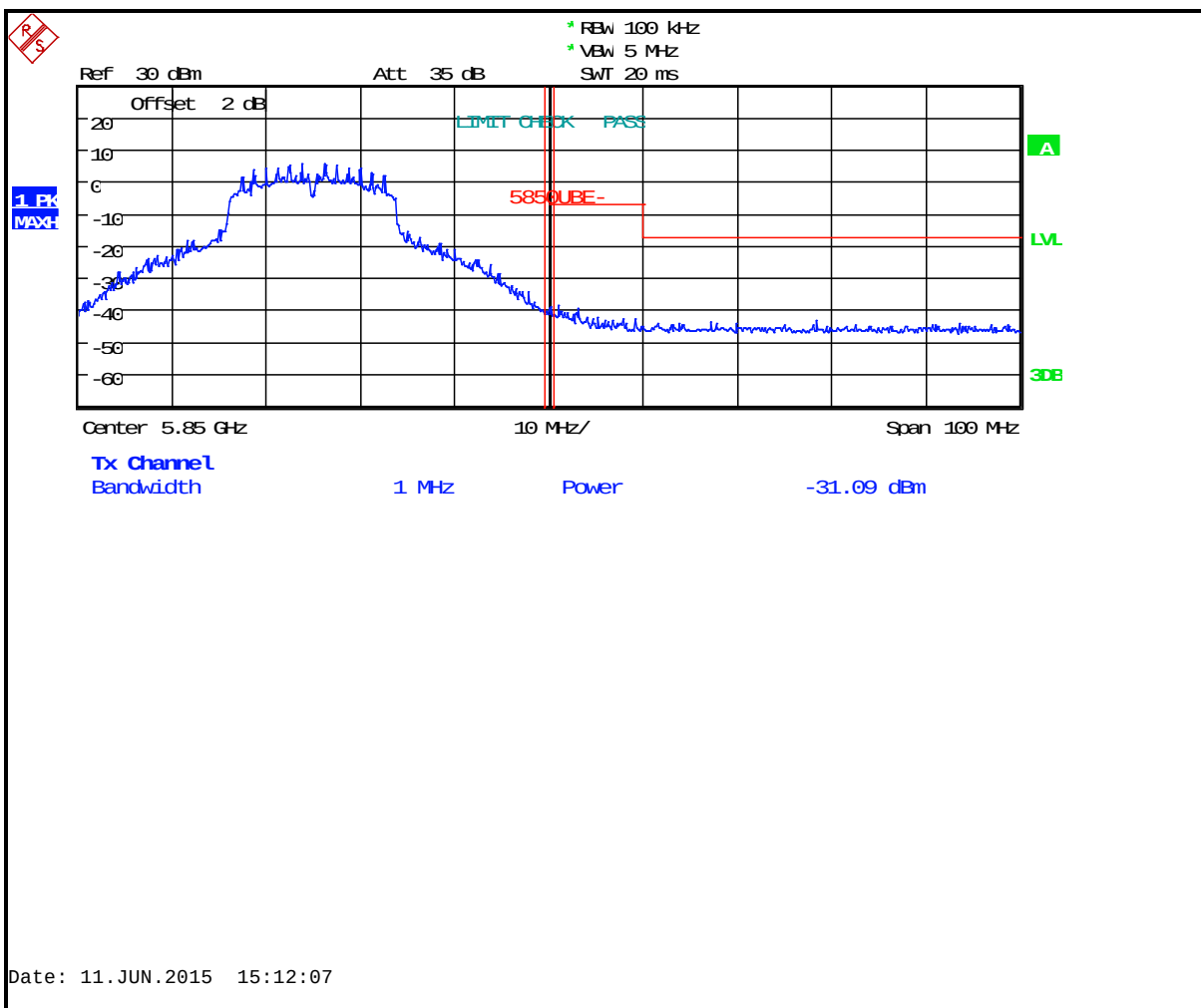
Plot 6-19: Upper Band Edge: Measurement Channel 165 (5825 MHz, 802.11n, Peak)
