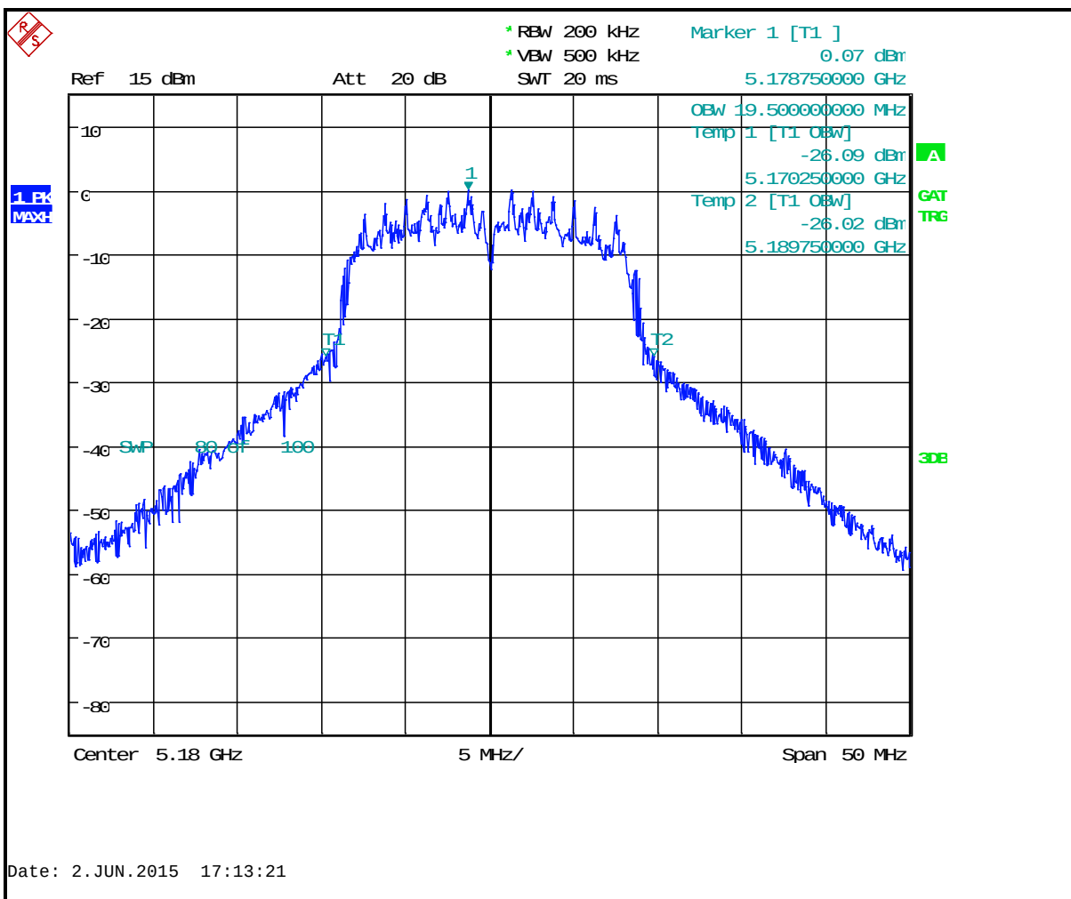
Plot 8-1: 26 dB Bandwidth Channel 36 (TX Frequency 5180 MHz) - 802.11a
