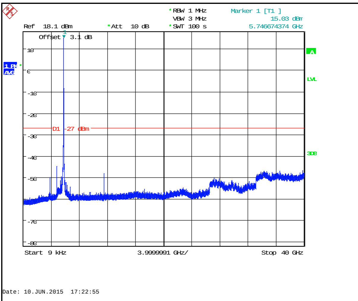
Plot 7-7: Undesirable Emissions Channel 149 (5745 MHz)
