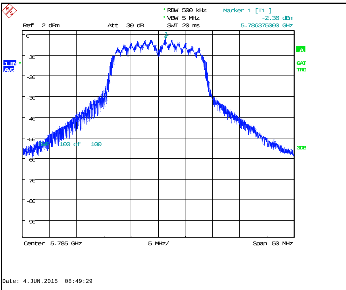
Plot 4-13: Power Spectral Density: Channel 157 (5785 MHz) 802.11n 65 Mbps
