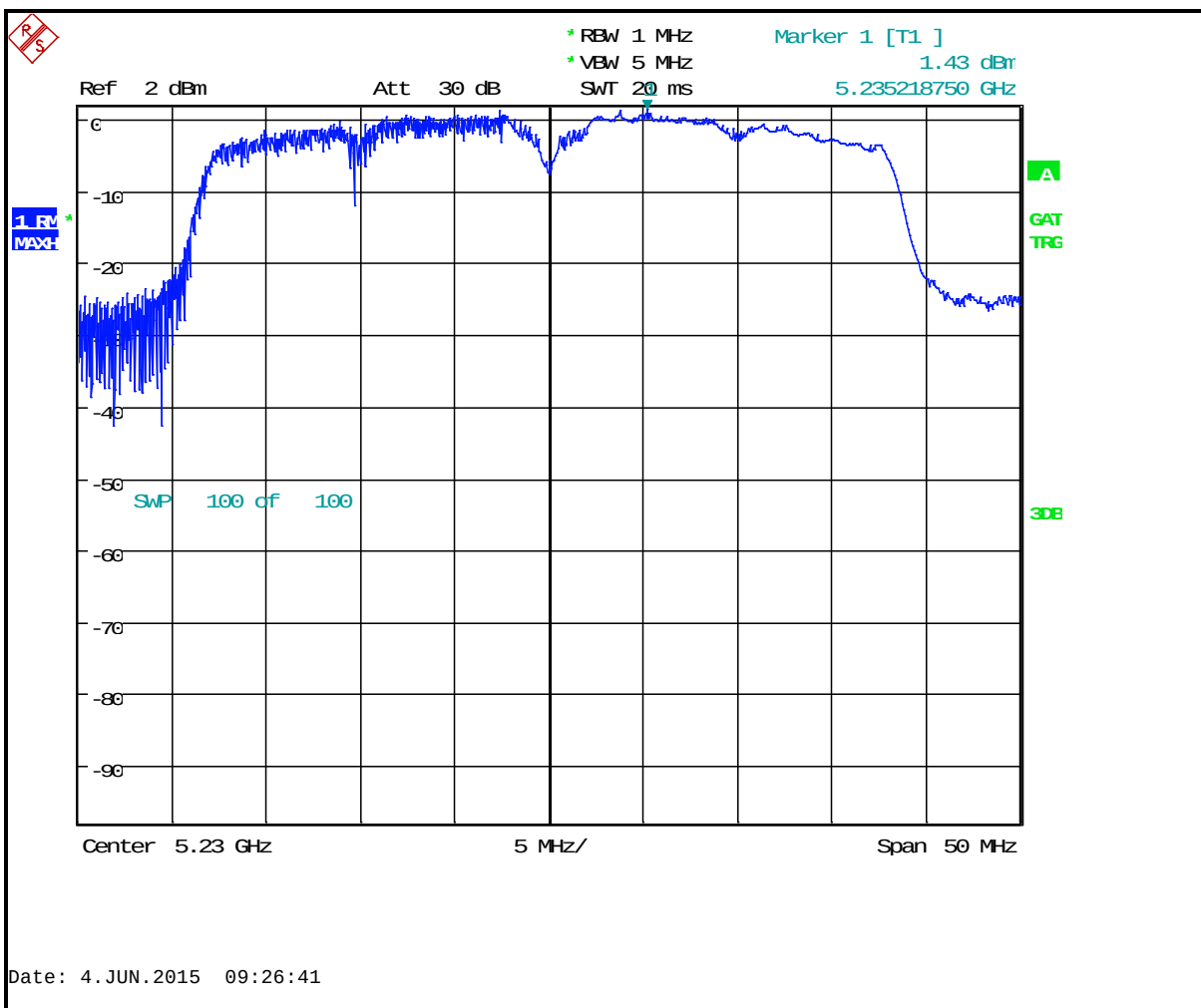
Plot 4-17: Peak Power Spectral Density: Channel 44 (5220 MHz, lower) 802.11n 40 MHz
