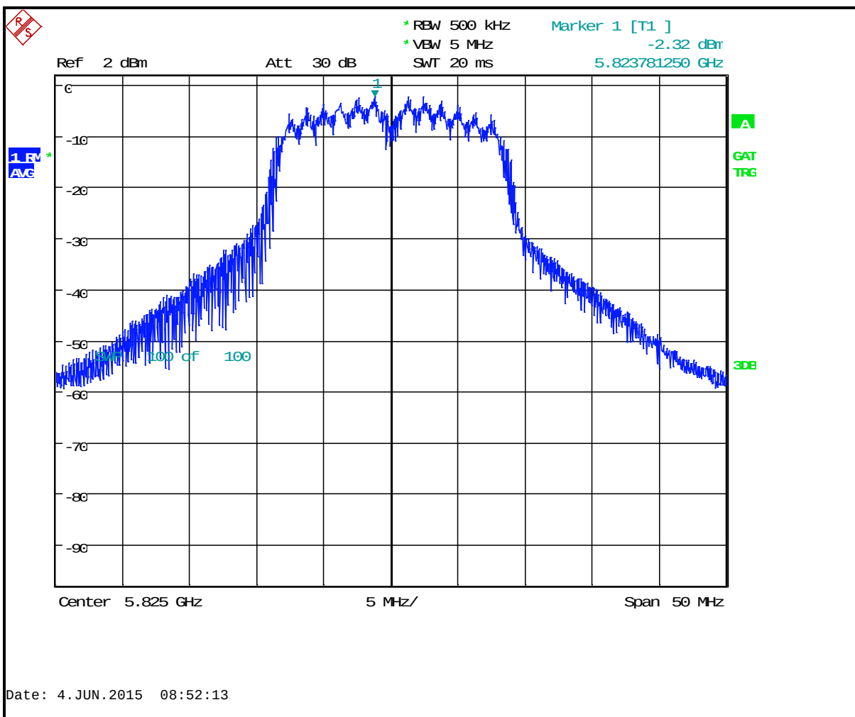
Plot 4-14: Power Spectral Density: Channel 165 (5825 MHz) 802.11n 65 Mbps
