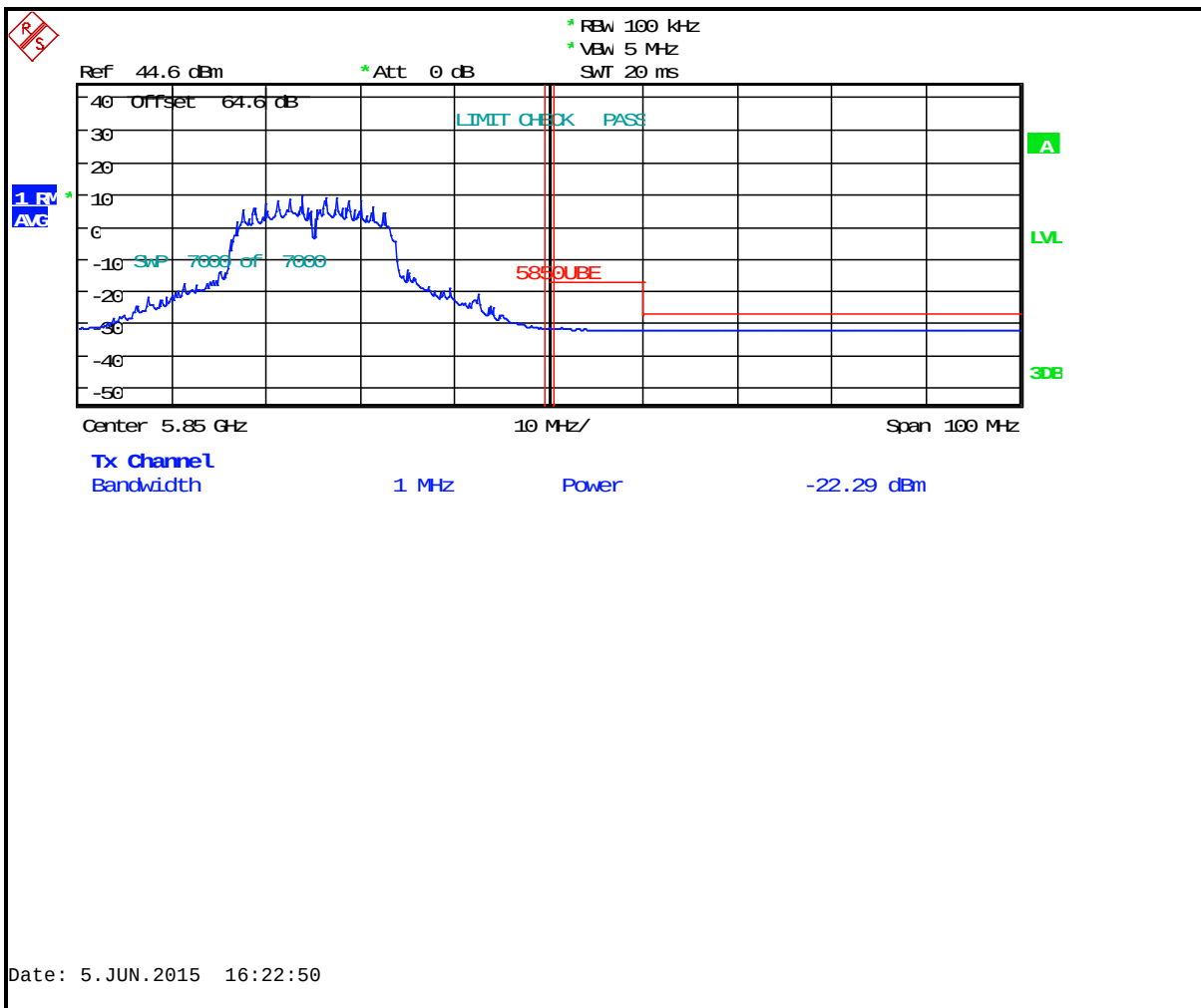
Plot 6-18: Upper Band Edge: Measurement Channel 165 (5825 MHz, 802.11a, Average)
