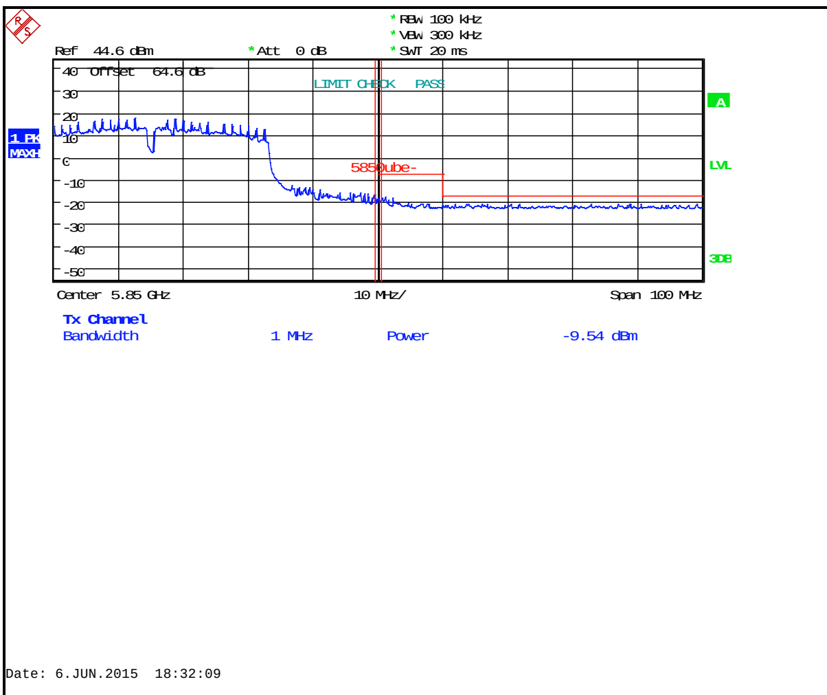
Plot 6-21: Upper Band Edge: Measurement Channel 165 (5825 MHz, 40 MHz BW, 802.11a, Peak)
