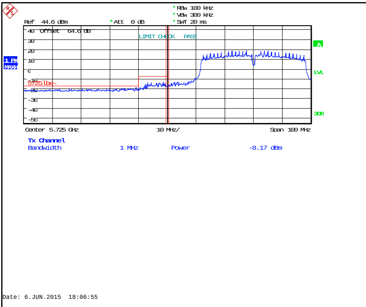
Plot 6-15: Lower Band Edge: Measurement Channel 149 (5745 MHz, 40 MHz BW, 802.11n, Peak)
