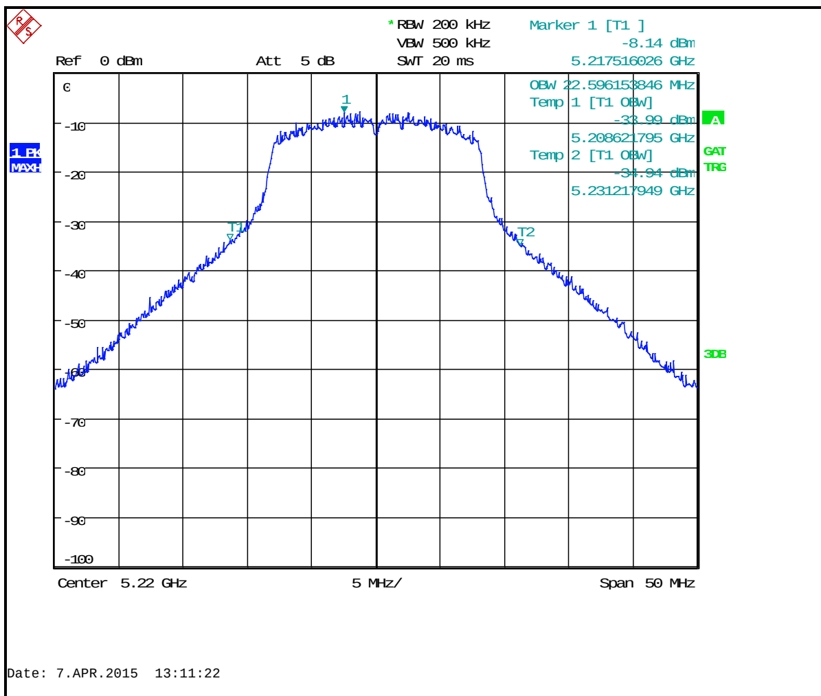
Plot 8-10: 26 dB Bandwidth Channel 44 (TX Frequency 5220 MHz) - 802.11n
