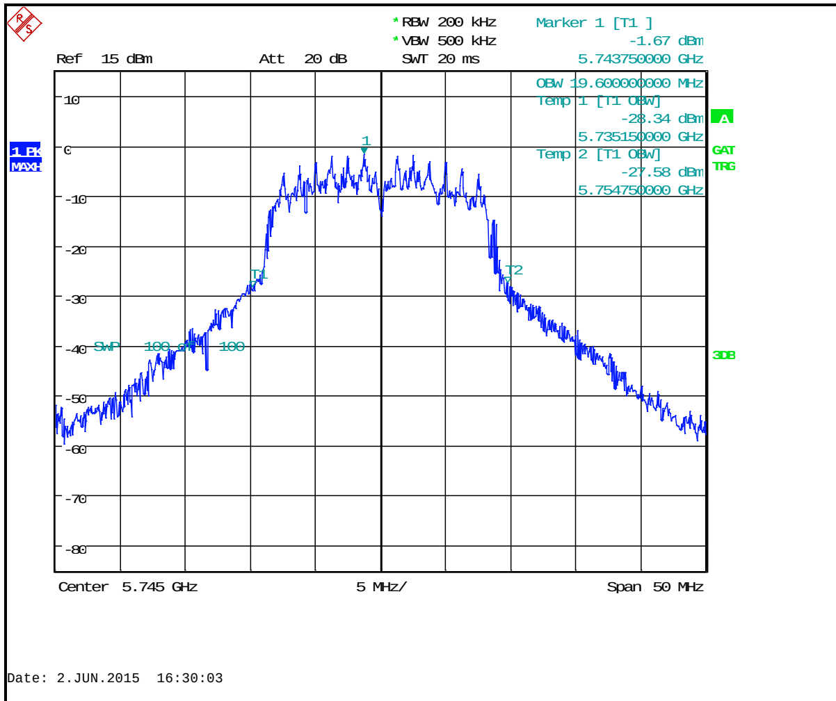
Plot 8-5: 26 dB Bandwidth Channel 149 (TX Frequency 5745 MHz) - 802.11a
