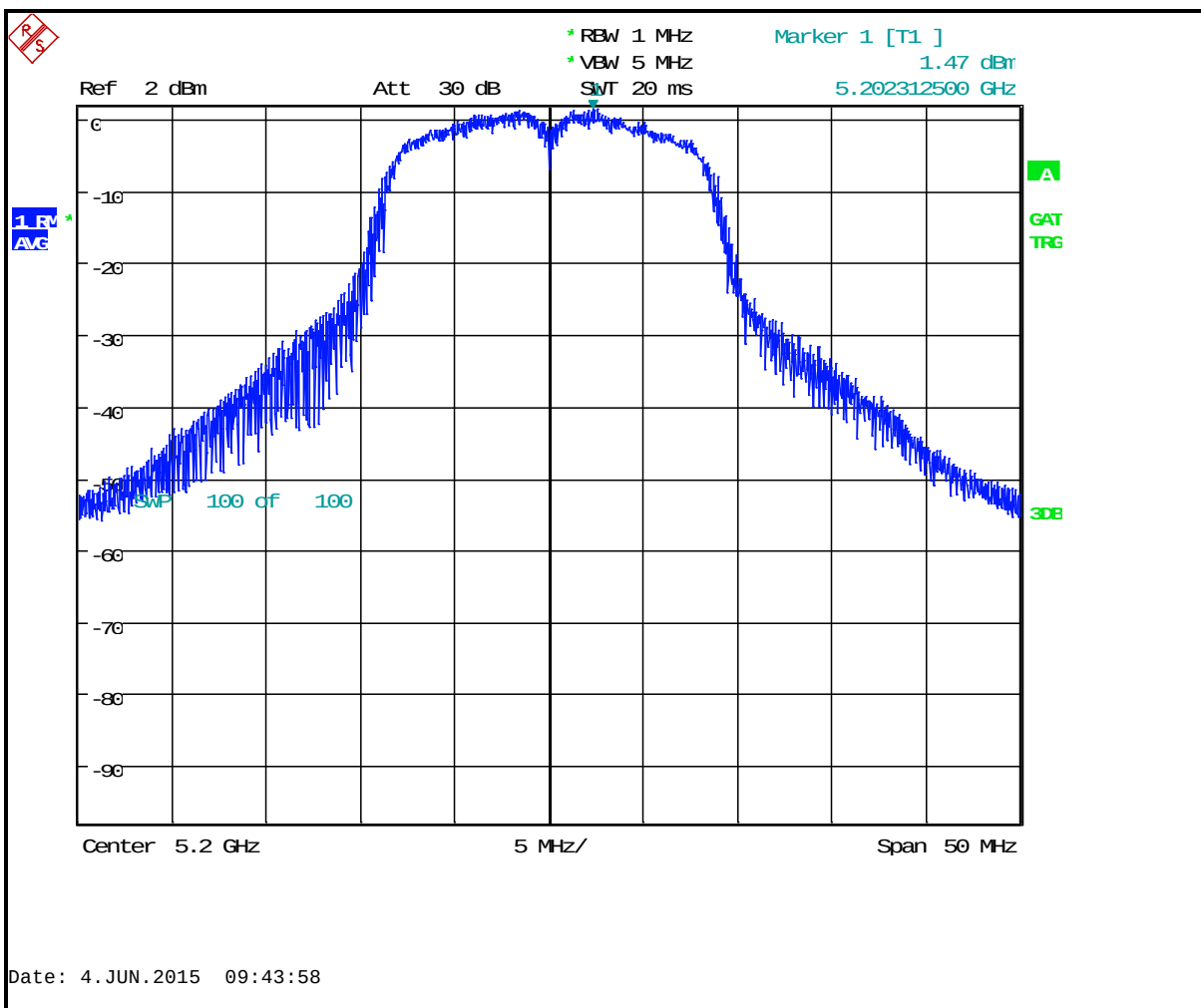
Plot 4-9: Peak Power Spectral Density: Channel 40 (5200 MHz) 802.11n 65 Mbps
