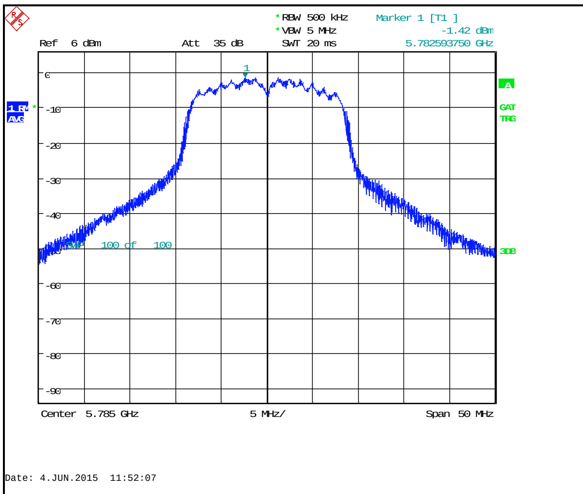
Plot 4-6: Power Spectral Density: Channel 157 (5785 MHz) 802.11a 54 Mbps
