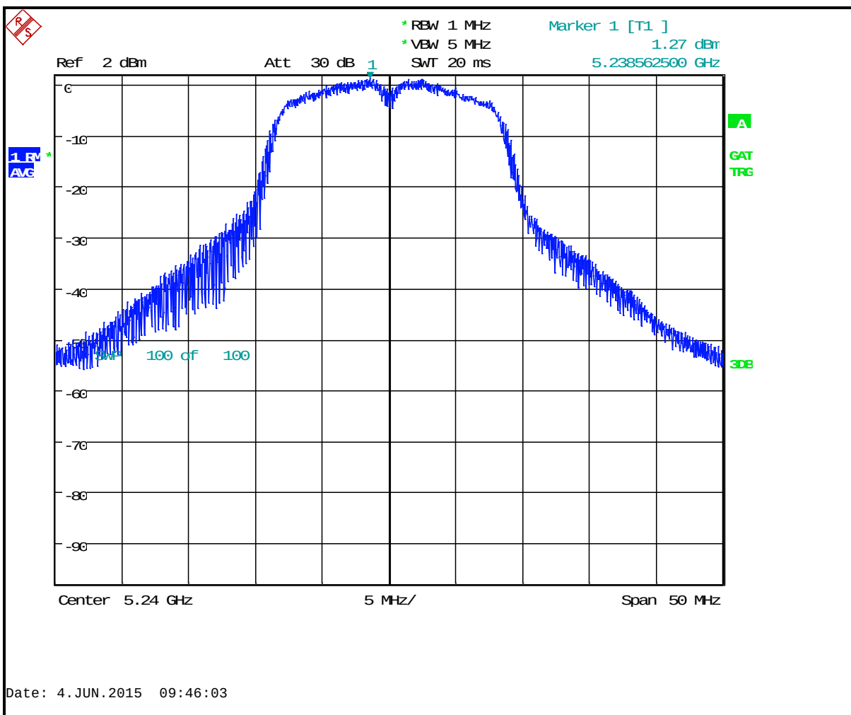
Plot 4-11: Peak Power Spectral Density: Channel 48 (5240 MHz) 802.11n 65 Mbps
