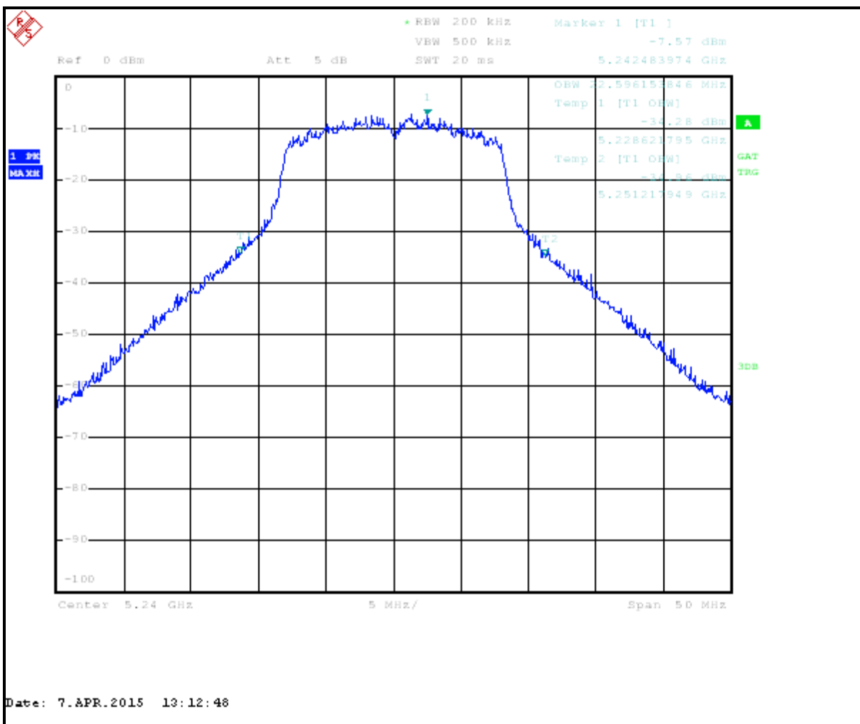
Plot 8-11: 26 dB Bandwidth Channel 48 (TX Frequency 5240 MHz) - 802.11n
