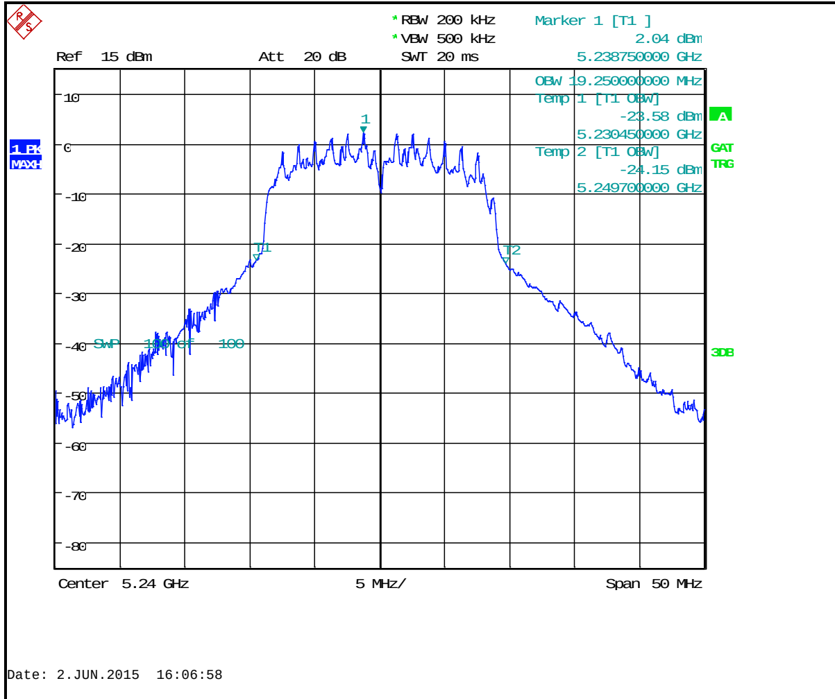
Plot 8-4: 26 dB Bandwidth Channel 48 (TX Frequency 5240 MHz) - 802.11a
