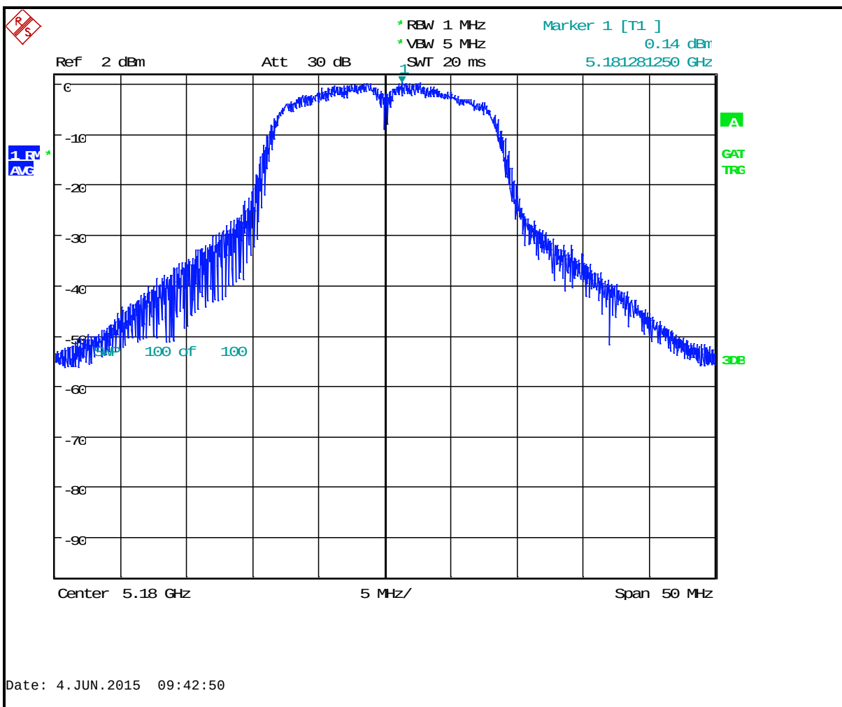
Plot 4-8: Peak Power Spectral Density: Channel 36 (5180 MHz) 802.11n 65 Mbps
