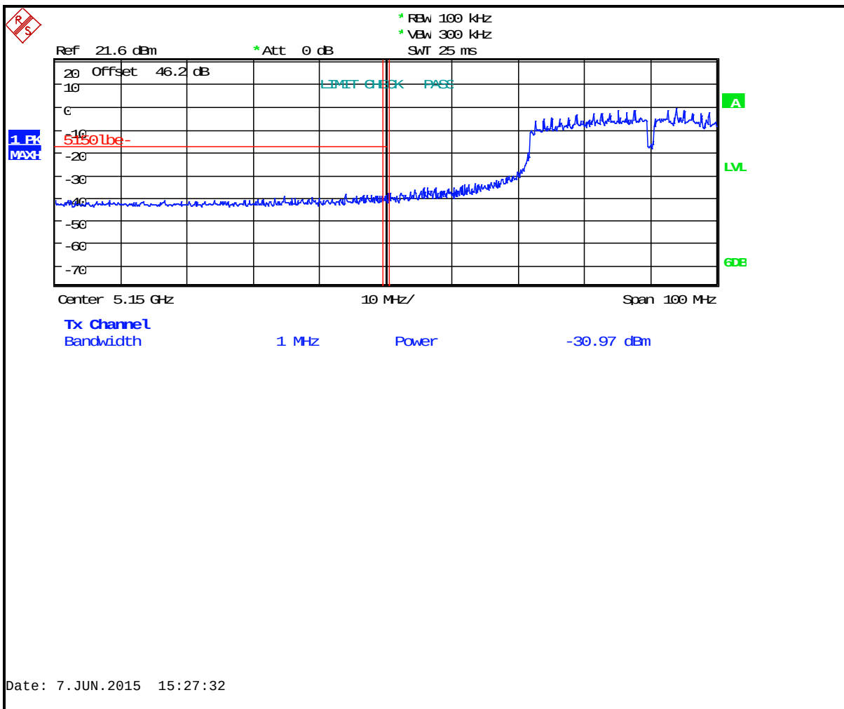
Plot 6-5: Lower Band Edge: Measurement Channel 36 (5180 MHz, 40 MHz BW, 802.11a, Peak)
