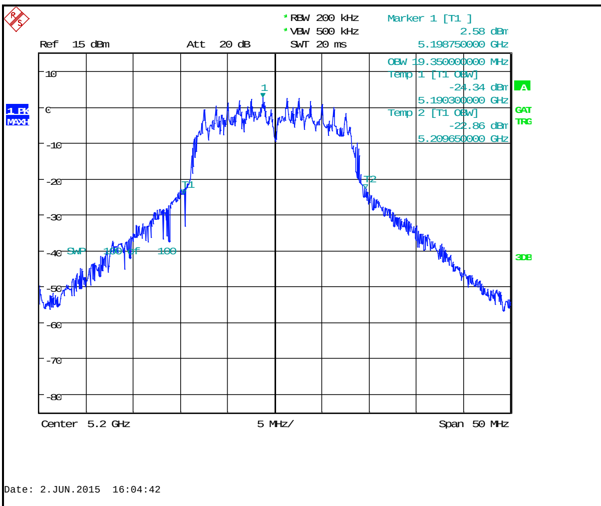
Plot 8-2: 26 dB Bandwidth Channel 40 (TX Frequency 5200 MHz) - 802.11a
