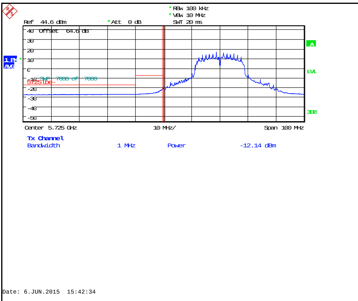
Plot 6-11: Lower Band Edge: Measurement Channel 149 (5745 MHz, 802.11n, Peak)
