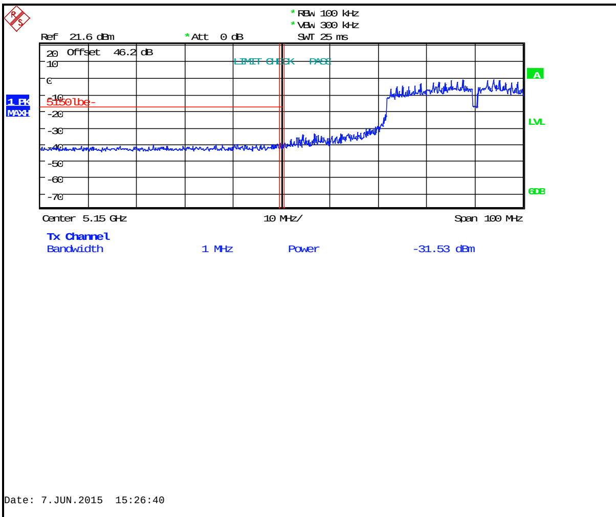
Plot 6-7: Lower Band Edge: Measurement Channel 36 (5180 MHz, 40 MHz BW, 802.11n, Peak)
