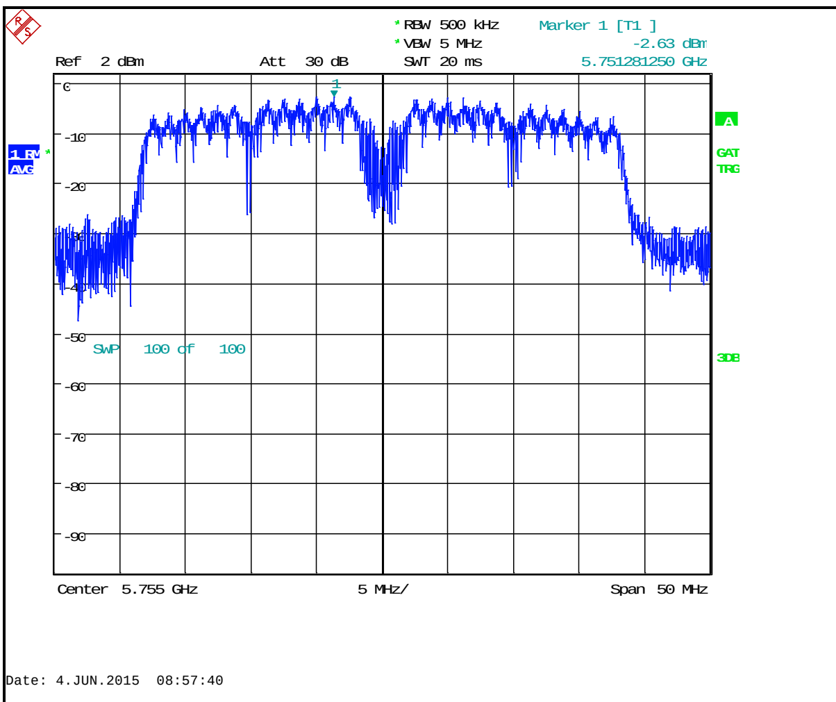
Plot 4-19: Power Spectral Density: Channel 149 (5745 MHz, lower) 802.11n 40 MHz
