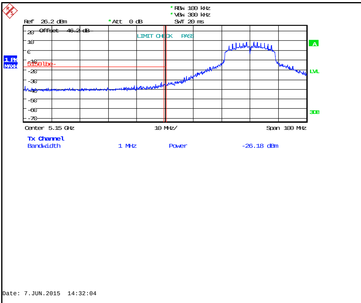
Plot 6-1: Lower Band Edge: Measurement Channel 36 (5180 MHz, 802.11a, Peak)
