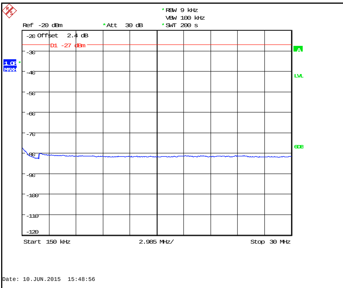
Plot 7-2: Undesirable Emissions Channel 36 (5180 MHz); 150 kHz – 30 MHz
