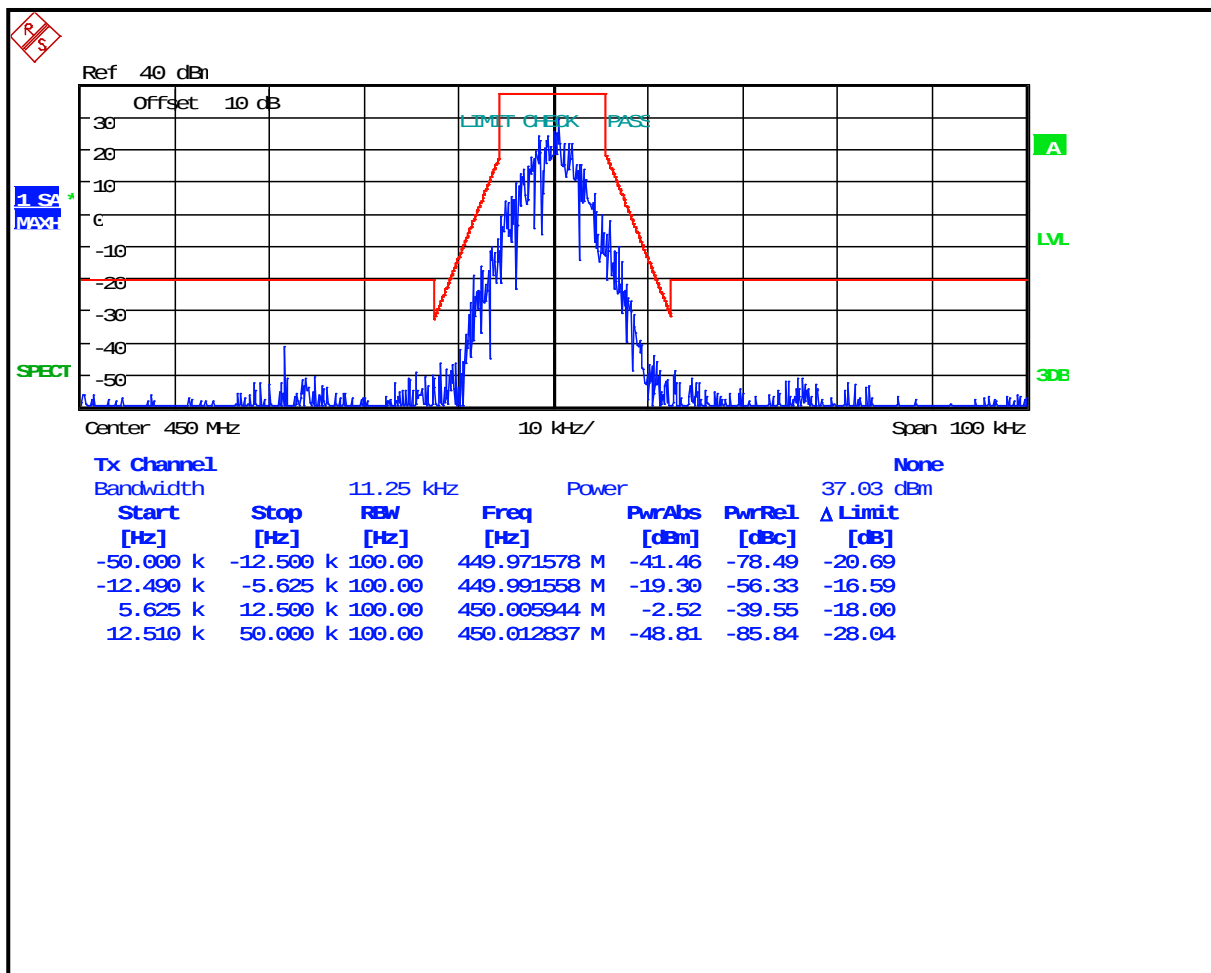
Plot 8-72: Occupied Bandwidth – 450 MHz; (4-level FSK Data/Voice; NB) OpenSky; Mask D
