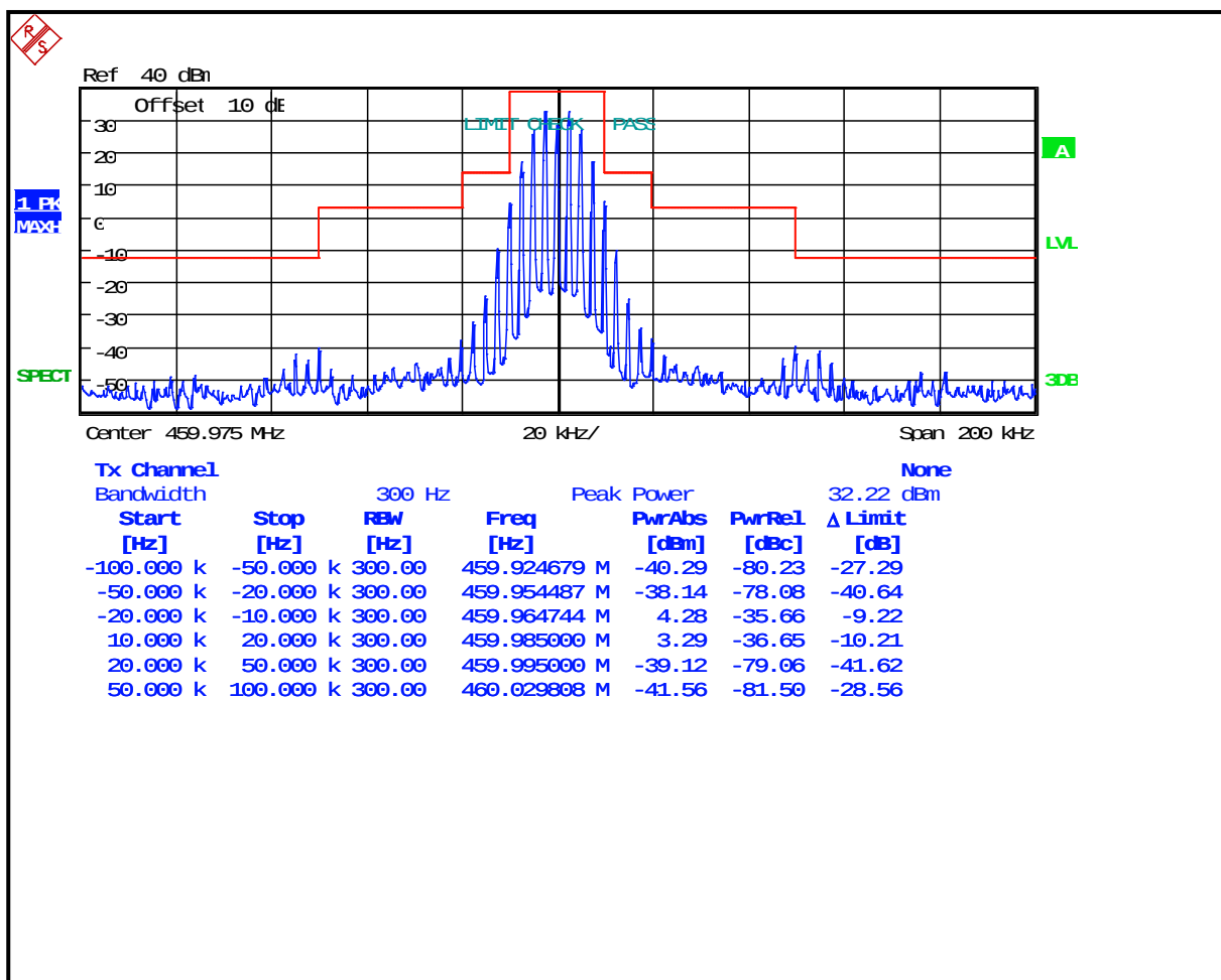
Plot 8-34: Occupied Bandwidth – 459.975MHz; Wideband Analog; Mask B
