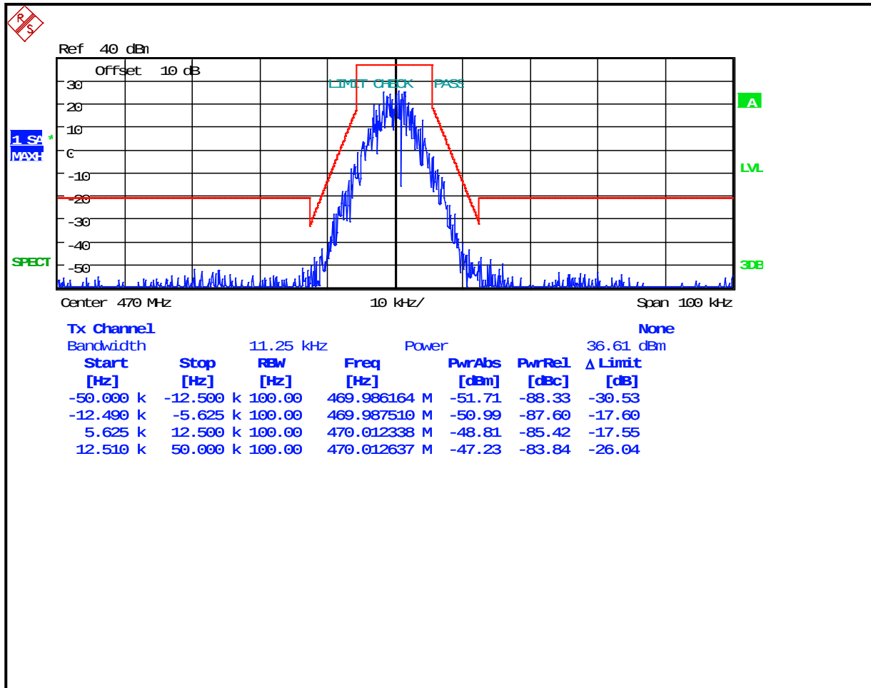
Plot 8-77: Occupied Bandwidth – 470 MHz; (4-level FSK Data/Voice; NB) OpenSky; Mask D
