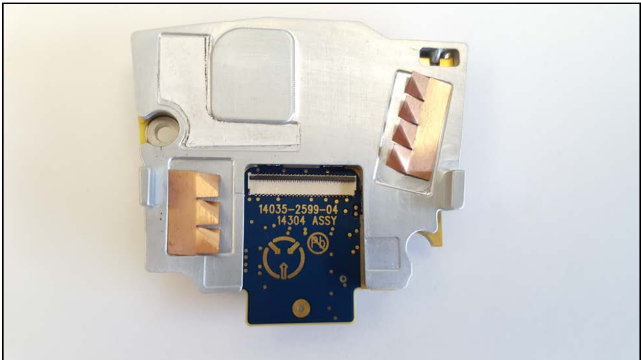
Expansion Board with LTE Module and LTE Processor Shield - Bottom
