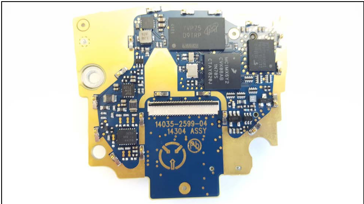
Expansion Board with LTE Module and no LTE Processor Shield – Bottom
