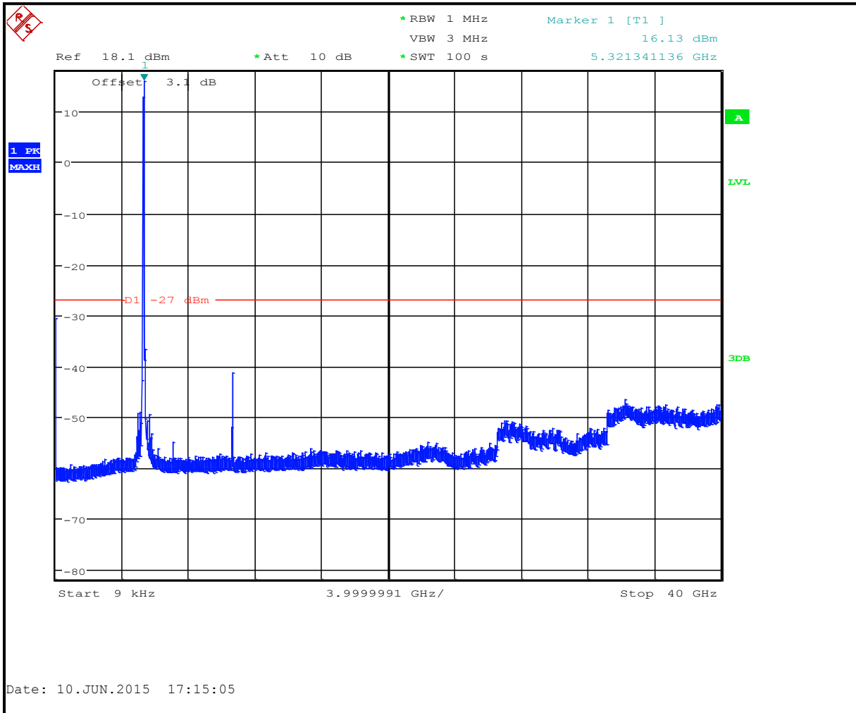
Plot 7-9: Undesirable Emissions Channel 64 (5320 MHz)
