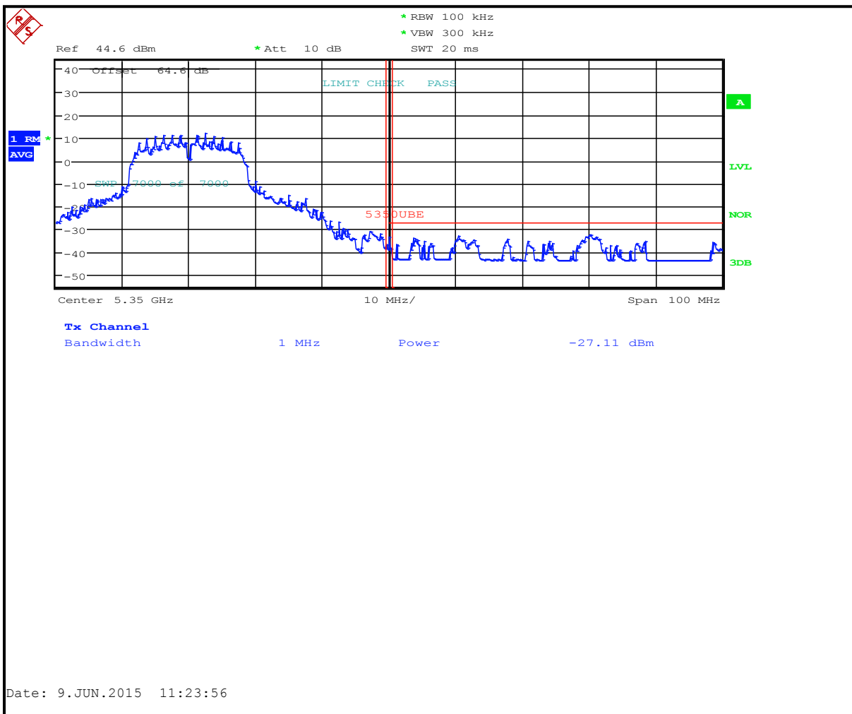
Plot 6-12: Upper Band Edge: Measurement Channel 64 (5320 MHz, 802.11n, Average)
