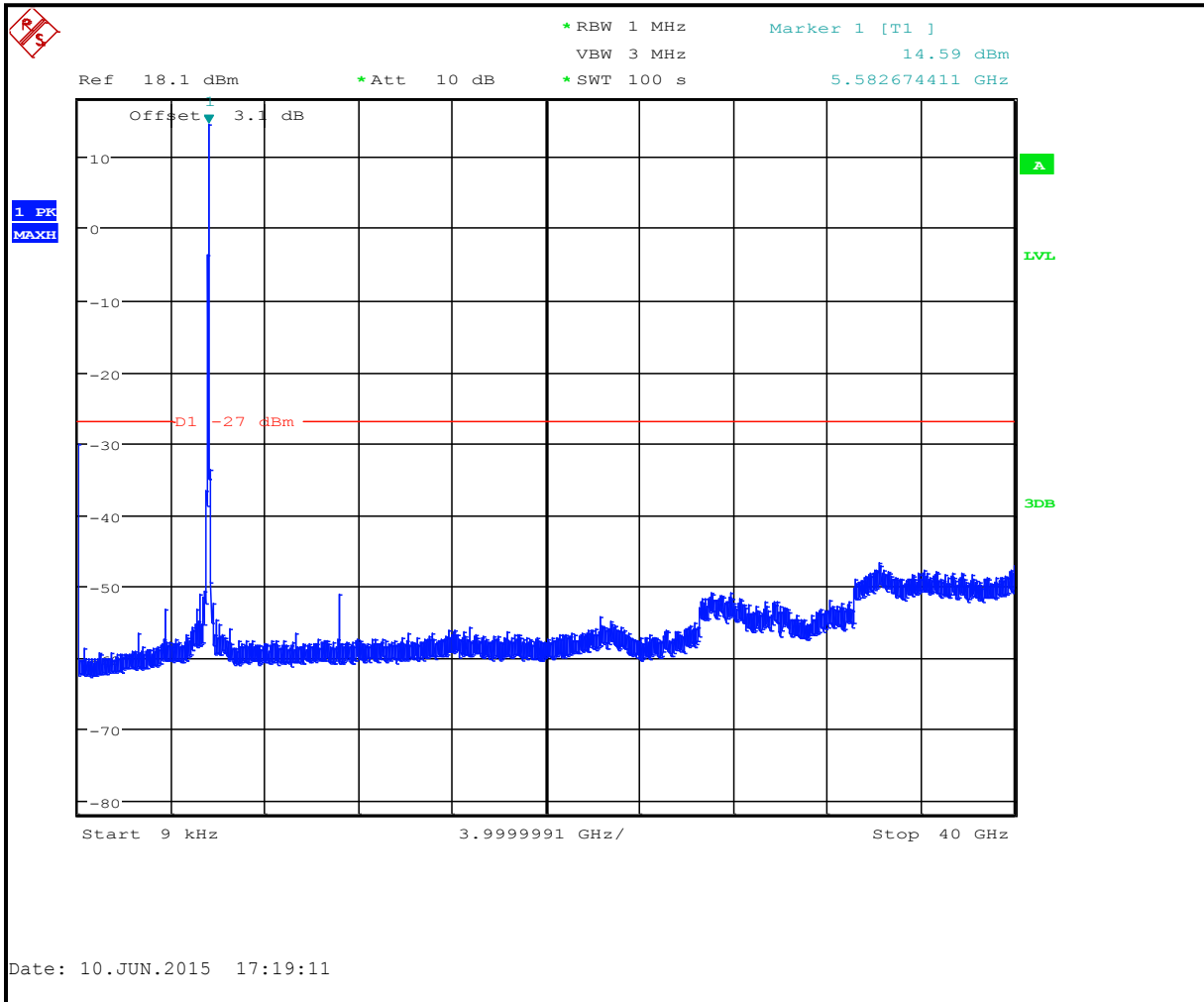
Plot 7-11: Undesirable Emissions Channel 116 (5580 MHz)
