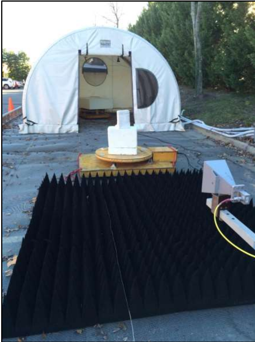
Photograph 6: Radiated Emissions – Back View (above 1 GHz)
